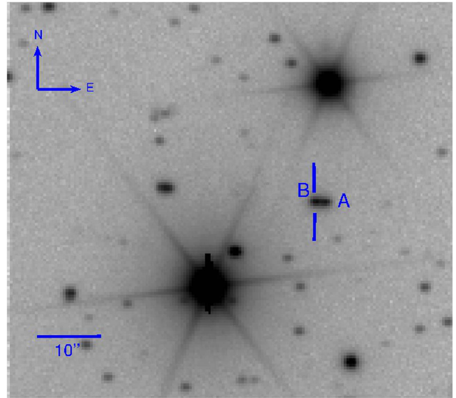
Figure 1. The r -band optical image of the sky region around the BL Lac object IES 0033+595 obtained at the GTC. The source flagged as “A” is a foreground star, and the BLL is the source labeled as “B.”
