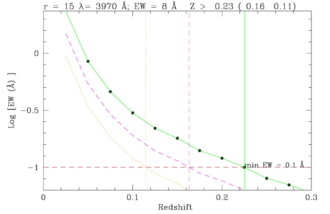
Figure 8. The relation between the EW of the Ca II absorption feature (assuming EW = 8 \text{ Å} ) and the redshift for the spectrum of a BL Lac object of magnitude r = 15 . The relation assumes that the host galaxy has M(R) = -22.9 (green solid line and solid circles). The other two similar relations are for M(R) = -22.4 (magenta dashed line) and M(R) = -21.9 (orange dotted line). The dashed horizontal line gives the assumed EW_{\min} level ( 0.1 \text{ Å} ), and the vertical lines represent the intersection with the above relationships with EW_{\min} level. In this case the redshift is z > 0.23 (for the average host galaxy; other values in parentheses).
