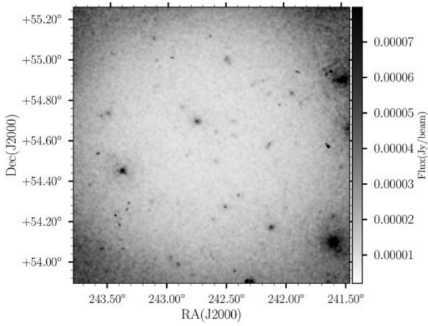
Figure 2. Grey-scale image showing the local rms noise of the final mosaicked GMRT image, derived using PYBDSF (see Section 2.2). The grey-scale brightness stretch ranges between 0.01 and 0.07 \text{ mJy beam}^{-1} .
