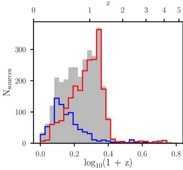
Figure 10. Redshift distribution for the GMRT 610 MHz sources. The grey histogram represents all the redshifts (i.e. both spectroscopic and photometric redshifts). The blue and red histograms represent spectroscopic and photometric redshifts, respectively.
