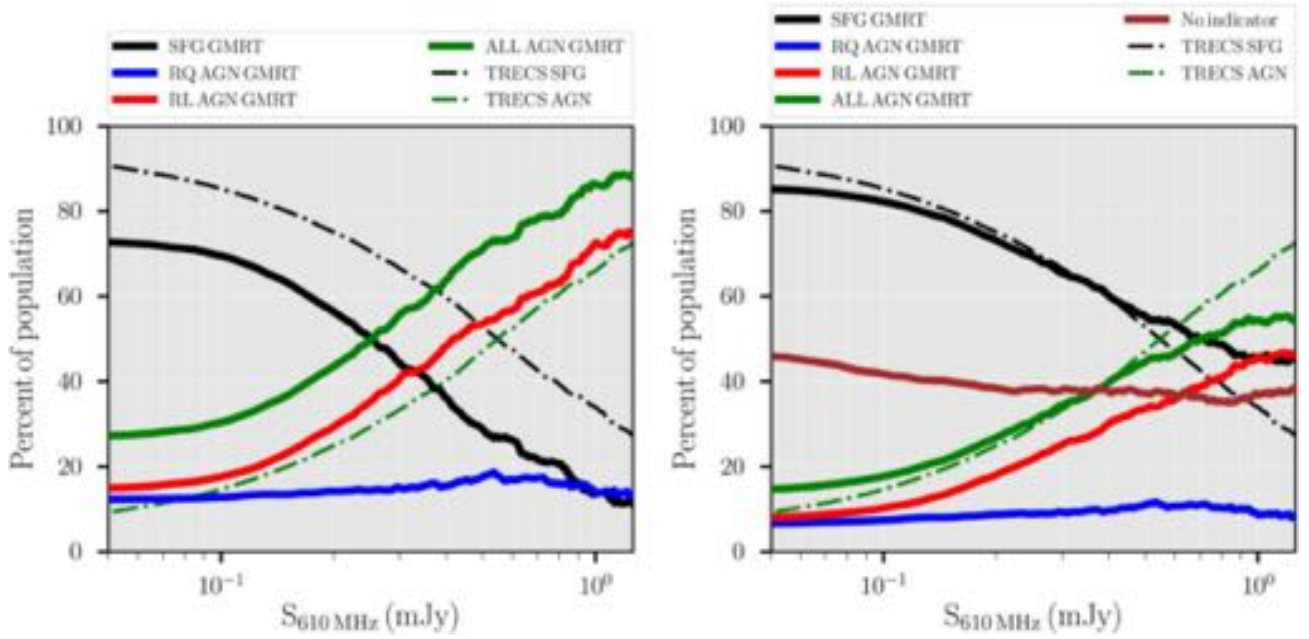
Figure 13. The relative fraction of AGNs and SFGs as a function of minimum flux density. The solid lines show the fraction of the sample with a flux density greater than S_{610 \text{ MHz}} which is classified as RQ AGN (blue), RL AGN (red), all AGN (green), and SFG (black). The dashed dotted green and black lines in both panels represent the relative fraction of AGN and SFG predicted by T-RECS (Bonaldi et al. 2019).
