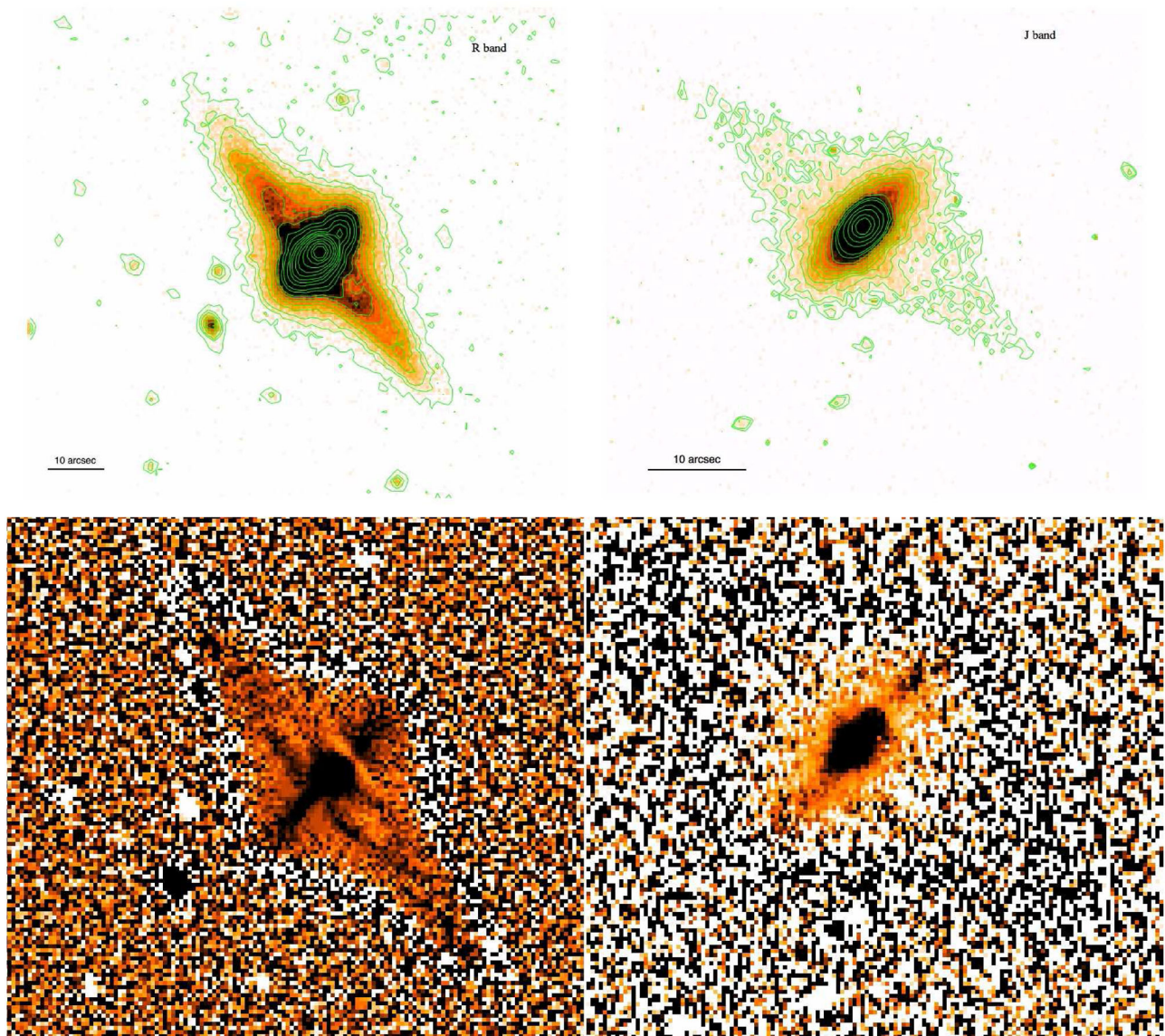
Figure 2. Top panels – the PRG A0136-0801 in the R band (left-hand panel, the image size is 96 \times 87 \text{ arcsec}^2 ) and in the J band (right-hand panel, the image size is 55 \times 50 \text{ arcsec}^2 ). North is up and east is on the left. The low- and high level of the contours (green lines) correspond to \mu_{\text{low}}^R = 23.87 \text{ mag arcsec}^{-2} and \mu_{\text{high}}^R = 15.52 \text{ mag arcsec}^{-2} , in the R band, and \mu_{\text{low}}^J = 20.78 \text{ mag arcsec}^{-2} and \mu_{\text{high}}^J = 16.42 \text{ mag arcsec}^{-2} , in the J band. Bottom panels – enlargement of the high-frequency residual images in the R band (left) and J band (right). Darker colours correspond to brighter features. The image size is 71 \text{ arcsec} \times 65 \text{ arcsec} for the R -band image and 41 \text{ arcsec} \times 37 \text{ arcsec} for the J -band image.
