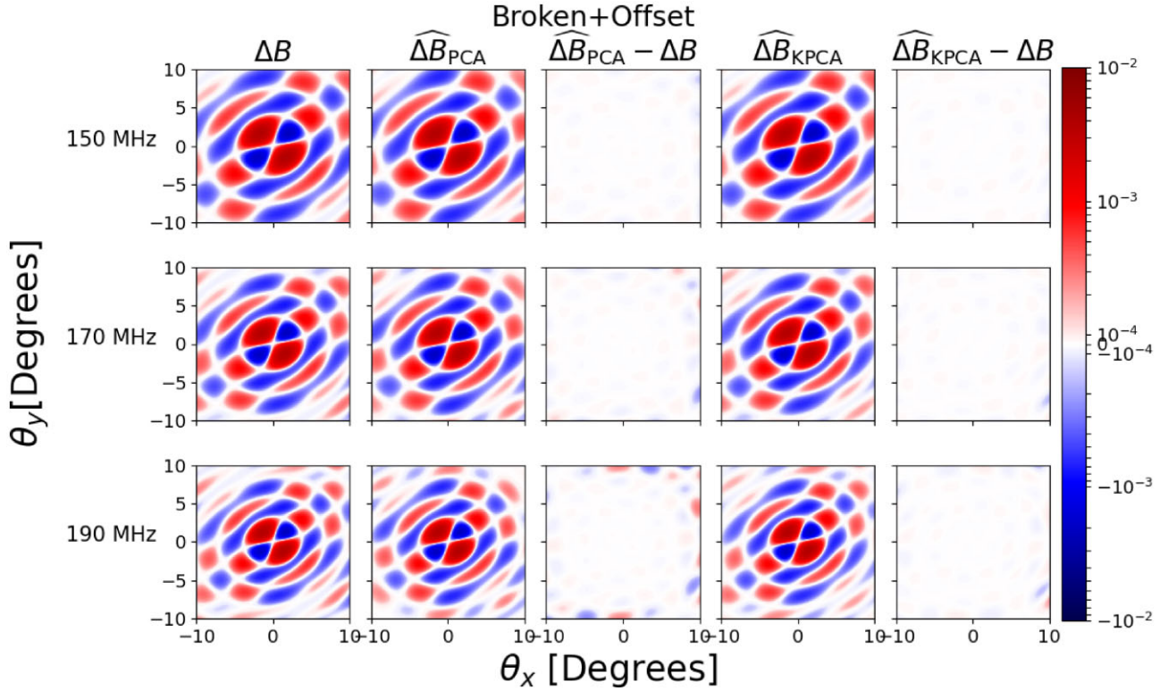
Figure 5. From left to right, the actual beam error ( \Delta B ), the PCA-reconstructed beam error ( \widehat{\Delta B}_{\text{PCA}} ), the difference between the PCA-reconstructed and actual error ( \widehat{\Delta B}_{\text{PCA}} - \Delta B ), the KPCA-reconstructed beam error ( \widehat{\Delta B}_{\text{KPCA}} ), and the difference between the KPCA-reconstructed and actual error ( \widehat{\Delta B}_{\text{KPCA}} - \Delta B ) from one sample realization of the broken + offset data for all three frequencies. In this example, the standard deviation of the fractional difference between the reconstructed and actual error over all \theta , \phi and \nu for PCA and KPCA is 344.1 and 114.68, respectively.
