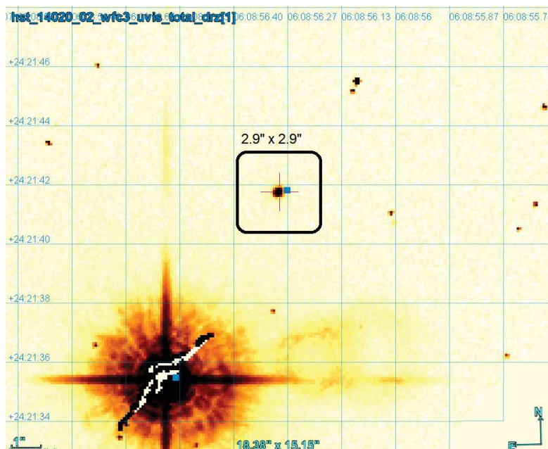
Figure 70: Cl* NGC 2168 BSB 5173 – Star in open cluster source_id=3426270715411638912, G=15.81 , R_{FGS}=15.49 , P1=0.83
