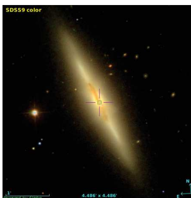
Figure 82: NGC 4710 – HII Galaxy source_id=3931025923551506944, G=18.19 , R_{FGS}=17.81 , P1=0.79
