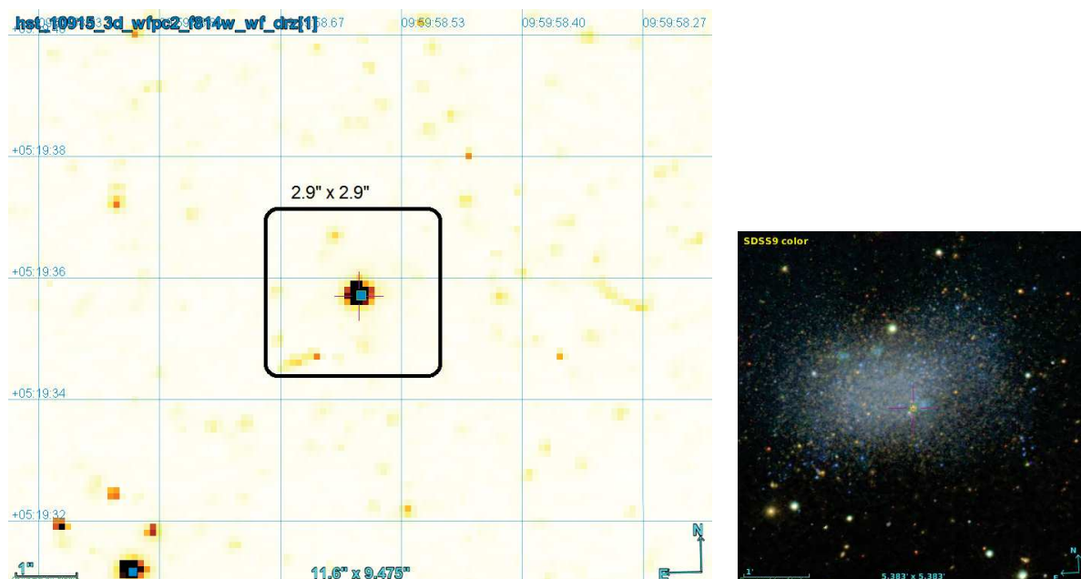
Figure 84: EV* SexB V0005 – Variable Star of irregular type in dwarf galaxy source_id=3849400001370256384, G=18.40 , R_{FGS}=17.95 , P1=0.73
