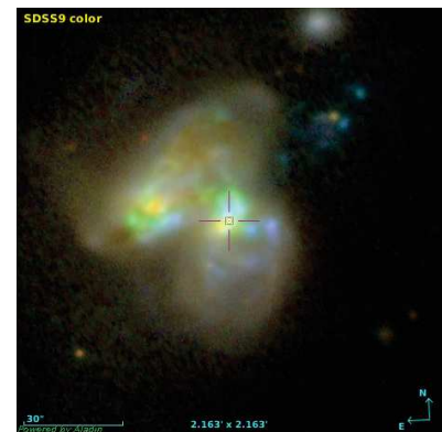
Figure 68: SDSS J112830.77+583342.9 – Interacting Galaxy (Star Formation Region) source_id=858231978679564160, G=15.46 , R_{FGS}=15.10 , P1=0.84
