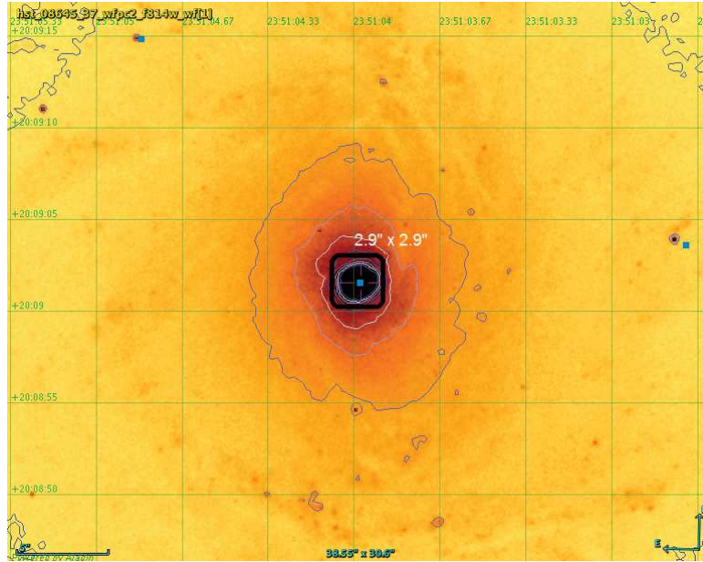
Figure 67: NGC 7769 – LINER-type Active Galaxy Nucleus source_id=2823242193058306048, G=15.20 , R_{FGS}=14.83 , P1=0.86
