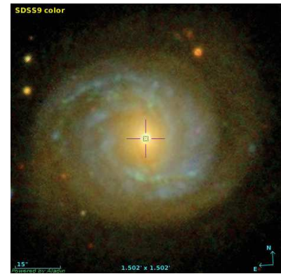
Figure 67: NGC 7769 – LINER-type Active Galaxy Nucleus source_id=2823242193058306048, G=15.20 , R_{FGS}=14.83 , P1=0.86
