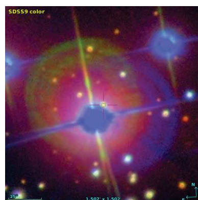
Figure 70: Cl* NGC 2168 BSB 5173 – Star in open cluster source_id=3426270715411638912, G=15.81 , R_{FGS}=15.49 , P1=0.83
