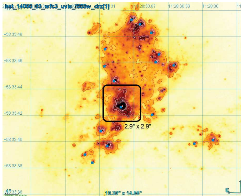
Figure 68: SDSS J112830.77+583342.9 – Interacting Galaxy (Star Formation Region) source_id=858231978679564160, G=15.46 , R_{FGS}=15.10 , P1=0.84
