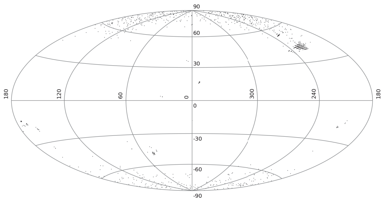
Figure 22: Location of the substandard FOVs (galactic coordinates).
