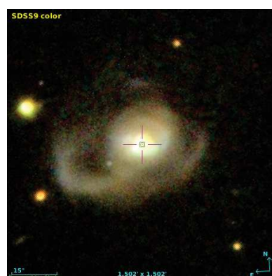
Figure 69: Mrk 334 – Seyfert 1 Galaxy source_id=2847176568328836736, G=15.83 , R_{FGS}=15.39 , P1=0.92
