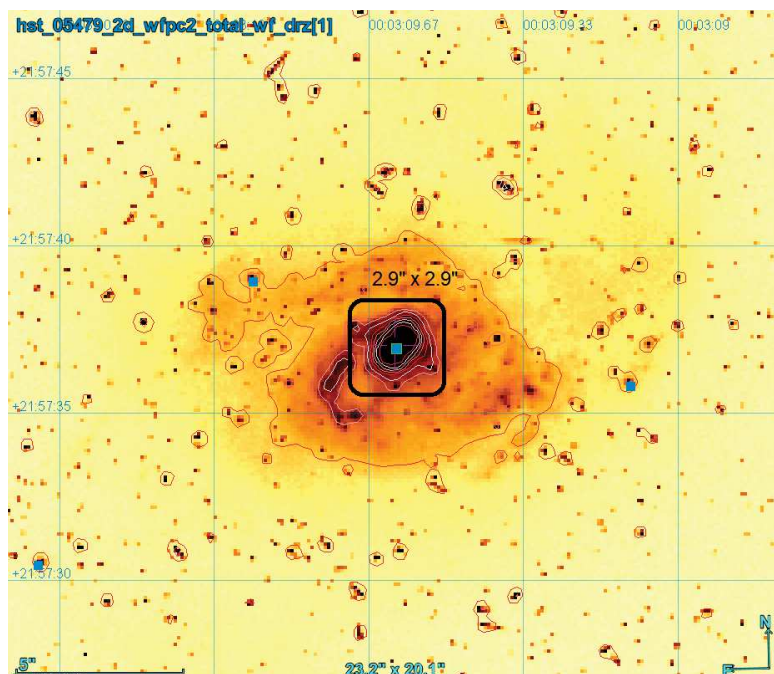
Figure 69: Mrk 334 – Seyfert 1 Galaxy source_id=2847176568328836736, G=15.83 , R_{FGS}=15.39 , P1=0.92
