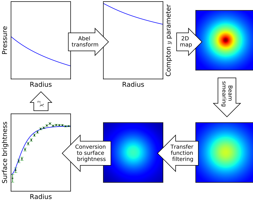
Fig. 1. Block diagram showing the program flow.
