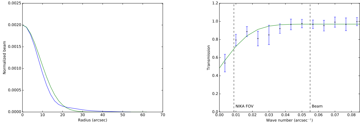
Fig. 2. Left panel: beam profile. Right panel: transfer function profile. Measured profiles are in blue, the approximations used for Fig. 6 in green.
