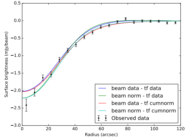
Fig. 6. Surface brightness profiles derived for various combinations of beam and transfer function, as specified in the inset, for a single set of pressure profile parameters. Points with 68% error bars show the data.
