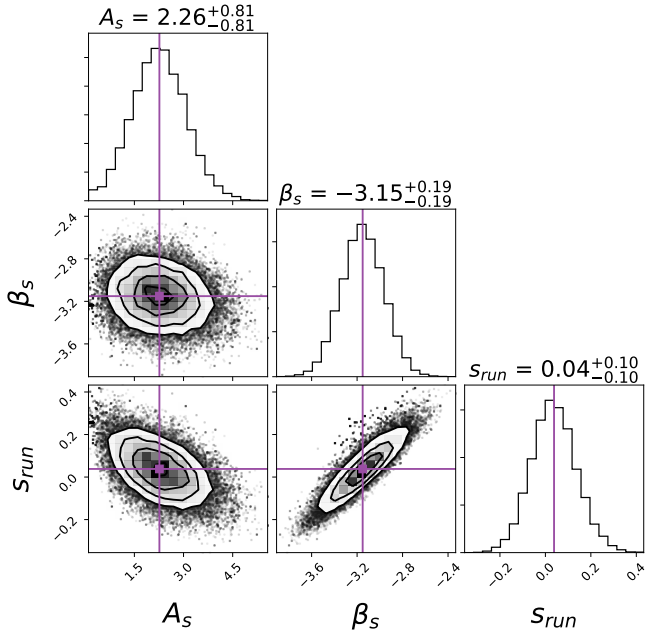
Fig. 8. Posterior distribution of the parameters obtained by fitting the model in 3 to BB power spectra of S-PASS, Planck and WMAP in the multiple bin at \ell \approx 50 and for the isolatitude mask with |b| > 35^\circ . The fit has been computed by applying a Gaussian prior on the synchrotron spectral index with \beta_s = -3.13 \pm 0.13 .
