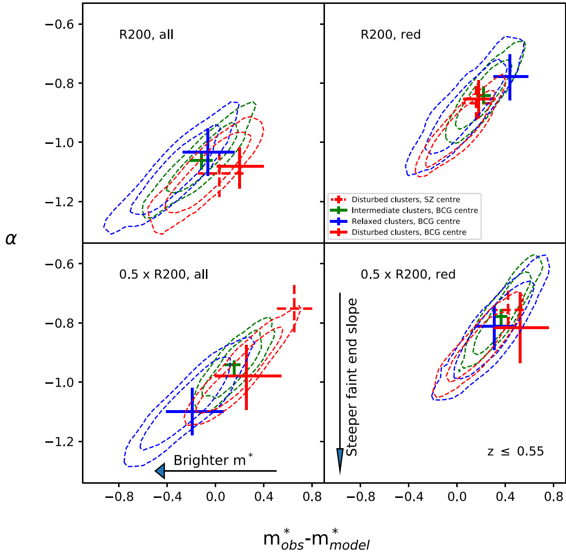
Figure 11. \alpha - \Delta m^*(m_{\text{obs}}^* - m_{\text{model}}^*) for cluster galaxies (all) and RS galaxies (red), within 1 and 0.5 r_{200} , at z \leq 0.55 . We obtain m_{\text{obs}}^* by fitting the data, while m_{\text{model}}^* corresponds to the model as discussed in Section 2.4. Solid red crosses represent disturbed clusters using the BCG as a centre (26 clusters), dash red crosses represent disturbed clusters using the SZ centroid as a centre, blue crosses correspond to the relaxed sample (16 clusters) while green crosses correspond to the intermediate sample (see Section 4.1.3 for details; 111 clusters), both using the BCG as a centre. Dashed red/blue contours correspond to 68 per cent and 90 per cent of the fits, when the centre is randomized 600 times within 0.4-1 r_{200} of the SZ centre, for the disturbed/relaxed sample. Green contours correspond to 68 per cent and 90 per cent of the fits, obtained by stacking 26 randomly selected clusters from the intermediate cluster sample, using the BCG as a centre 600 times. At this redshift range all cluster populations seems to occupy a very similar \alpha - \Delta m^* parameter space.
