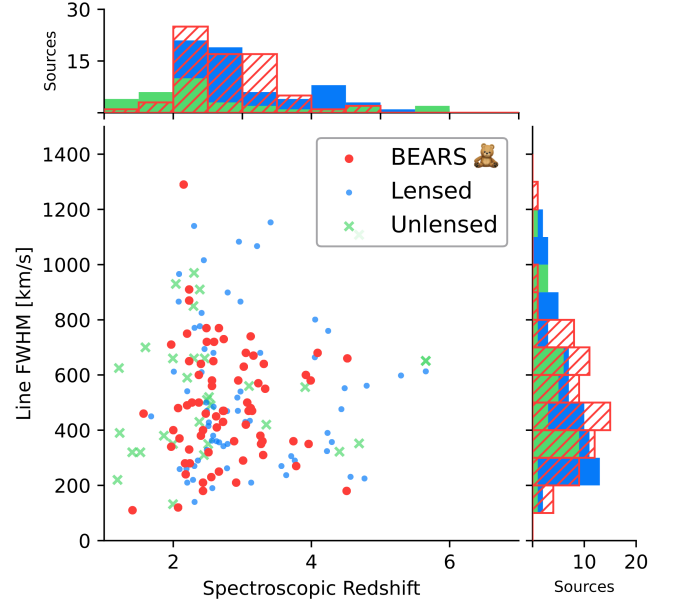
Figure 5. Distribution of the spectroscopic redshifts and linewidths of the 71 BEARS galaxies presented in this work, compared to the samples described in the text.
