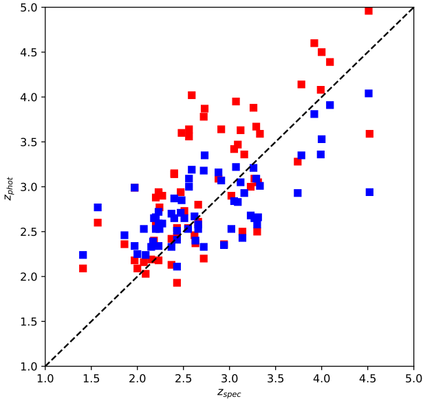
Figure 4. Comparison of the spectroscopic redshifts presented here with the photometric redshifts from Bakx et al. (2018) shown in red and from Ivison et al. (2016) shown in blue. Our results are consistent with the spread seen in, e.g., Ivison et al. (2016), Bakx et al. (2018), Pearson et al. (2013). Note that this diagram is necessarily restricted to objects with spectroscopic redshifts.
