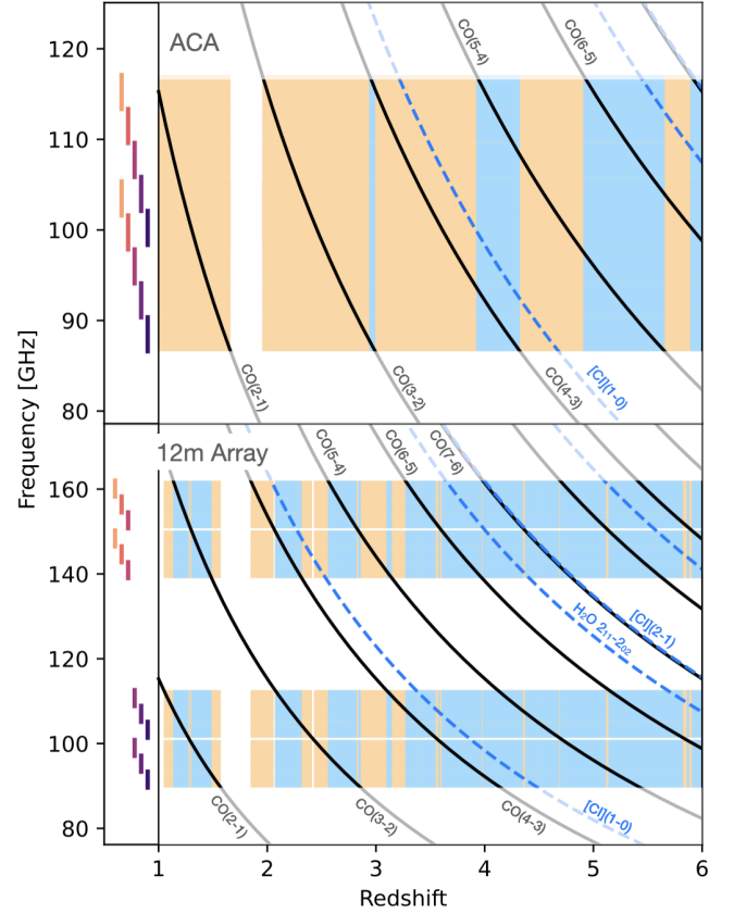
Figure 2. Redshift as a function of frequency for the ACA Band 3 spectral coverage (86.6–115.7 GHz; top panel) and ALMA 12-m Array (89.6–112.6 and 139–162 GHz; bottom panel) for the ^{12}\text{CO} (solid black lines), CI and water (dashed blue lines) emission lines. The blue areas identify the redshift range where at least 2 CO emission lines fall within this frequency range, and the orange areas show where only one CO line falls within the frequency range. “Redshift deserts” are shown as white areas. The coloured bars at the left-hand side of the plots show the location of the spectral tunings that were used for the ACA and 12-m Array. Our 12-m Array tunings (Section 2.3) dramatically improved our ability to find robust redshifts drastically from an estimated 12 to 90 per cent using only one extra tuning.
