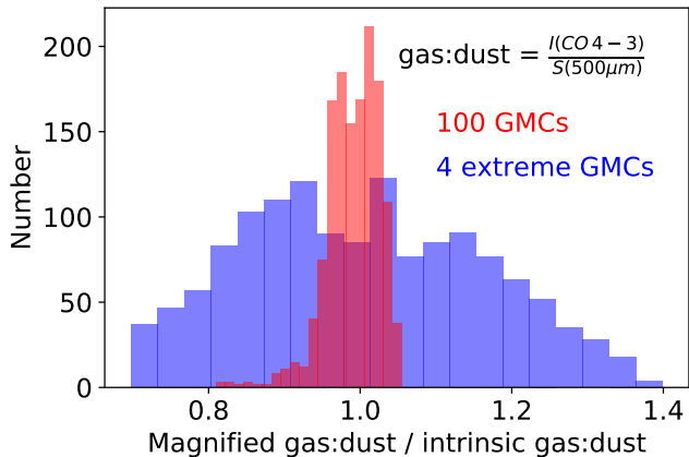
Figure 7. Simulation of differential magnification effects on a submm galaxy at z = 2.286 lensed by a z = 0.9 foreground galaxy. The blue histogram shows random realisations assuming the star formation is confined to only four giant molecular clouds as claimed originally for the Cosmic Eyelash by Swinbank et al. (2010), while the red histogram with narrower bins shows the distribution of random lensing realisations with star formation distributed over 100 identical molecular clouds, as suggested by the smooth continuum observed by Ivison et al. (2020). Note the much narrower distribution when the star formation is spread more uniformly throughout the system (red), and the wider distribution when the star formation is concentrated into a very small number of clumps (blue).
