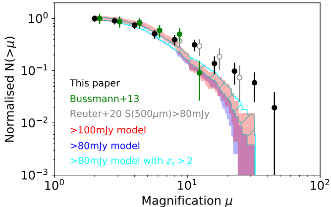
Figure 8. Observed cumulative magnification distribution of lensed submm galaxies (magnifications \mu \geq 2 ) with redshifts from this paper, compared to the LensPop submm population discussed in the text with a flux limit of > 100 mJy (red) and > 80 mJy (blue), and with a HERBS-like additional selection of source redshift z_{\text{source}} > 2 (cyan hatched). The shaded areas represent the Poisson uncertainties in the numbers from the model realisations. Note the good agreement between data and models over most of the magnification range, but the hint of an excess at large magnifications. Also shown is the magnification distribution from the 500\text{ }\mu\text{m} -selected sample of Bussmann et al. (2013), and the South Pole Telescope targets with \geq 80 mJy at 500\text{ }\mu\text{m} and with modelled magnifications (Reuter et al. 2020), though note that the latter data points have flux limits at a total of three wavelengths so are not straightforwardly comparable.
