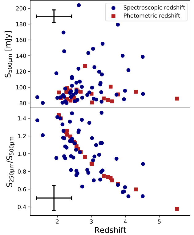
Figure 1. Top panel: 500 \mu\text{m} flux density against redshift. Sources with spectroscopic redshifts are shown as blue dots , while sources with only photometric redshifts are shown as red squares . Sources are selected with 500 \mu\text{m} greater than 80 mJy. We show the typical uncertainties on these values in the top-left of the figure, assuming a z_{\text{phot}} = 3 . For sources with multiple galaxies at different redshifts, we use the average spectroscopic redshift. Bottom panel: Submm colours and redshifts of our sample, illustrating the photometric selection function above z_{\text{phot}} = 2 . Typical uncertainties in the colour and photometric redshift estimates are shown in the bottom-left of the graph.
