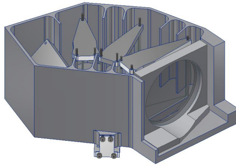
Figure 15: prisms sub-bench.
