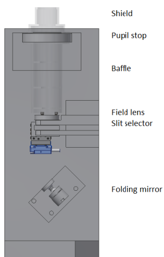
Figure 14: slit sub-bench.
