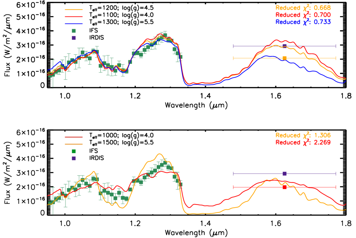
Fig. 7. Upper panel: Spectrum extracted for HR 2562 B (green squares) with its error bars. The colored solid lines represent the three best fitting spectra from the BT-Settl synthetic spectra. Orange square is obtained from the corresponding spectrum calculating the flux on the IRDIS H broad band filter to be able to better compare it with the IRDIS data. The same operation was not done for the other spectra to avoid confusion in the final plot. Lower panel: Same as upper panel, but using synthetic spectra with poorer fits.
