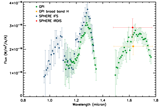
Fig. 4. Low resolution spectrum for HR 2562 B (blue circles) compared to the GPI spectrum for the same object (green squares). The red circle is the spectral point derived from IRDIS where the large error band on the wavelength scale denotes that it is derived with a broad band filter. The orange square is derived from the GPI data considering the same wavelength range of the IRDIS broad band filter to be able to make a comparison between the two instruments.
