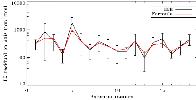
Figure 25: Comparison of the LO residual on axis from the end-to-end simulations and from the formula, for 18 random asterisms and 2 DMs.
