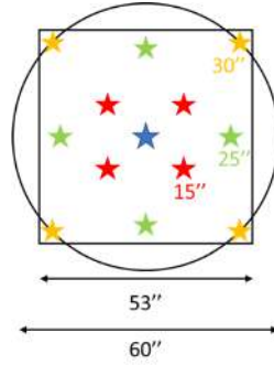
Figure 5: Directions used for the jitter/SR computation in the FoV of diameter 60''. The square of side 53'' corresponds to the large MICADO FoV. The stars are distributed as follows: 1 star on axis, 4 stars at 15'', 4 stars at 25'' and 4 stars at 30''. When the small MICADO FoV is considered (20×20''), we average from 1 star on axis and 4 stars at 10'' (placed in the same manner as the 4 stars at 15'').
