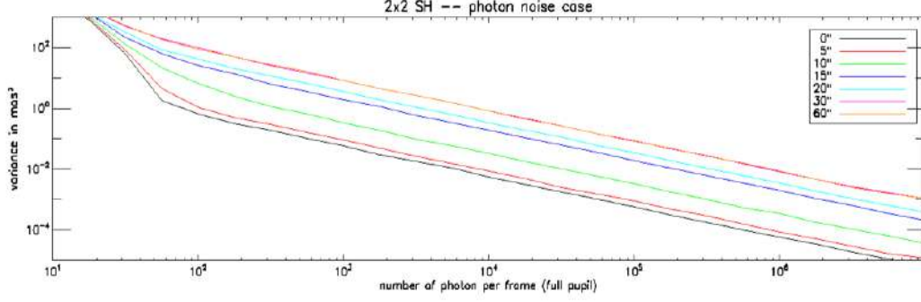
Figure 4: Example of noise computed for a 2x2 SHWFS, for different level of fluxes, and different position of the NGS in the field, in the case of an LTAO correction without OLDLM.
