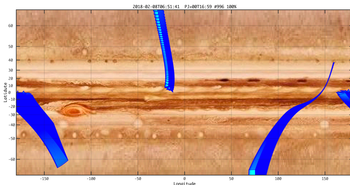
Figure 3: Coverage Nadir
