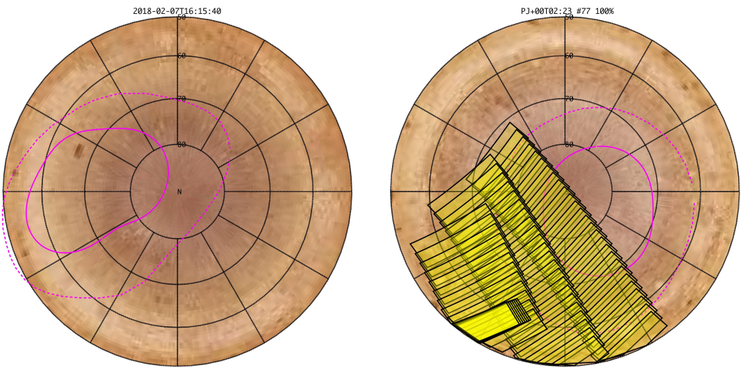
Figure 1: South Aurora.
