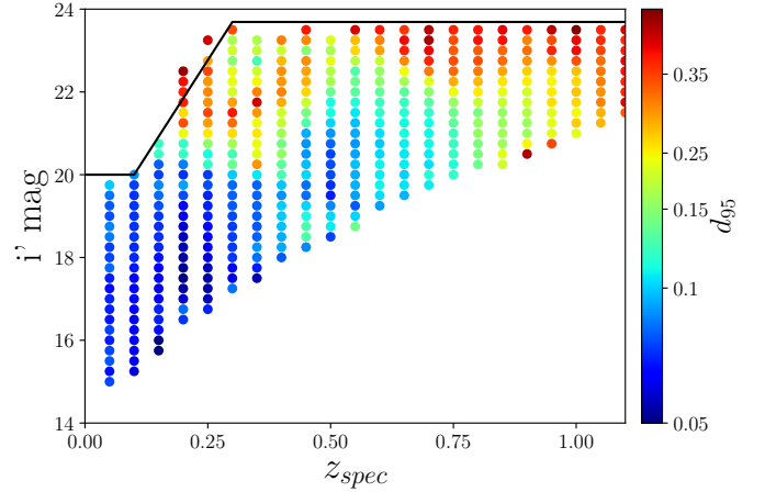
Fig. 5. Photometric redshift dispersion d_{95} , computed as the 95th percentile of |z_{\text{phot}} - z_{\text{spec}} - \text{bias}(z_{\text{spec}})| in the (z, i' \text{mag}) plane. The dots indicate the centres of the \Delta(z, i' \text{mag}) = 0.1 \times 0.5 cells used to compute the dispersion (if they contain at least 30 objects). The continuous black line shows the limiting magnitude we impose for the rest of the study.
