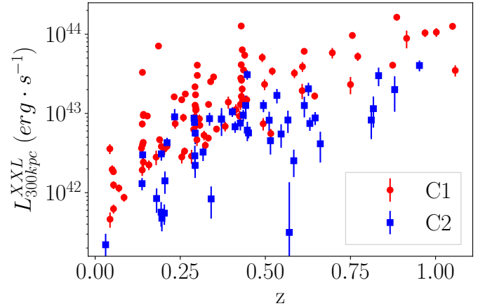
Fig. 1. X-ray luminosity in the [0.5-2] \text{ keV} band computed in a 300 kpc aperture as a function of redshift for the cluster sample used in this study. Red points and blue squares represent clusters classified as C1 and C2, respectively (see text).
