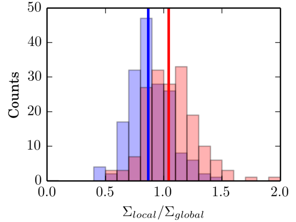
Fig. 7. Histogram of the ratio between local and global background galaxy number densities. Global backgrounds refer to the whole CFHTLS W1 field, whereas local backgrounds refer to annuli of 3–5 Mpc centred on the X-ray cluster positions. The distribution of the ratio when structures are discarded from (taken into account in) the local background fields is shown in blue (red). The solid lines indicate the median values of the ratios.
