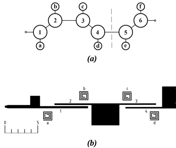
Fig. 1. (a) Architecture of the notch filter; (b) geometrical layout of part of the filter. Slightly more than half geometry is drawn in (b), corresponding to the left of the dashed line in (a), due to its symmetry. The scale is given in mm
