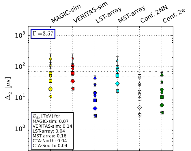
Figure 3. Uncertainty in the position of the interpulse P2 ( \Delta_2 ) of the VHE profile of the Crab pulsar, simulated for MC PROD2 Conf. 2NN (white) and Conf. 2e (green). Results for MAGIC (yellow), VERITAS (red) and the CTA LST-array (blue) and MST-array are also shown. The spectral index of the Crab pulsar spectrum used in these simulations is \Gamma = 3.57 (see Section 2). Different markers correspond to observations of different durations in units of the MAGIC observing time ( t_{\text{obs}}^{\text{M}} = 72.78 h): 0.1 (triangles), 0.3 (stars), 1 (circles), 1.5 (thin diamonds), 3 (squares), 10 (diamonds), 30 (rotated triangles). Error bars represent the standard deviation calculated from a set of simulations. The dashed and dot-dashed lines show the uncertainties of the MAGIC ( \Delta_2 = 50 \mu\text{s} ; Aleksić et al. 2012b) and VERITAS ( \Delta_2 = 70 \mu\text{s} ; Aliu et al. 2011) observations, respectively.
