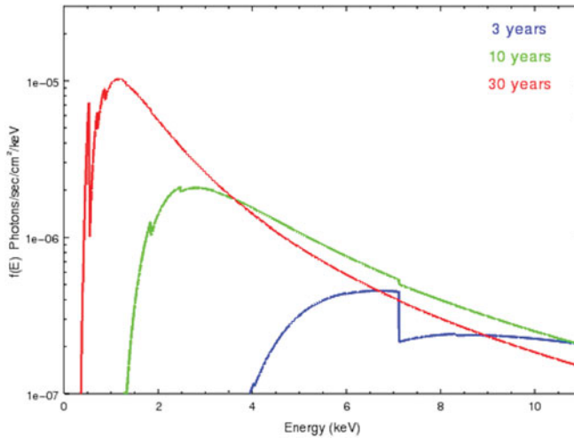
Figure 1. Estimated emerging PWN X-ray spectra, for the model and parameter values described in the text, at t_{\text{age}} = 3, 10 and 30 years after the supernova explosion.
