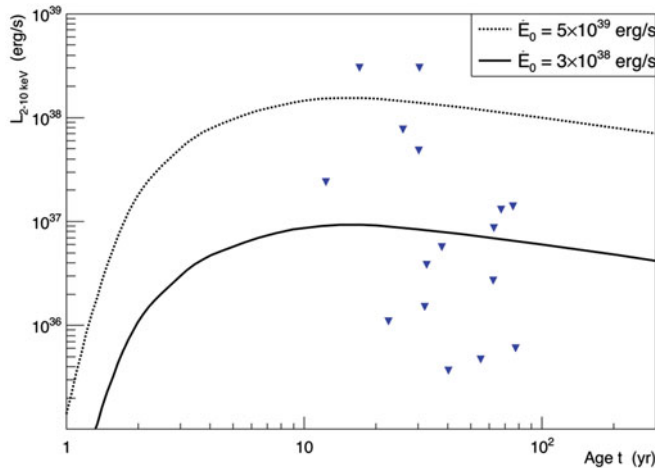
Figure 2. Estimated emerging PWN X-ray fluxes for the model and parameter values detailed in Sect. 2 and two representative values of \dot{E}_0 , along with upper limits from Perna et al. (2008).
