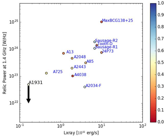
Figure 4. Specific luminosity at 1.4 GHz of AGN/phoenix relics from Nuza et al. (2017) versus the X-ray luminosity of their host cluster in 10^{44} \text{ erg s}^{-1} . The colour of the points represents their largest linear scale/size in Mpc. The X-ray luminosity of the clusters 24P73 and MaxBCG 138+25 is not known.
