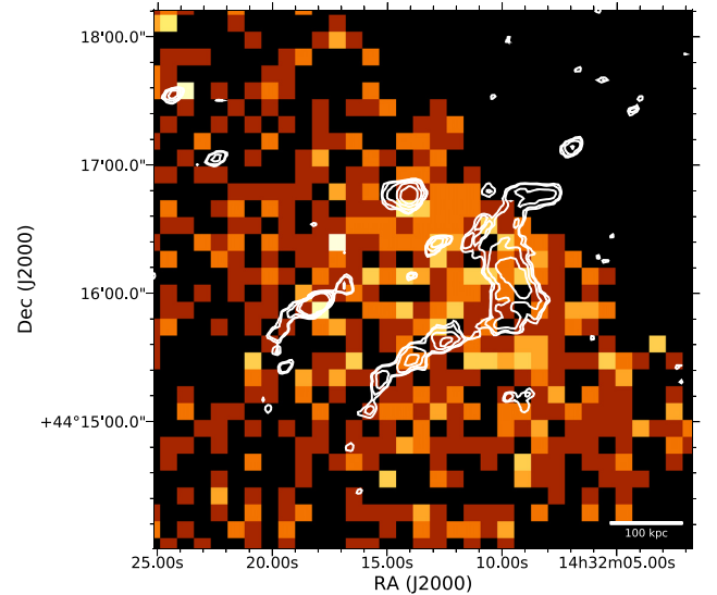
Figure 3. Chandra map with LOFAR contours overlaid. The LOFAR contours start at 3\sigma ( 0.56 \text{ mJy beam}^{-1} ) and increase by a factor of 2. The image (0.5–2 keV, exposure-corrected) was binned such that each pixel is 16 \times 16 original pixels in order to make the emission more visible. The cross marks the location of the BCG.
