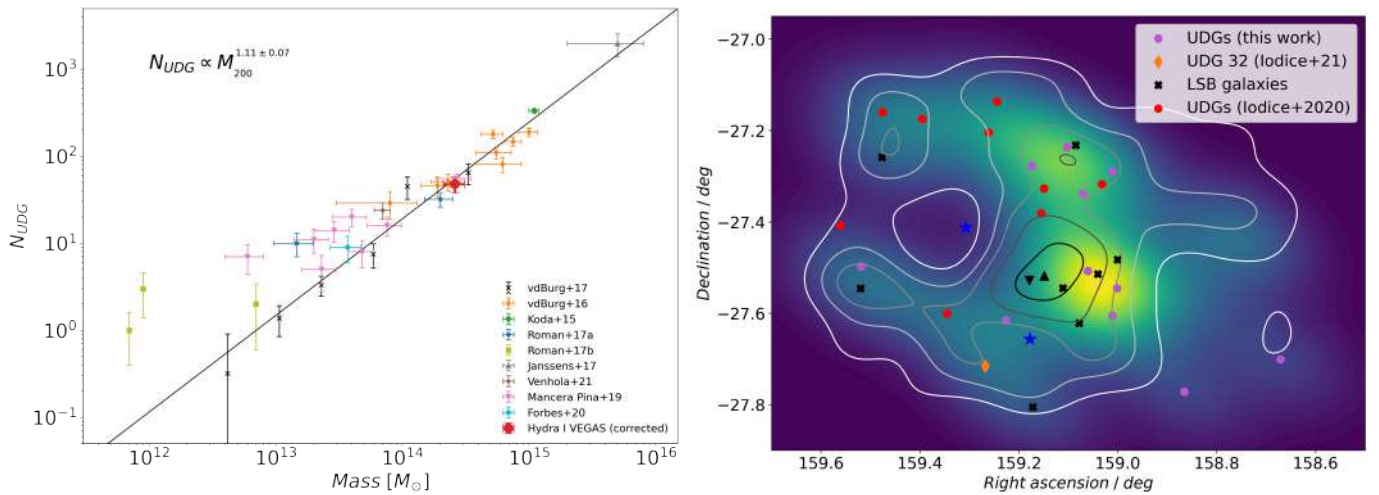
Fig. 6. UDG numerical abundance and spatial distribution. Left panel: abundance of UDGs as a function of the halo mass for available data (van der Burg et al. 2017, 2016; Koda et al. 2015; Román & Trujillo 2017a,b; Janssens et al. 2017; Mancera Piña et al. 2019; Forbes et al. 2020b; Venhola et al. 2022). For the Hydra I cluster, the number of UDGs within \approx 0.4R_{vir} is scaled to N_{UDG}(\leq R_{vir}) on an assumed radial number density distribution (see Sect. 5.1). The black line represents the relation fitted by van der Burg et al. (2017), the equation for which is reported in the plot. Right panel: 2D projected distribution of all the UDGs detected in the Hydra I cluster, and of the 8 LSB galaxies presented in this work (sequential color map). Contours represent the density distribution of dwarf galaxies (see Paper I), with increasing density from white to black. The two brightest cluster members NGC 3311 and NGC 3309 are marked as black triangles. The locations of the two brightest stars in the field are also indicated as blue stars.
