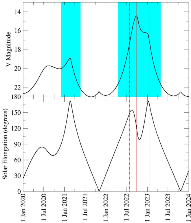
Figure 3. V magnitude (top) and solar elongation (bottom) for the Didymos system over 2020–2023. Note that the y-axis for the top panel is inverted to represent larger magnitudes being fainter. Didymos spends an extended period as a bright object at large solar elongations during the DART impact epoch in 2022–2023, with two separate oppositions. Shaded regions on the top panel represent periods when Didymos is >90^\circ from the Sun. The solid red vertical line represents an impact date of 2022 September 30. The period between the two vertical dashed lines is the period when Didymos is brighter than V = 17.5 and meter-class telescopes can obtain data that can meet required photometric precision in typical conditions (Section 3.2.1).
