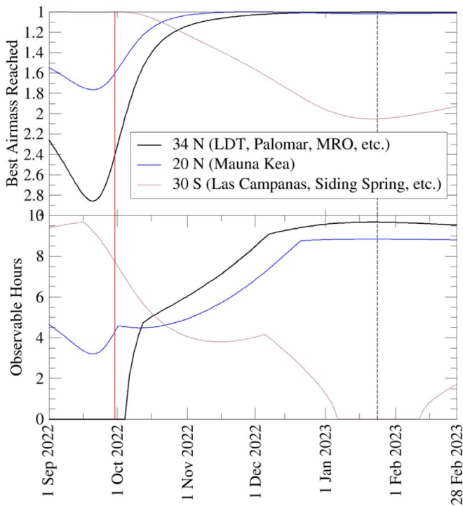
Figure 4. Best air mass (astronomically defined as the secant of the zenith angle, so air mass overhead = 1.0) reached by Didymos (top) and the number of hours above 30° elevation (i.e., air mass <2) for three latitudes during the DART impact apparition. These latitudes are representative ones for southern hemisphere observatories (30°S), Hawaiian observatories (20°N), and the observatories of the U.S. Southwest (34°N). As in Figure 3, the dashed line marks the time after which Didymos is fainter than V = 17.5 . Early in the apparition, observations from Las Campanas (and other observatories at similar southern latitudes) are best, with Didymos spending long periods high in the sky. By late October, northern hemisphere observatories have observing circumstances as good as southern hemisphere locations and are better sites for Didymos observations through late 2022 into early 2023.
