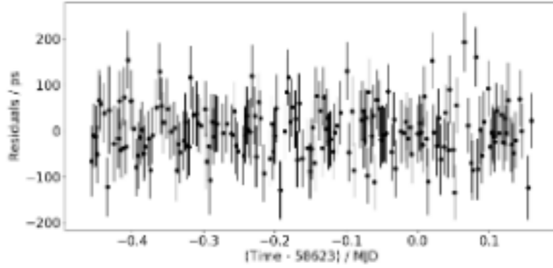
Figure 1: Post-fit group delay residuals as a function of observing time for the geodetic VLBI experiment VI007 in which Matera and Medicina shared the same remote frequency reference from INRiM (Torino).
