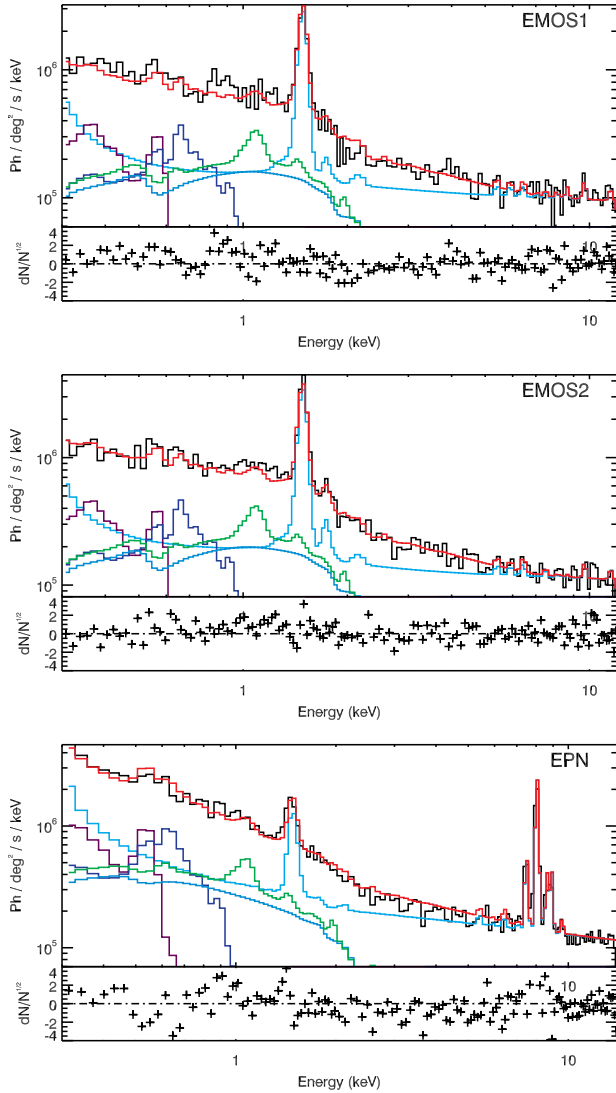
Fig. 2. Joint-fit of XMM-Newton EPIC background and cluster emission from MKW 08. From top to bottom : background fitting of MOS1, MOS2 and PN cameras. Total number of counts (black); thermal emission of LHB (purple); thermal emission of GTE (dark blue); power-law emission from CXB (blue); quiescent particle background emission (cyan); cluster emission (green); total background emission (red). Residuals correspond to the total photon count with respect to the ICM and total background emission.
