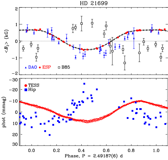
Figure C2. Top: \langle B_z \rangle measurements for HD 21699, obtained from Brown et al. (1985), DAO, and ESPaDOnS data, folded with the rotation period. Solid/dashed curves show the third-order harmonic fit to the ESPaDOnS data and the fit uncertainty. Bottom: TESS and Hipparcos light curves folded with the rotation period.
