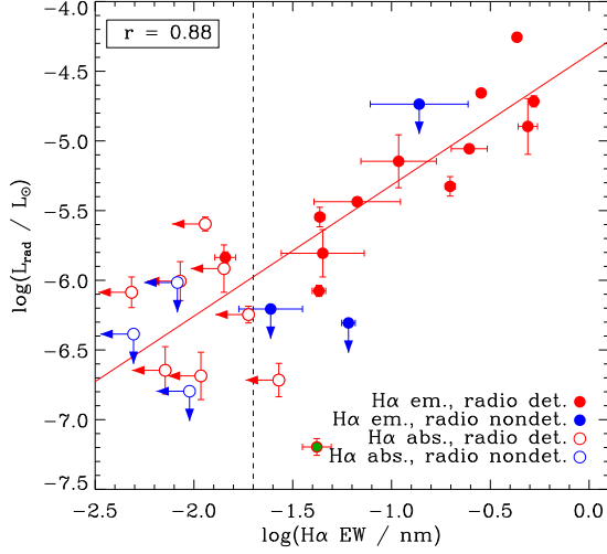
Figure 6. Radio luminosity as a function of H \alpha emission equivalent width. The solid diagonal line shows a fit to the measurements of stars detected in both H \alpha and radio. The vertical dashed line indicates the approximate noise floor identified by Shultz et al. (2020). Red and blue points are stars detected and not detected in the radio; filled and open symbols are stars with H \alpha in emission and absorption respectively. HD 64740 is highlighted with dark green.
