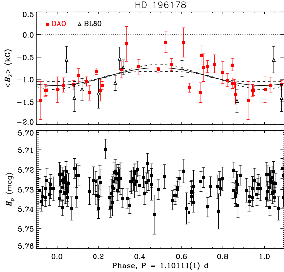
Figure C35. \langle B_z \rangle measurements of HD 196178 ( top ) and Hipparcos light curve ( bottom ) phased with the period determined from the magnetic data.
