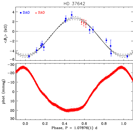
Figure C12. Top: DAO and SAO \langle B_z \rangle measurements for HD 37642, phased with the TESS rotation period. Bottom: TESS photometry phased with the rotation period.
