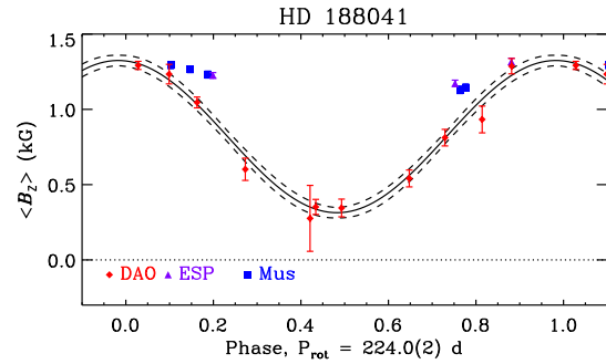
Figure C34. \langle B_z \rangle measurements of HD 188041 phased with the period determined from the same measurements.
