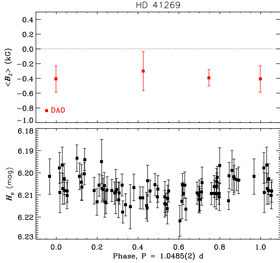
Figure C14. Top: DAO SAO \langle B_z \rangle measurements for HD 41269, phased with the Hipparcos rotation period. Bottom: Hipparcos photometry phased with the rotation period.
