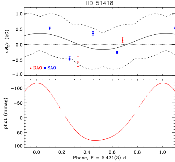
Figure C15. Top: DAO and SAO \langle B_z \rangle measurements for HD 51418, phased with the TESS rotation period. Bottom: TESS photometry phased with the rotation period.
