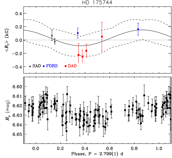
Figure C30. Top: \langle B_z \rangle measurements of HD 175744 folded with the rotation period inferred from Hipparcos photometry ( Bottom ). The harmonic fit to \langle B_z \rangle is performed to the combined magnetic dataset.
