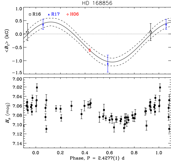
Figure C26. Top: \langle B_z \rangle measurements for HD 168856, obtained from Romanyuk et al. (2016b), Romanyuk et al. (2017b), and Hubrig et al. (2006), folded with the rotation period. Bottom: Hipparcos light curve phased with the rotation period.
