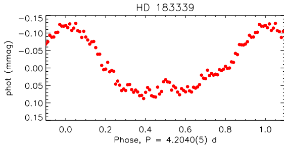
Figure C32. Phase-binned TESS light curve of HD 183339, folded with the strongest period.
