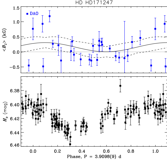
Figure C28. DAO \langle B_z \rangle measurements ( top ) and Hipparcos light curve ( bottom ) of HD 171247 folded with the photometric period.
