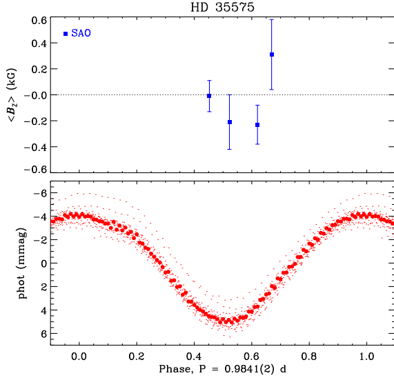
Figure C5. SAO \langle B_z \rangle measurements ( top ) and TESS photometry ( bottom ) of HD 35575 phased with the rotation period. Larger points indicate phase-binned data.
