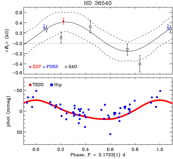
Figure C7. Top: \langle B_z \rangle measurements for HD 36540, obtained from Romanyuk et al. (2017b), Bagnulo et al. (2015a), and ESPaDONs, folded with the rotation period. Solid/dashed curves show first-order harmonic fit and uncertainty. Bottom: Hipparcos and TESS light curves folded with the rotation period. Larger points indicate phase-binned data.
