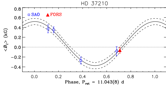
Figure C11. SAO and FORS \langle B_z \rangle measurements for HD 37210.
