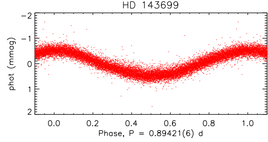
Figure C21. TESS light curve for HD 143699, folded with the rotation period. The data have been pre-whitened with the probable pulsation frequency at 1.12 c/d.
