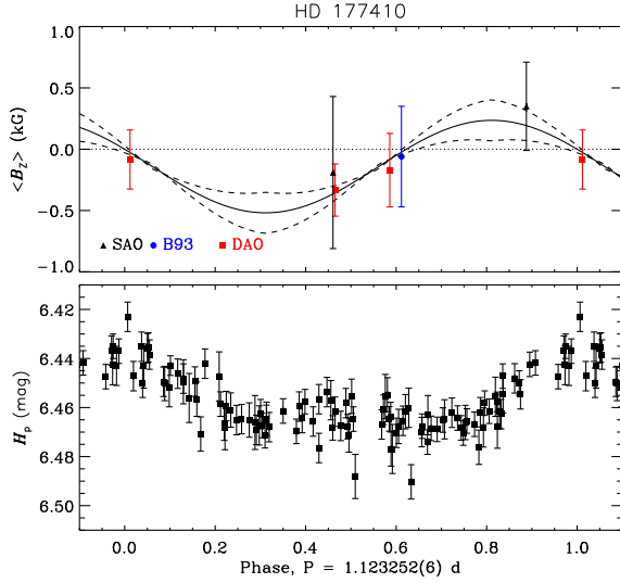
Figure C31. Top: \langle B_z \rangle measurements of HD 177410 folded with the photometric rotation period Bottom: Hipparcos photometry folded with the rotation period. The harmonic fit to \langle B_z \rangle is performed to the combined magnetic dataset.
