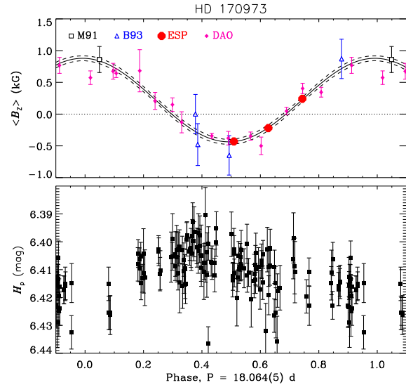
Figure C27. Top: \langle B_z \rangle measurements for HD 170973, obtained from Mathys (1991b), Bohlender et al. (1993a), and ESPaDOnS, folded with the rotation period. Solid curve shows first-order harmonic fit. Bottom: Hipparcos light curve folded with the rotation period.
