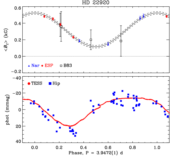
Figure C3. Top: \langle B_z \rangle measurements for HD 22920, obtained from Borra et al. (1983), ESPaDOnS, and Narval, folded with the rotation period. Solid/dashed curves show first-order harmonic fit and uncertainty. Bottom: Hipparcos and TESS light curves folded with the rotation period.
