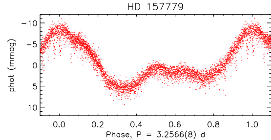
Figure C24. TESS light curve of HD 157779 folded with the rotational period.
