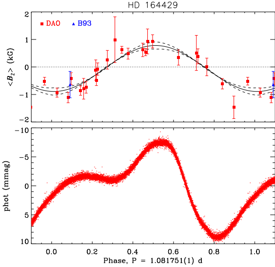
Figure C25. Top: \langle B_z \rangle measurements for HD 164429, phased with the period determined from TESS data. Bottom: TESS light curve folded with the rotation period.
