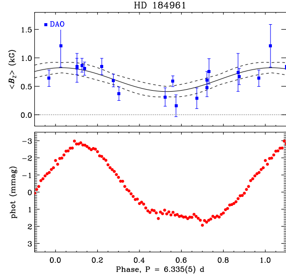
Figure C33. DAO \langle B_z \rangle measurements ( top ) and phase-binned TESS light curve ( bottom ) phased with the period determined from the magnetic data.
