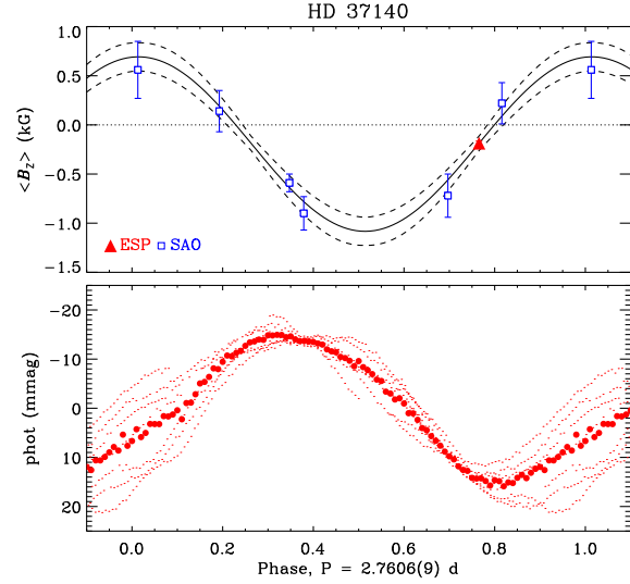
Figure C10. Top : SAO and ESPaDOnS \langle B_z \rangle measurements for HD 37140. Bottom : TESS light curve folded with the rotation period. Larger points indicate phase-binned data.
