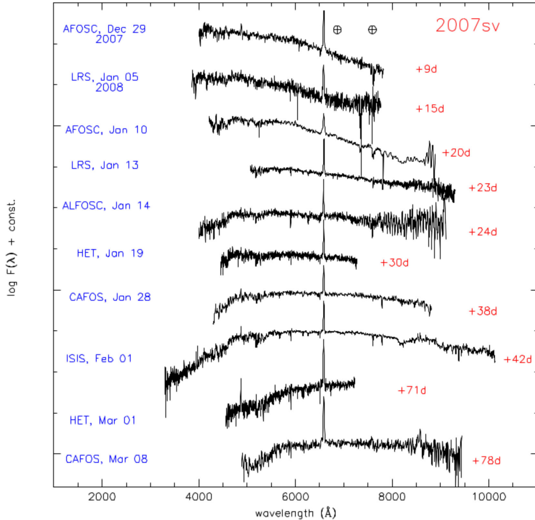
Figure 5. Spectral sequence of 2007sv. The date and the instrumental set-up are reported on the left, the phase (in days after the discovery) is indicated on the right. Spectra are flux-calibrated. The \oplus symbols mark the position of the visible telluric absorptions.
