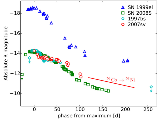
Figure 3. Comparison of the absolute R -band light curves of the impostors 2007sv and 1997bs, the enigmatic transient SN 2008S, and the classical Type II n SN 1999el. The red line indicates the slope of the ^{56}\text{Co} decay.
