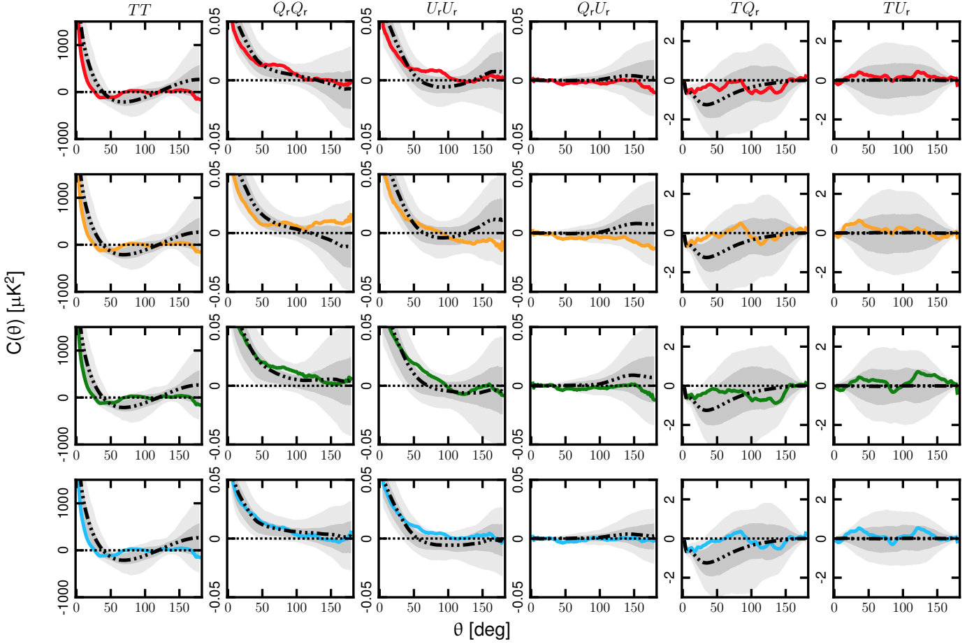
Fig. 8. 2-point correlation functions determined from the N_{\text{side}} = 64 Planck CMB 2018 temperature and polarization maps. Results are shown for the Commander , NILC , SEVEM , and SMICA maps (first, second, third, and fourth rows, respectively). The solid lines correspond to the data, while the black three dots-dashed lines indicate the mean determined from the corresponding FFP10 simulations, and the shaded dark and light grey areas indicate the corresponding 68 % and 95 % confidence regions, respectively.
