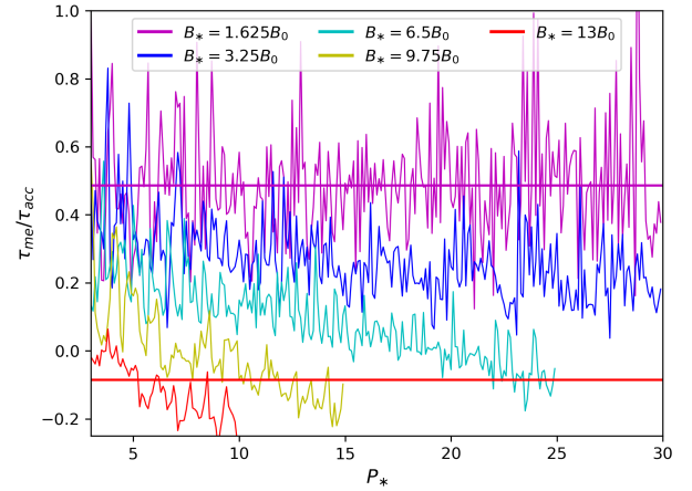
Fig. 11. \tau_{\text{me}}/\tau_{\text{acc}} versus time (given in P_* ). Colors and line styles have the same meaning as in Fig. 9. In the plot, a negative (positive) ratio indicates a spin-down (spin-up) torque due to MEs.
