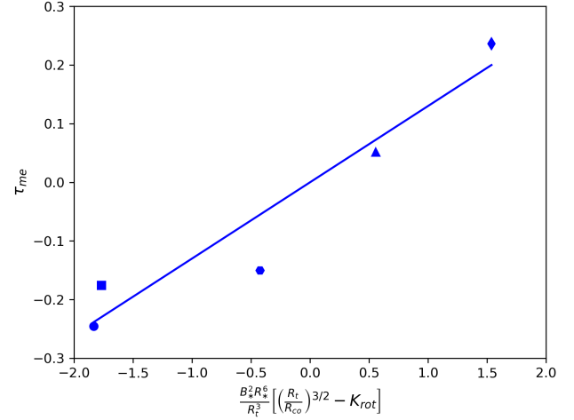
Fig. 10. Normalized \tau_{\text{me}} versus quantity in curly brackets in Eq. (42). Symbols are the same as in Fig. 3. In the plot, a negative (positive) \tau_{\text{me}} spins up (down) the stellar rotation. Using Eq. (42), the best fit to the points gives K_{\text{me}} = 0.13 and K_{\text{rot}} = 0.46 .
