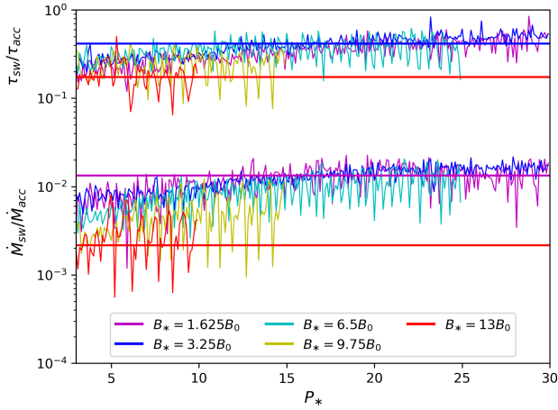
Fig. 9. Absolute values of the mass ejection efficiency \dot{M}_{\text{sw}}/\dot{M}_{\text{acc}} and torque efficiency \tau_{\text{sw}}/\tau_{\text{acc}} as a function of time expressed in units of the stellar rotation period. The straight lines in the plot represent the time-averaged values for the two cases exhibiting the lowest and highest values of these two quantities.
