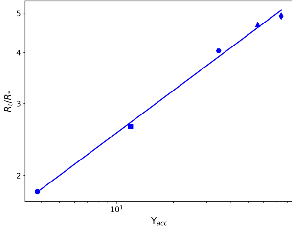
Fig. 3. Normalized truncation radius, R_t/R_* , as a function of parameter Y_{\text{acc}} . Each symbol (or data point) in the plot represents a single SDI simulation. The solid line shows the fitting function (29), with K_t = 1.1452 and m_t = 0.35 .
