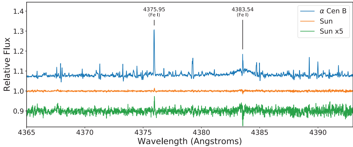
Figure 4. Comparison of the features found on the relative spectra (generated by dividing a high-activity spectrum by a low-activity template) of \alpha Cen B (blue), discussed in Paper I, with features found on the Sun (orange). The strongest narrow peak belongs to the Fe I 4375 Å line, and the broader feature is due to Fe I 4383 Å as indicated. The lower activity level of the Sun means that the features are considerably weaker. Both the orange and green lines show relative spectra from the Sun, but with the values increased by a factor of 5 for the green line, allowing the features to be more easily compared. Note that, for the Sun, only a few features are easily visible compared to the forest of features found on \alpha Cen B, which is due, in part, to residual etaloning noise.
