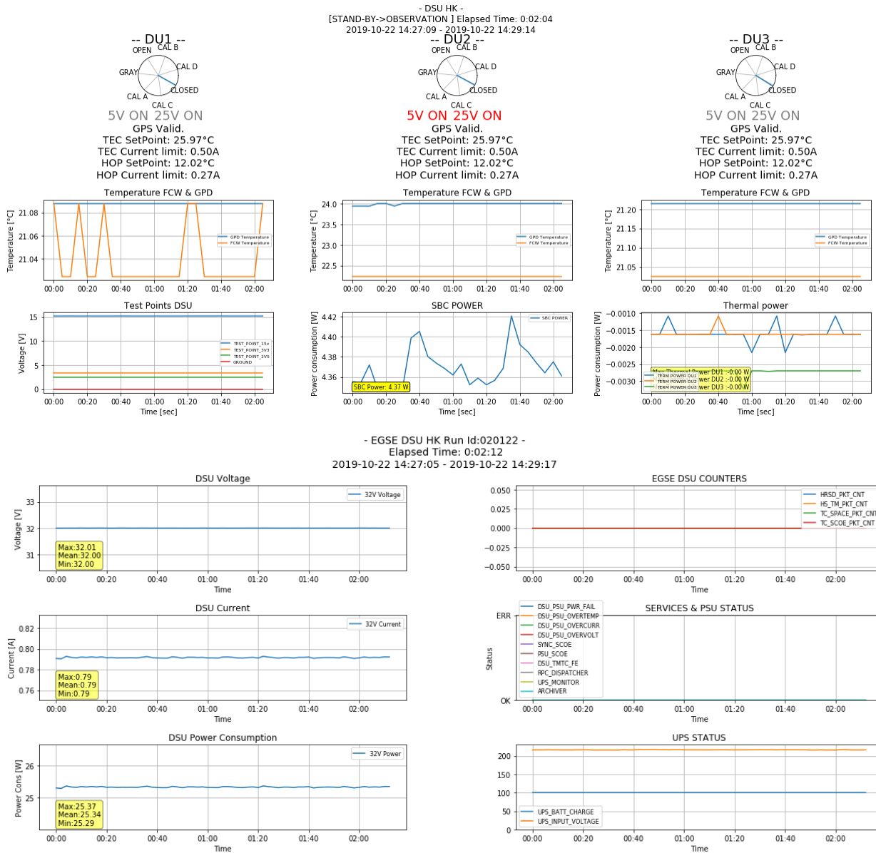
Fig 7-6: Instrument status during the DU Charge Injection Procedure (sec. 7.7). The DSU EM is powered on, the DU FM2 is powered on with both 5 V and 25 V. DU FM1 and DU FM4 are powered off.
