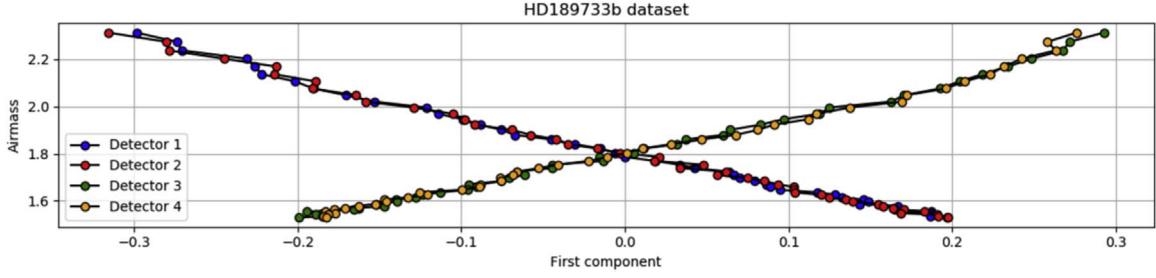
Figure 5. Linear relation between the first component of each detector in the time domain and the recorded airmass for the HD189733b data set.
