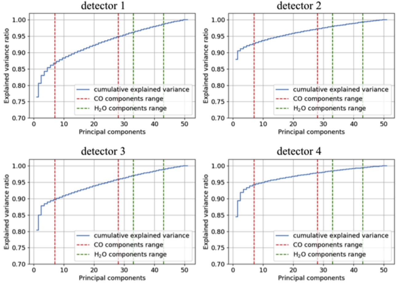
Figure 7. Detectors' variances of the PCA decomposition relative to the HD209458b data set. The first component always carries more than 75% of the information. However, the variance is different for each of the detectors. The red dashed lines highlight the determined component range relative to the CO, while the green dashed lines are relative to the H 2 O.
