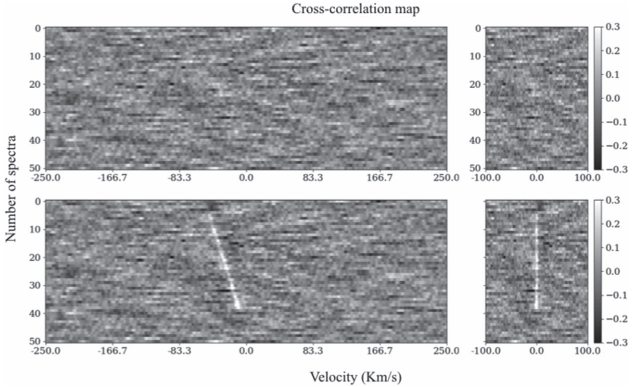
Figure 8. Top left panel: the four CCFs of the four detectors of CRILES of the HD209458b data set summed together. Bottom left panel: same as top but with the model injected. The injection is 1 \times the synthesized model ( R_p/R_\star \sim 10^{-3} ). Top right panel: cross-correlation after changing the reference frame from the Earth to the rest frame of the exoplanet. In this frame the planetary cross-correlation signal is aligned to 0 \text{ km s}^{-1} . Bottom right panel: same as the top right panel, but with the injection. The injected signal is aligned to 0 \text{ km s}^{-1} in the exoplanet’s rest frame.
