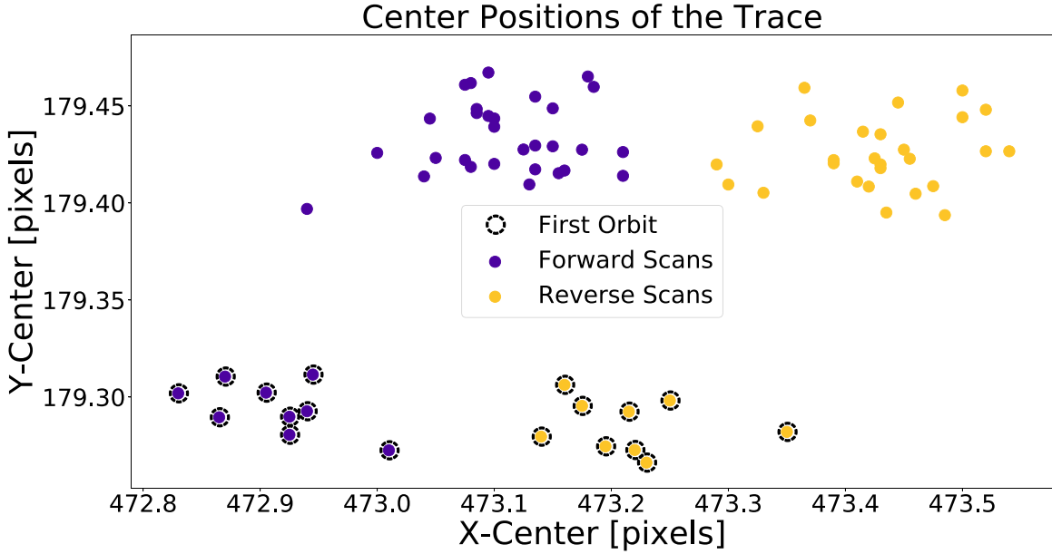
Figure 13. The x - and y -center positions of the trace during all 75 images taken with HST WFC3/UVIS for our WASP-43b eclipse observations. There is a clear separation of \sim \frac{1}{2} pixel in the x -center position between the forward and reverse scanned images; there is also a small but significant shift in the y -center positions during the first orbit, as discussed above.
