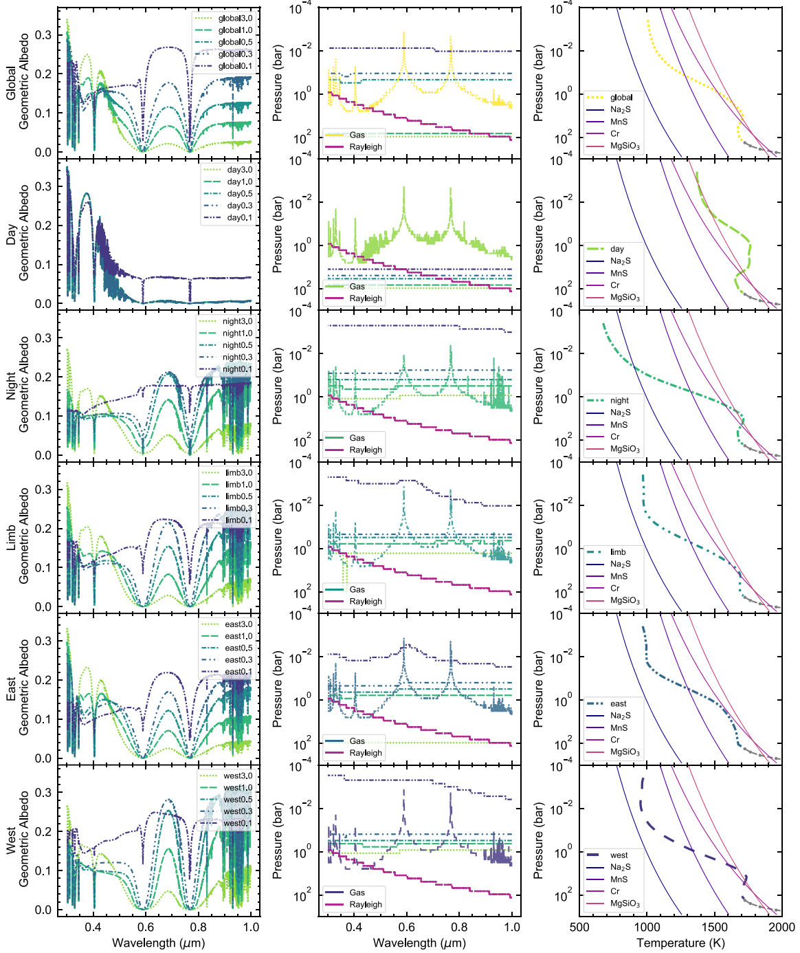
Figure 9. Geometric albedos for the cloudy cases. Each row is a different profile from Kataria et al. (2015). Left: geometric albedo spectrum for each of the five sedimentation efficiencies. Middle: photon attenuation diagram showing the pressure level at which the two-way optical depth in the atmosphere reaches \tau = 0.5 , caused by the gas absorption and cloud or Rayleigh scattering. Line styles and colors for the cloud opacity correspond to their geometric albedo spectrum counterparts. Note the pressure level where clouds contribute changes with f_{\text{sed}} . Right: temperature–pressure profile overlaid on the cloud condensation curves. All profiles readily produce clouds, of which only the most lofted begin to dominate as an opacity source, except for the dayside profile.
