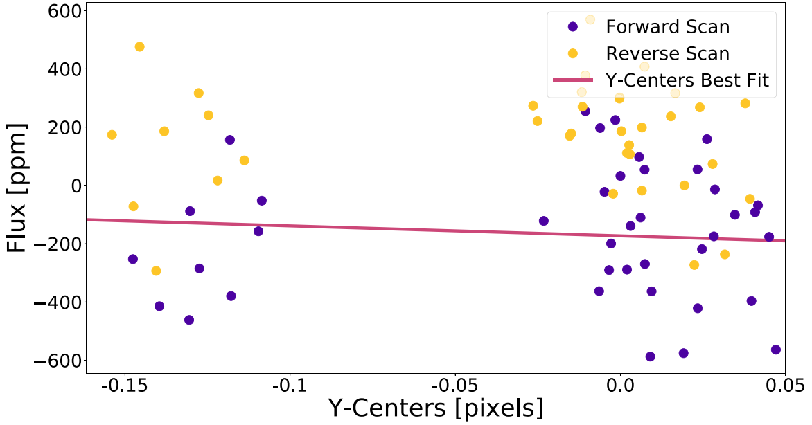
Figure 15. The 2D linear correlation between time + y-center positions and normalized flux for our (AICc) “best” light curve. The slope values are relative to the standard deviation of the flux and pixel coordinates (over the full observation). As before, we coded the forward scan values in violet and reverse scan values in orange.
