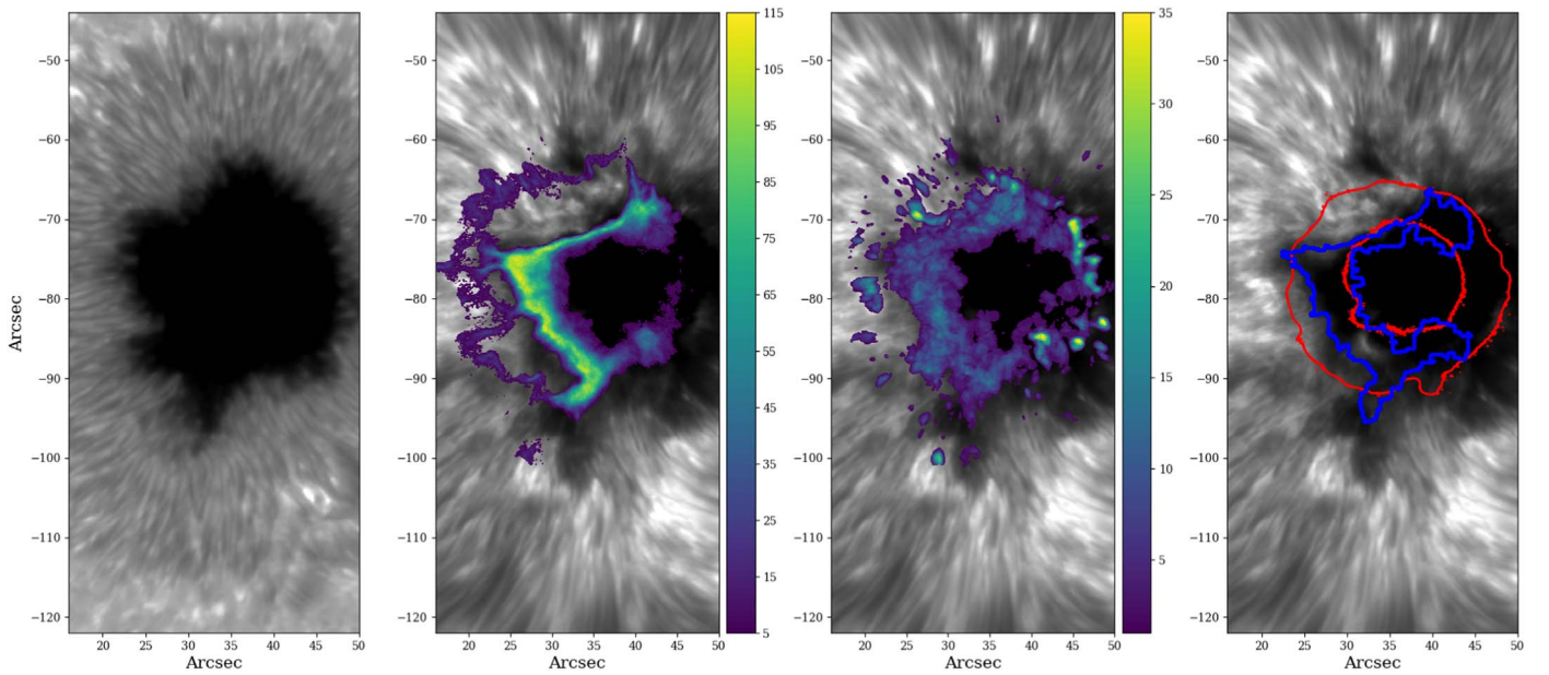
Figure 1. Left: IBIS Ca II red wing image of NOAA AR 12546, acquired at 8542.6 Å (line core +0.5 Å). Middle left: Ca II λ8542 line core image, where the overlaid colored pixels represent the locations where reversals in either Stokes Q/I_c , U/I_c , or V/I_c spectropolarimetric profiles are detected between neighboring frames. The color scale indicates the total number of polarimetric reversals occurring in that pixel throughout the duration of the time series. Middle right: locations and occurrences of pixels that exhibit a change in their Stokes I/I_c magnitude exceeding 3\sigma above their quiescent value. Right: the red lines represent plasma- \beta = 1 isocontours spanning optical depths of ( \sim 450 km) -3 > \log_{10} \tau > -4 ( \sim 625 km). The blue contour represents an outer boundary that encompasses all locations that are deemed “active” pixels (see Section 3.1).
