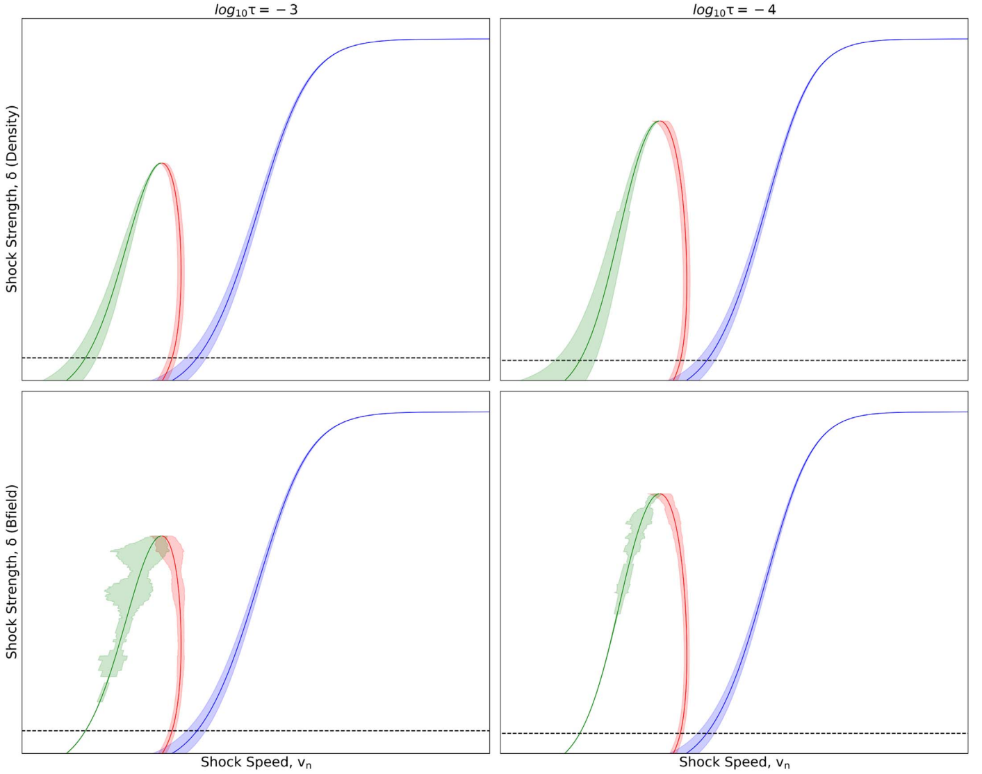
Figure 8. Shock solutions corresponding to the three possible shock normal speeds, slow (green), Alfvén (red), and fast (blue), are displayed for optical depths of \log_{10} \tau = -3 and -4 for a typical shock pixel. The translucent bands represent the average difference between solutions obtained using the input parameters and solutions obtained when the input parameters are perturbed within their error margins. The top panels show how a 10% change in the density ratio alters the solutions, while the bottom panels represent the uncertainties that arise from a change in the magnetic field magnitude. The dashed black line shows the shock strength for the particular pixel.
