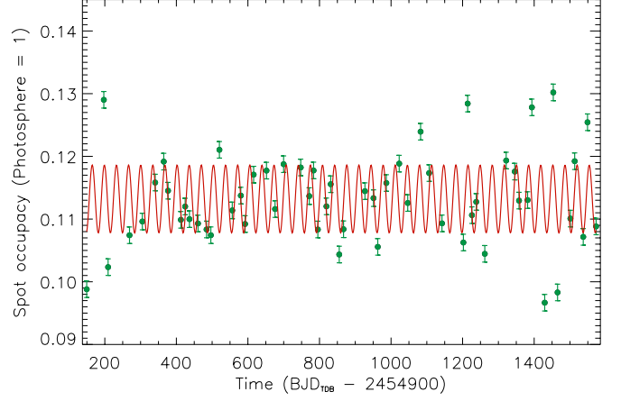
Fig. C.2. The total spotted area on Kepler-30 as derived from the spot modelling of the SAP light curve vs. the time (green dots). A sinusoid with a period of 33.878 days corresponding to the maximum of the GLS periodogram is overplotted (red solid line).
