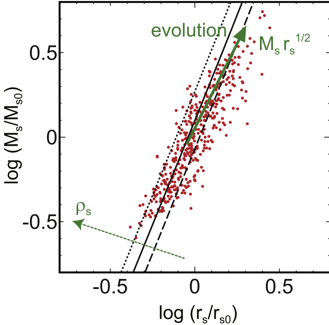
Figure 2. Relation between M_s and r_s at z = 0.25 . The black solid line is calculated for the fiducial c_\Delta . The black dotted and dashed lines are calculated for c_\Delta^U and c_\Delta^K , respectively. Individual clusters generally evolve in the direction of the green solid arrow to which the value M_s r_s^{1/2} increases. The characteristic density \rho_s increases and the cluster formation epoch occurs earlier in the direction of the green dotted arrow. Note that the dotted green arrow is almost (but not perfectly) perpendicular to the three parallel black lines. Red dots are the data points of the MUSIC simulation at z = 0.25 , which are the same as those in Figure 5(a) of Paper I.
