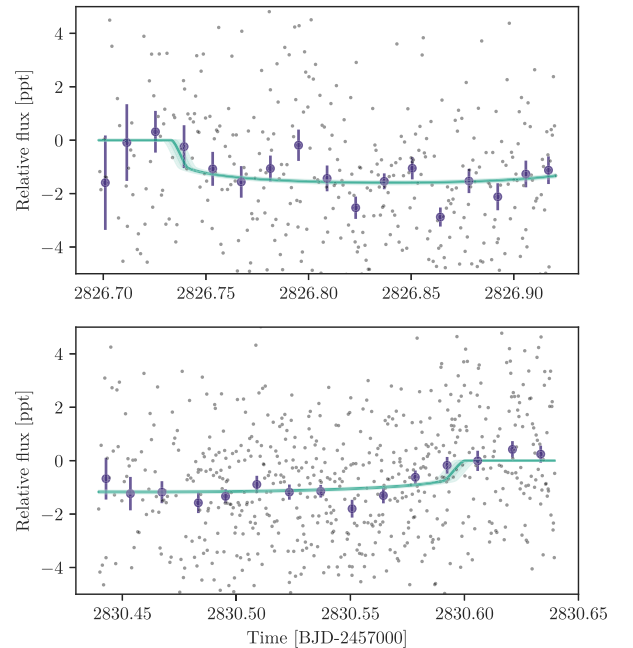
Figure 2. 2022 observations of HIP 9618 using LCOGT 1-m telescopes at CTIO and SAAO, respectively, which confirmed the orbital periods proposed here. Upper: Ingress of HIP 9618 b; Lower: Egress of HIP 9618 c. The grey points show individual points, circles show binned photometry (and errors), and the green line represents the expected transit model given priors from our final combined model.
