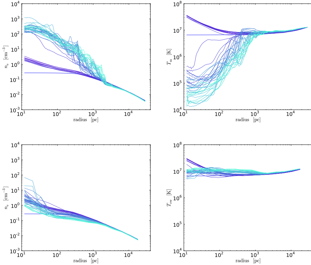
Fig. 20. Accretion with heating, cooling, turbulence ( \text{Ma} \sim 0.35 ), and e_{\text{rot}} = 0.3 : 3D mass- (top) and X-ray emission-weighted ( \propto \mathcal{L} ; bottom) radial profiles of density and temperature (cf. Fig. 7). The profiles show the extended multiphase structure, which is largely concealed in the X-ray band. The X-ray temperature profile is remarkably flat, in contrast to the hot-mode accretion, which has a peaked temperature profile. This is a key observable, which can be thoroughly tested (Wong et al. 2014; Russell et al. 2015), to unveil the evolutionary stage in which the galaxy is residing.
