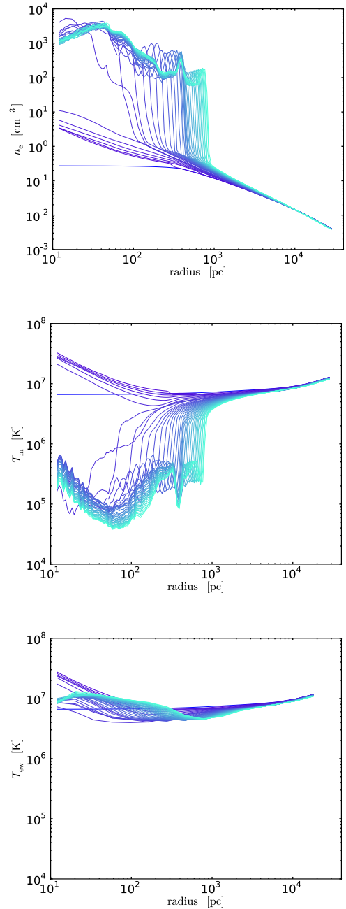
Fig. 7. Accretion with cooling and e_{\text{rot}} = 0.3 : 3D mass- and emission-weighted radial profiles of density and temperature (cf. Fig. 3). The T_{\text{ew}} profile has X-ray threshold of 0.3 \text{ keV} and is computed in larger radial bins (emulating a Chandra observation). The cold thin disk keeps growing via condensation. The X-ray temperature is overall insensitive to the presence of the cold disk.
