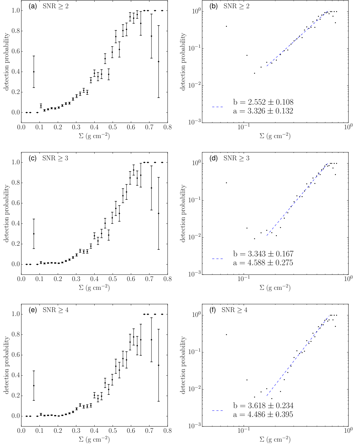
Figure 3. (a): 1.3 mm continuum detection probability P_{1.3\text{mm}} as a function of \Sigma . Here the continuum detection threshold is SNR = 2 with the RMS noise being 0.2 mJy per 2'' beam. The error bars are the square root of the variance of the Bernoulli distribution (see text). (b): The same as panel (a), but in logarithmic scale. The blue dashed line shows a power-law fit over the indicated range of \Sigma . The parameters a and b follow equation 3. (c): Same as (a), but with a detection threshold of SNR = 3. (d): Same as (c), but in logarithmic scale. (e): Same as (a), but with a detection threshold of SNR = 4. (f): Same as (e), but in logarithmic scale.
