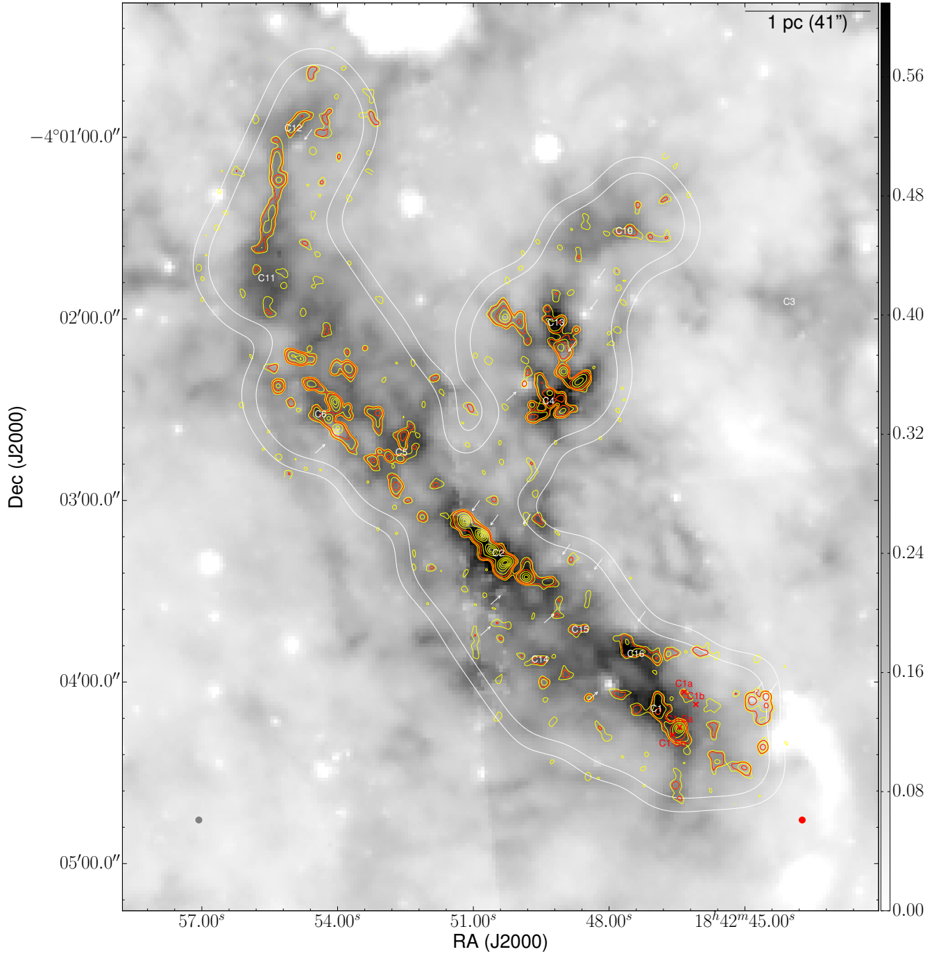
Figure 1. Greyscale: MIREX mass surface density map from BTK14 (scale in \text{g cm}^{-2} ). The angular resolution of the map is shown as the gray filled circle at lower-left. “C1, C2, C3...” label extinction peaks from BTK14. The white arrows point to possible embedded protostars that show as local enhancements in the 8\mu\text{m} image, which produce local “holes” in the MIREX map. Contours: ALMA 1.3 mm continuum mosaic. The contours range from \text{SNR} = 2, 3, 5, 10, 20, 40, 60, \dots with the rms noise at map center \sigma_{\text{center}} \sim 0.2 \text{ mJy beam}^{-1} . The two red contours highlight \text{SNR} = 3 and 10. The synthesized beam is shown as the red filled ellipse at lower-right. The two white enclosing contours show primary-beam responses of 0.3 (outer) and 0.5 (inner).
