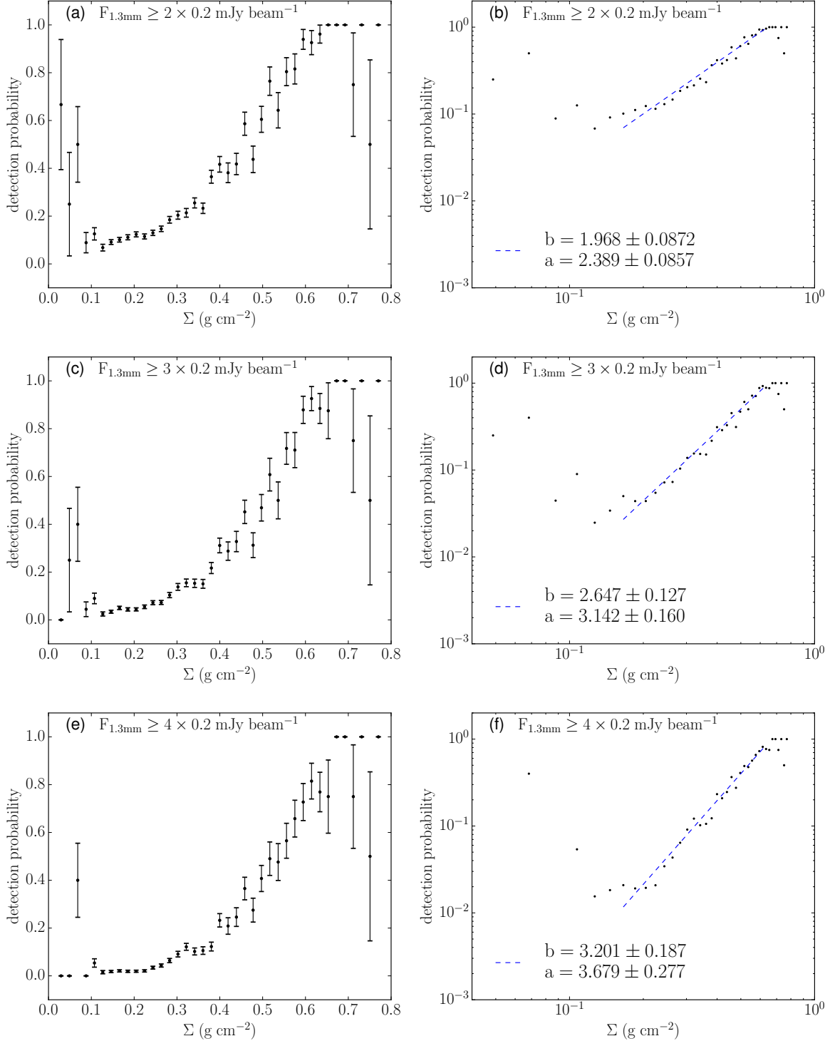
Figure 4. (a): 1.3 mm continuum detection probability P_{1.3\text{mm}} as a function of \Sigma . Here the continuum detection threshold is 2\sigma_{\text{center}} , where \sigma_{\text{center}} ( = 0.2 \text{ mJy per } 2'' \text{ beam} ) is the RMS noise at map center (primary-beam response = 1). The error bars are the square root of the variance of the Bernoulli distribution (see text). (b): The same as panel (a), but in logarithmic scale. The blue dashed line shows a power-law fit over the indicated range of \Sigma . The parameters a and b follow equation 3. (c): Same as (a), but with a detection threshold of 3\sigma_{\text{center}} . (d): Same as (c), but in logarithmic scale. (e): Same as panel (a), but with a detection threshold of 4\sigma_{\text{center}} . (f): Same as panel (e), but in logarithmic scale.
