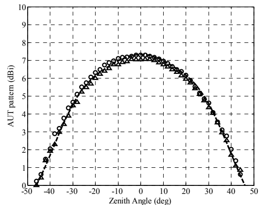
Fig. 5. Co-polar AUT pattern extracted with measured orientation: measurement A (triangles) and B (circles); simulated AUT pattern (dashed line).
