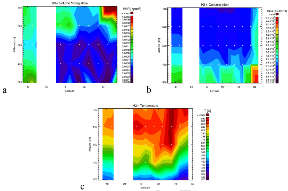
Fig. 5. \text{H}_3^+ VMR (a), concentration (b) and temperature (c) maps obtained from the analysis of the limb data in Sys III. White points in the figures indicate the latitude and altitude values of each bin of the considered grid. The white area, instead, indicates a region where no data are available in the considered dataset.
