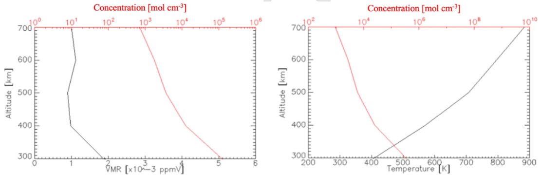
Fig. 6. Correlation of VMR and \text{H}_3^+ concentration (image on the left) and between temperature and \text{H}_3^+ concentration (image on the right), retrieved with our inversion code. The scale for VMR and temperature are shown in the lower x-axis, while in the upper one there are the values for concentration in log-scale (in red). Data at all available latitudes were averaged. (For interpretation of the references to colour in this figure legend, the reader is referred to the web version of this article.)
