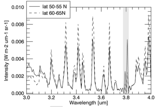
Fig. 3. Averaged spectrum of \text{H}_3^+ emission at 50\text{--}55^\circ N (solid line) and 60\text{--}65^\circ N (dashed line), from JIRAM session 160,826–175,419, obtained considering all the pixels with tangent altitudes in the range 0–1100 km above the 1-bar level. The most intense \text{H}_3^+ bands are observed in both spectra at 3\text{--}3.8\ \mu\text{m} , although their intensities are on average lower at mid-latitudes. The shaded area identifies an instrumental artefact.
