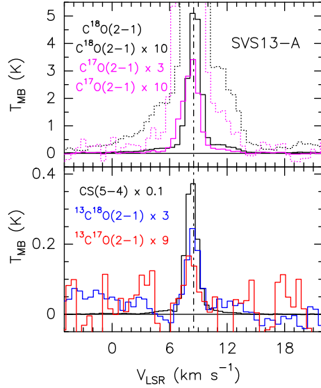
Figure 7. Emission detected towards SVS13-A with the IRAM 30 m in the 1 mm spectral window with HPBW's consistent with that used for the observations of \text{NO } ^2\Pi_{1/2} J = 5/2-3/2 . Upper panel: \text{C}^{18}\text{O}(2-1) and \text{C}^{17}\text{O}(2-1) lines (in T_{\text{mb}} scale; also increased by different factors to show the outflow wings; dotted histograms). The vertical dashed line indicates the ambient LSR velocity ( +8.6 \text{ km s}^{-1} ; Chen, Launhardt & Henning 2009). Bottom panel: ^{13}\text{C}^{18}\text{O}(2-1) , ^{13}\text{C}^{17}\text{O}(2-1) , and \text{CS}(5-4) profiles, scaled to be drawn on the same scale.
