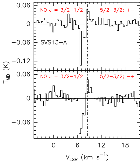
Figure 4. Upper panel: spectral signatures due to the \text{NO } ^2\Pi_{1/2} J = 3/2-1/2 spectral pattern (black histogram; see Table 1; in T_{\text{mb}} scale after correction for beam dilution, see the text) observed towards SVS13-A with the IRAM 30-m antenna. The spectrum is centred at the frequency of the hyperfine component F_{\text{ul}} = 5/2-3/2 ; p_{\text{ul}} = + \rightarrow - (150 546.52 MHz). The vertical dashed line indicates the ambient LSR velocity ( +8.6 \text{ km s}^{-1} , Chen, Launhardt & Henning 2009). The absorption is due to emission in the OFF position, observed in wobbler mode with a throw of 180 arcsec (see Section 3). Bottom panel: same as for the upper panel for the hyperfine component F_{\text{ul}} = 5/2-3/2 ; p_{\text{ul}} = - \rightarrow + (150 176.48 MHz).
