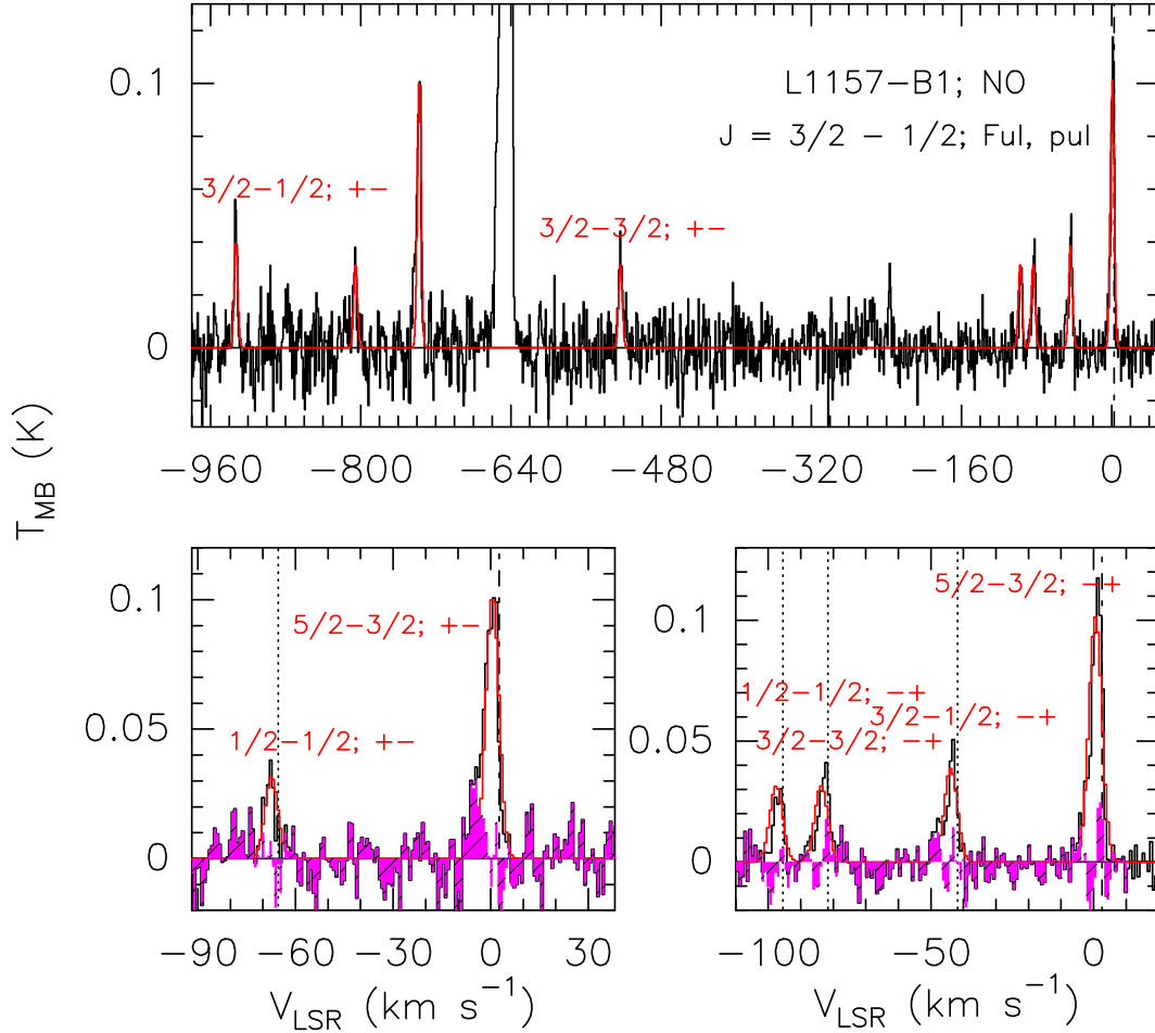
Figure 6. Upper panel: emission due to the NO ^2\Pi_{1/2} J = 3/2-1/2 spectral pattern (black histogram; see Table 1; in T_{\text{mb}} scale after correction for beam dilution, see the text) observed towards L1157-B1 with the IRAM 30-m antenna. The red line shows the best fit obtained with the GILDAS-CLASS package using the simultaneous fit of all the hyperfine components (see Table 2). For sake of clarity, the hyperfine components that are not indicated in the upper panel are labelled in the zoom-in in the lower panels. The spectrum is centred at the frequency of the hyperfine component F_{\text{ul}} = 5/2-3/2 ; p_{\text{ul}} = - \rightarrow + (150 176.48 MHz). The vertical dashed line indicates the ambient LSR velocity ( +2.6 \text{ km s}^{-1} ; Bachiller et al. 2001). Bottom-right panel: zoom-in of the upper panel. Dotted lines point the hyperfine components falling in that portion of the spectrum. The purple filled histogram shows the residual after Gaussian fit (red) of the NO emission (black). Bottom-left panel: zoom-in of the upper panel, after having centred the spectrum at the frequency of the hyperfine component F_{\text{ul}} = 5/2-3/2 ; p_{\text{ul}} = + \rightarrow - (150 546.52 MHz).
