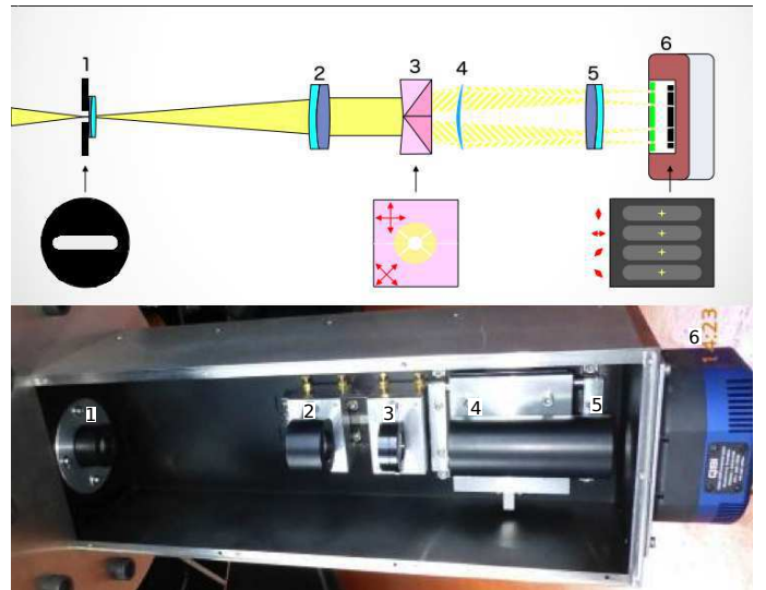
Figure 2. Scheme and photograph of the ToPol instrument. 1: Field stop followed by the field lens. 2: Collimator lens. 3: Wedged double Wollaston. 4 and 5: Camera optics. 6: QSI632 CCD camera
