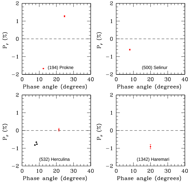
Figure 9. Phase - polarization data for asteroids (194) Prokne, (500) Selinur, (532) Herculina and (1342) Haremar. Triangles: data available in the literature for (532) Herculina. Full symbols: new CAPS data.
