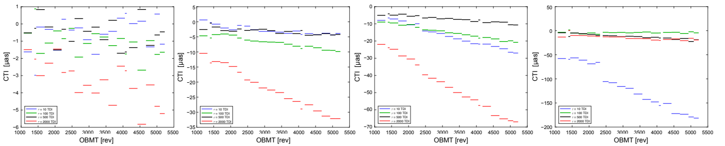
Fig. A.8. CTI calibration averaged over CCDs and FoVs. From left to right : WC0a ( G \leq 11 ), WC0b ( 11 \leq G \leq 13 ), WC1 ( 13 \leq G \leq 16 ), and WC2 ( 16 \leq G ). Each diagram shows the development of the coefficients of \exp(-\Delta t/\tau) , where \Delta t is the time since last charge injection, for the time constants \tau indicated in the legends.
