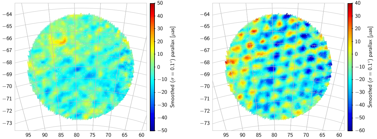
Fig. 14. Smoothed maps of parallaxes in the LMC area, visualising small-scale systematics (the “checkered pattern”) in Gaia EDR3 and DR2. Left : smoothed parallaxes in EDR3 for sources in the magnitude range G = 16 –18 (median G = 17.4 ), kinematically selected as probable members of the system (see Appendix B in Lindegren et al. 2021 for details). Right : smoothed parallaxes in DR2 for the same sample of sources. Both maps were smoothed using a Gaussian kernel with standard deviation 0.1^\circ . While the sample includes about 730 000 sources within 5^\circ radius of the adopted centre, only smoothed points within a radius of 4.5^\circ are shown to avoid unwanted edge effects. Comparison between the two diagrams is facilitated by the use of the same colour scale, only shifted by 10 \mu\text{as} to compensate for the mean difference in parallax between DR2 and EDR3.
