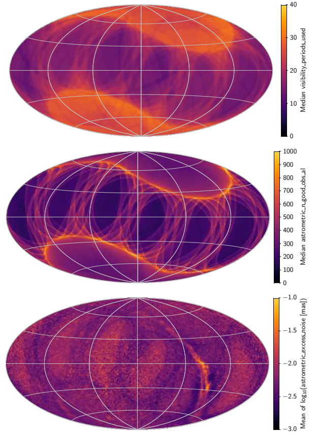
Fig. 9. Selected observation statistics at G \approx 15 for sources with a five-parameter solution in EDR3. These statistics are main factors governing the formal uncertainties of the astrometric data. Top : number of visibility periods used. Middle : number of good CCD observations AL. (The number of FoV transits used in the solution looks very similar, only with a factor nine smaller numbers.) Bottom : mean of \log_{10}[\max(0.001, \text{astrometric\_excess\_noise})] .
