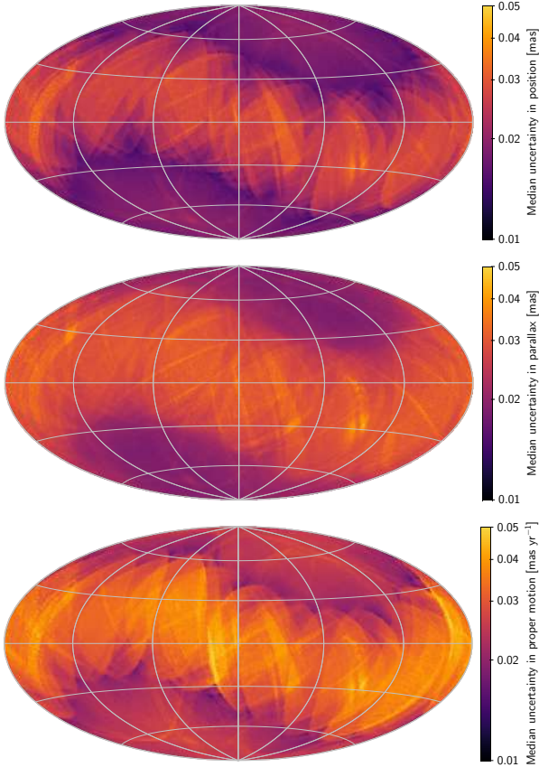
Fig. 8. Formal uncertainties at G \approx 15 for sources with a five-parameter solution in EDR3. Top : semi-major axis of the error ellipse in position at epoch J2016.0. Middle : standard deviation in parallax. Bottom : semi-major axis of the error ellipse in proper motion. These and all other full-sky maps in the paper except Fig. 12 use a Hammer–Aitoff projection in equatorial (ICRS) coordinates with \alpha = \delta = 0 at the centre, north up, and \alpha increasing from right to left.
