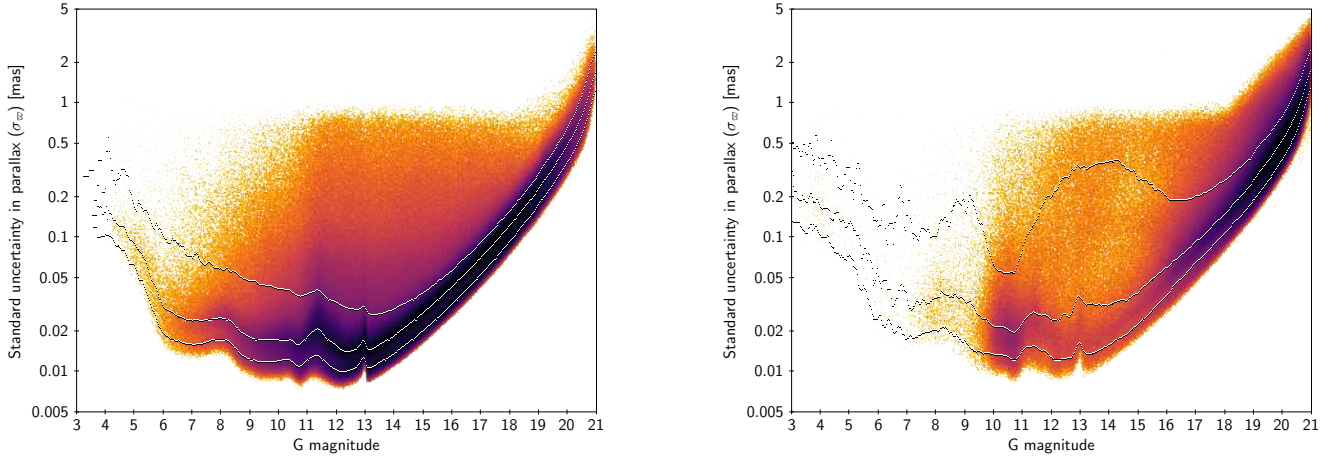
Fig. 7. Uncertainty in parallax versus magnitude. Left: five-parameter solutions. Right: six-parameter solutions. The plots include all sources with G < 11.5 and a geometrically decreasing random fraction of the fainter sources, so as to give a roughly constant number of sources per magnitude interval. The colour scale from yellow to black indicates an increasing density of data points in the diagram. The curves show the 10th, 50th, and 90th percentiles of the distribution at a given magnitude.
