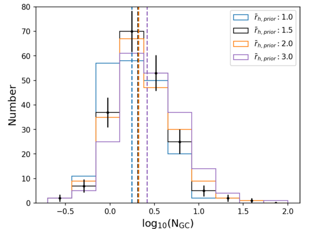
Figure D1. The distribution of N_{GC} estimates for our sample of galaxies as a function of the mean of the prior on the GC half-number radius, \bar{r}_{h, \text{prior}} , in units of galaxy half-light radius. Also shown are the median values (dashed lines). Our value of \bar{r}_{h, \text{prior}} = 1.5r_e is adopted from the literature and Poisson error bars are shown for this value.
