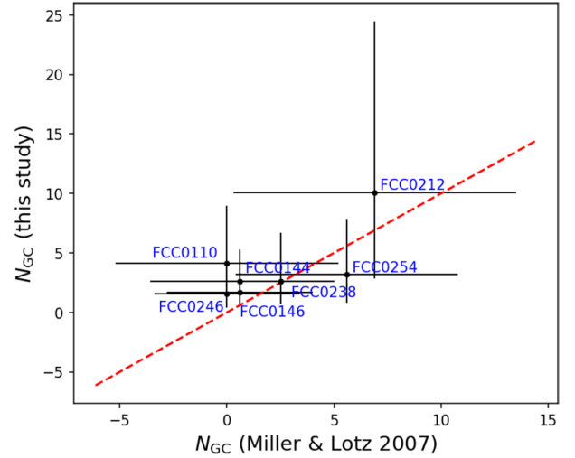
Figure C1. Comparison of GC number counts. The black points are median values from the MCMC posterior. The error bars span the range of 1\sigma . The red dashed line is the one-to-one relation. A chi-square test (accounting for the errors) shows that the null hypothesis that the measurements are consistent with the one-to-one relation cannot be rejected with confidence greater than around 4 per cent.
