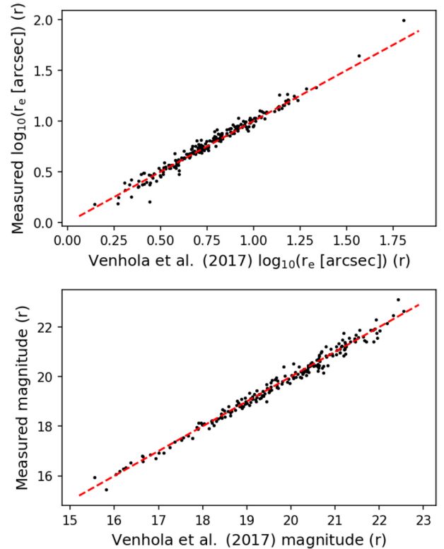
Figure A1. Our galaxy measurements (IMFIT) versus those of V17 (GALFIT). Red dashed line: The one-to-one relation. The RMS of the residuals are 0.18 mag and 0.04 dex in r_{\text{e}} .
