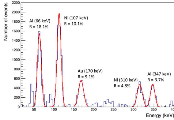
Figure 19. Spectrum with a pure Hydrogen filling of the target, as seen from one Ce:LaBr 3 detector, equipped with a Hamamatsu S13361-AS SiPM array. Background has been subtracted.
