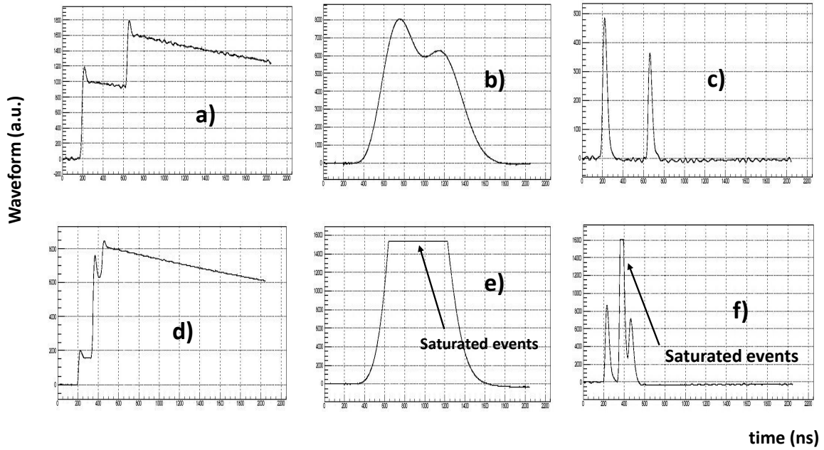
Figure 20. (a), (d) pre-amplified signals for a HPGe GEM-S detector. (b), (c) amplified signals with an Ortec 672 spectroscopy amplifier. (e), (f) amplified signals with a fast Ortec 579 shaping module.
