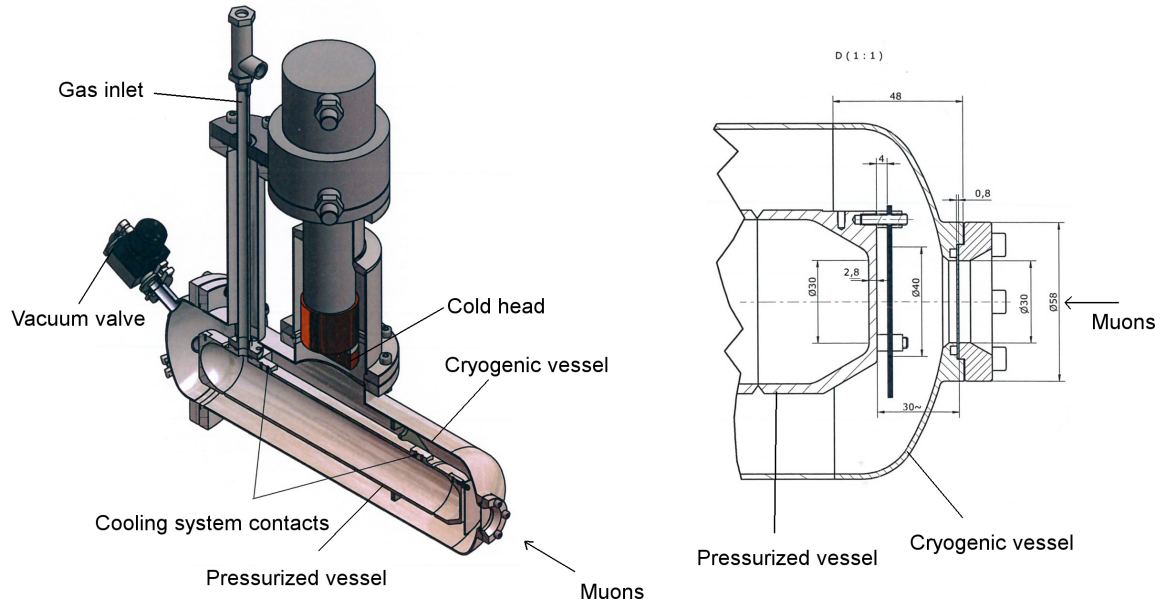
Figure 4. The target design. Left panel: the double volume shell needed for thermal insulation is clearly visible: the whole is realized in Aluminium alloy. Right panel: the details of the muon beam entrance window. Beam goes from right to left.
