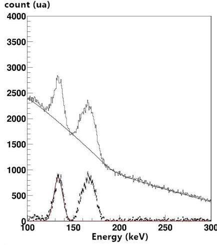
Figure 17. Measured delayed spectrum with a H 2 +O 2 (0,3%) gas mixture in the target. Muonic Oxygen X-rays: 133 keV K_\alpha , 158 keV K_\beta and 167 keV K_\gamma lines, with background (top) and background subtracted (bottom). The energy resolution for the 133 keV line is 8.5%.
