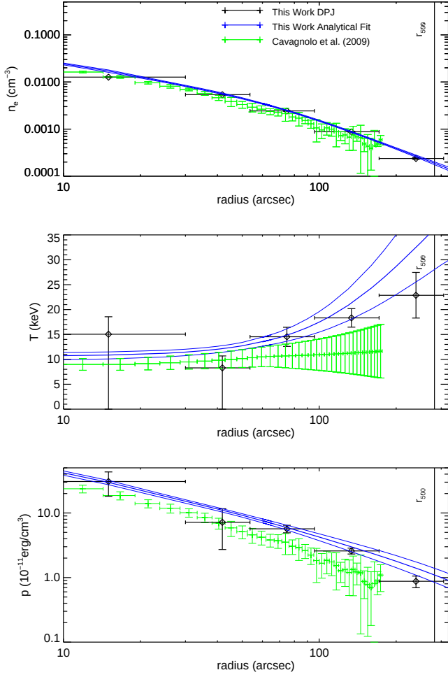
Figure A26. MACS J1206.2-0847. Both our density and temperature profiles are in reasonable agreement with the ACCEPT results, and our smooth parametric fits indicate a drop in temperature near the core at a significance of 2.3\sigma . Donahue et al. (2014) obtained temperature profiles using X-ray spectroscopy from XMM-Newton and Chandra . The Chandra profile has a large temperature peak in the center (15 keV), dropping to a nearly isothermal profile of 10 keV to the maximum radius probed by the data (1000 kpc or 180'' ). The XMM-Newton profile, on the other hand, has a cool core of \sim 7 keV, which increases with radius to 10 keV before dropping to 5 keV in the outskirts. Our analysis is consistent with these results at intermediate radii, but we find an approximately isothermal profile into the core and a slight temperature increase at large radius. Several studies, using X-ray, optical, and/or lensing data have found this cluster to be relaxed (Gilmour et al. 2009; Mann & Ebeling 2012; Umetsu et al. 2012).
