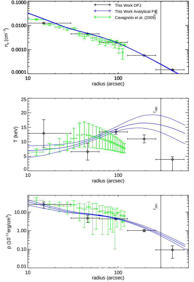
Figure A25. MACS J0417.5-1154. From our smooth parametric fits, we detect a cool-core at a significance of 3.3\sigma , and both our density and temperature profiles are reasonably consistent with the ACCEPT results. Mann & Ebeling (2012) identified this cluster as a primary candidate for a binary, head-on collision type merger: the X-ray core aligns with one of two optical cores, but the X-ray emission bleeds into the outskirts and meets with the second of the optical cores.
