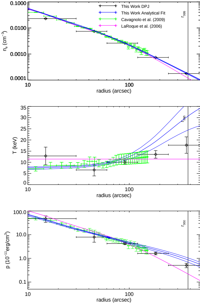
Figure A10. Abell 1835. In the regions of overlap, both our density and temperature profile fits are in excellent agreement with the ACCEPT results, and our smooth parametric fits show modest evidence for a temperature drop in the core ( 2.8\sigma ). In the outer regions of the cluster, our temperature and pressure profiles are somewhat higher compared to the joint X-ray/SZ study presented in LaRoque et al. (2006), although this may be related to the isothermal assumption used in that analysis. In contrast to the rising temperature at large radius seen in our fits, Ichikawa et al. (2013) found that the temperature slowly decreases from 8 keV in the inner region to around 2 keV near the virial radius using Suzaku X-ray spectroscopy. Based on Chandra observations, Bonamente et al. (2013) also found a similarly large drop in temperature towards the cluster outskirts. We note that many studies have found this cluster to be spherically symmetric without any significant substructure (Korngut et al. 2011; Ichikawa et al. 2013), although Morandi et al. (2012) find that the cluster is elongated in the line of sight, which may be the cause of the apparent temperature increase at large radius in our fits. In addition, Baldi et al. (2007) found that the temperature drops by a factor of 2 in core region relative to the peak, in contrast to both our results and the ACCEPT results.
