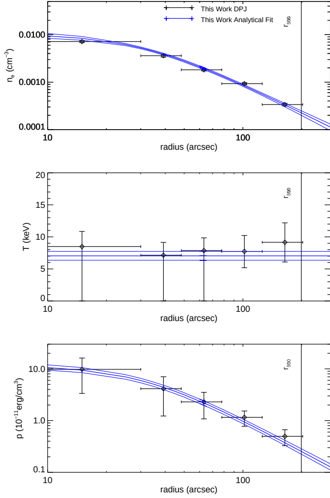
Figure A24. MACS J0451.9+0006. Maughan et al. (2008) used Chandra spectroscopy to obtain an isothermal temperature of \sim 5.6 keV at radii < r_{500} (4.8 keV if the central region is excised). This is somewhat lower, but reasonably consistent with, the approximately isothermal profile found in our analysis. Mann & Ebeling (2012) found this cluster to have highly irregular morphology, but it was not classified as an extreme or active merger due to its small BCG-Xray peak and BCG-Xray center separations.
