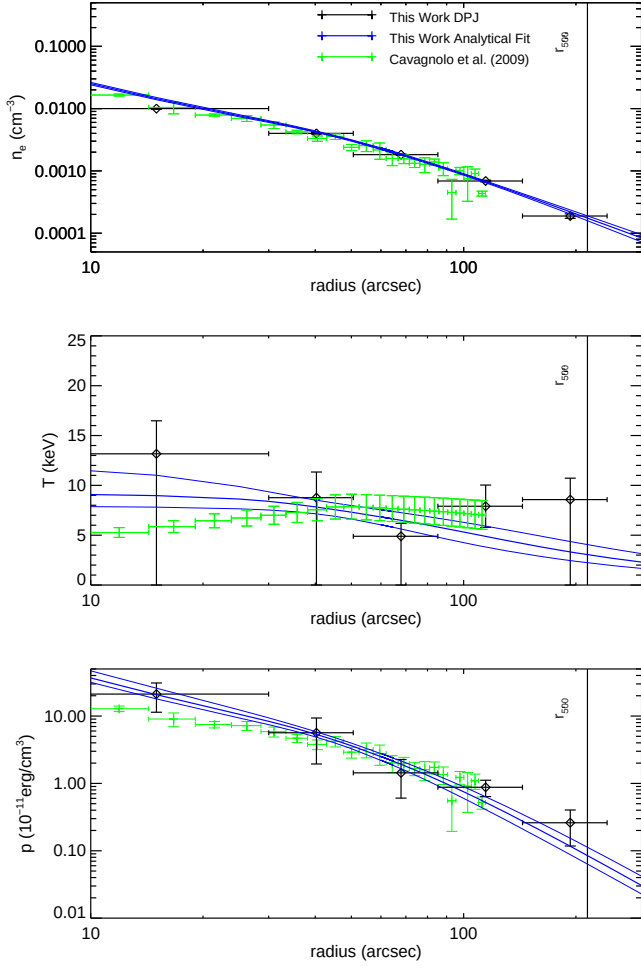
Figure A22. MACS J1720.3+3536. Our data indicate a decrease in the temperature in the outskirts at a significance of 6.5\sigma and are generally in good agreement with the ACCEPT results. Donahue et al. (2014) obtained temperature profiles using X-ray spectroscopy from XMM-Newton and Chandra , and found that the temperature profiles from the two instrument have different shapes. Both have a central temperature of \sim 3.5 keV. XMM-Newton jumps to 10 keV then slowly decreases down to \sim 2 keV at 900 kpc ( 170'' ), consistent with our results outside of the core region. In contrast, Chandra slowly reaches 10 keV but then drops down to temperatures close to zero around 400kpc ( 70'' ). Essentially, the outer temperature slope is steeper for Chandra , but the inner temperature slope is steeper for XMM-Newton . Maughan et al. (2008) used Chandra spectroscopy to obtain an isothermal temperature of \sim 6.1 keV for radii < r_{500} (7.8 keV if the core region is excised), broadly consistent with our results.
