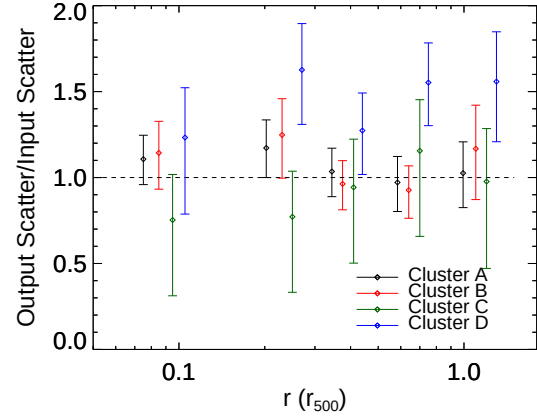
Figure 6. Output intrinsic temperature scatters with errors for the four mock cluster samples. Since the input scatter used for Cluster C was different from the other three test clusters, the recovered scatters are plotted relative to the input values.
