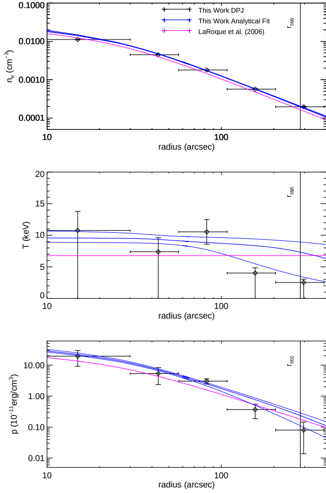
Figure A12. Abell 611. We find a relatively flat temperature profile, in good agreement with the spectroscopic X-ray measurements from Bonamente et al. (2006) . In addition, Donnarumma et al. (2011) performed an analysis of this cluster using X-ray data from Chandra and lensing results from Hubble . Unlike our analysis, they identify it as a cool-core cluster. However, their overall temperature profile is in good agreement with our results. They found a central temperature of 6 keV, a peak of 8 keV at 100 kpc (20''), and a slow drop in temperature to 5 keV at 600 kpc (150''). There is a known error in the ACCEPT results for this cluster, and so they are not included in the plot.
