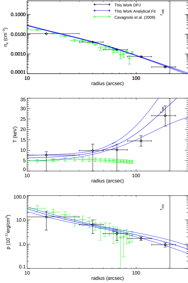
Figure A20. MACS J0429.6-0253. Our analysis indicates a temperature increase at large radius that is not seen in the ACCEPT results, and our smooth parametric fits indicate a drop in temperature towards the core at a significance of \sim 2\sigma . Donahue et al. (2014) found temperature profiles using X-ray spectroscopy from XMM-Newton and Chandra , with the temperature profile showing a central temperature of 4 keV and a peak of 9 keV at 200 kpc (40''), roughly consistent with our results over the same range.
