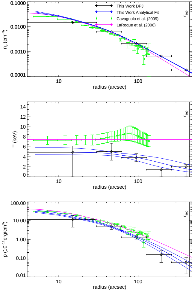
Figure A6. Abell 2261. Based on our smooth parametric fit, we detect a temperature drop in the outskirts at a significance of 5.5\sigma . Comparing to X-ray spectroscopy, ACCEPT (Cavagnolo et al. 2009) shows a slight temperature drop in the center which is not detected in our analysis, along with an overall temperature somewhat higher than our results. In good agreement with the ACCEPT results, Baldi et al. (2007) found a slight cool-core, with a central temperature of 7.7 \pm 0.4 keV and peak of 9.0 \pm 0.4 keV. Bonamente et al. (2006), also using X-ray spectroscopy, similarly found a temperature profile in good agreement with the ACCEPT results. Coe et al. (2012) found a density profile slope that is shallower than the usual slope at small radii for cool-core clusters, thus they defined it as a “borderline” relaxed and cool core cluster (our analysis classifies it as a CC non-disturbed cluster). Finally, Abell 2261 is a CLASH cluster (Postman et al. 2012), and Coe et al. (2012) used the CLASH data to obtain a detailed mass measurement, deducing that the DM halo is elongated along the line of sight.
