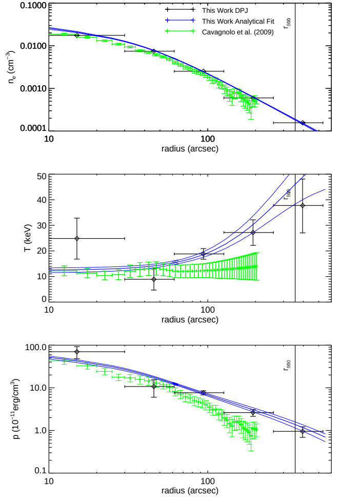
Figure A15. Abell S1063. As with MACSJ1931.8-2634, our results are fairly consistent with the ACCEPT results other than a slight increase in temperature at large radius. Gómez et al. (2012) found evidence of merging through both X-ray and optical observations, with an elongated X-ray emission feature in the same direction as two regions of high galaxy density. They found high cluster temperatures of 12-17 keV from the center to \sim 800 kpc (160"), in reasonable agreement with our results over the same range.
