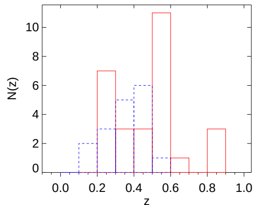
Figure 1. Cluster redshift distribution of the sample. The red solid line indicates NCC clusters while the blue dotted line indicates CC clusters.
