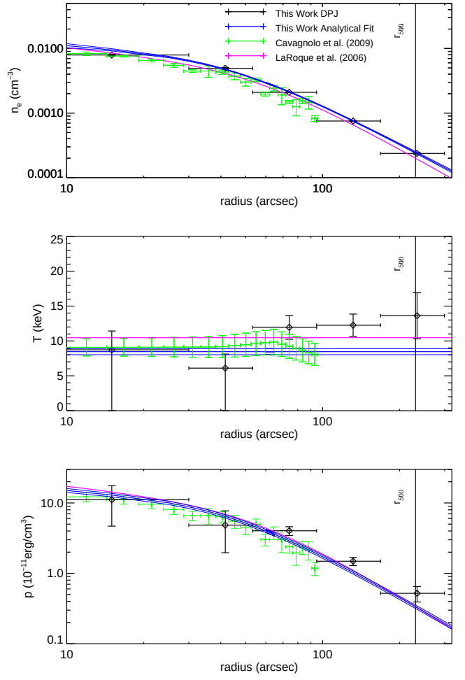
Figure A33. MACS J0018.5+1626. The profiles we obtain for this cluster are in excellent agreement with the ACCEPT and LaRoque et al. (2006) results. Several studies have found this cluster to be relaxed (e.g., Kotov & Vikhlinin 2005), however, Solovyeva et al. (2007) found evidence for it to be undergoing a merger near the center of the cluster using XMM-Newton observations. They also found a temperature profile out to r_{200} , showing a clear decrease in the outskirts, to 4 keV, which does not match the approximately isothermal profile found in our analysis. Worral & Birkinshaw (2003) found no evidence of a cool core, but they did find evidence for a merger in the center of the cluster due to the non-spherical X-ray shape in that region. Overall, they find an isothermal temperature of \sim 9.13 keV, consistent with our results.
