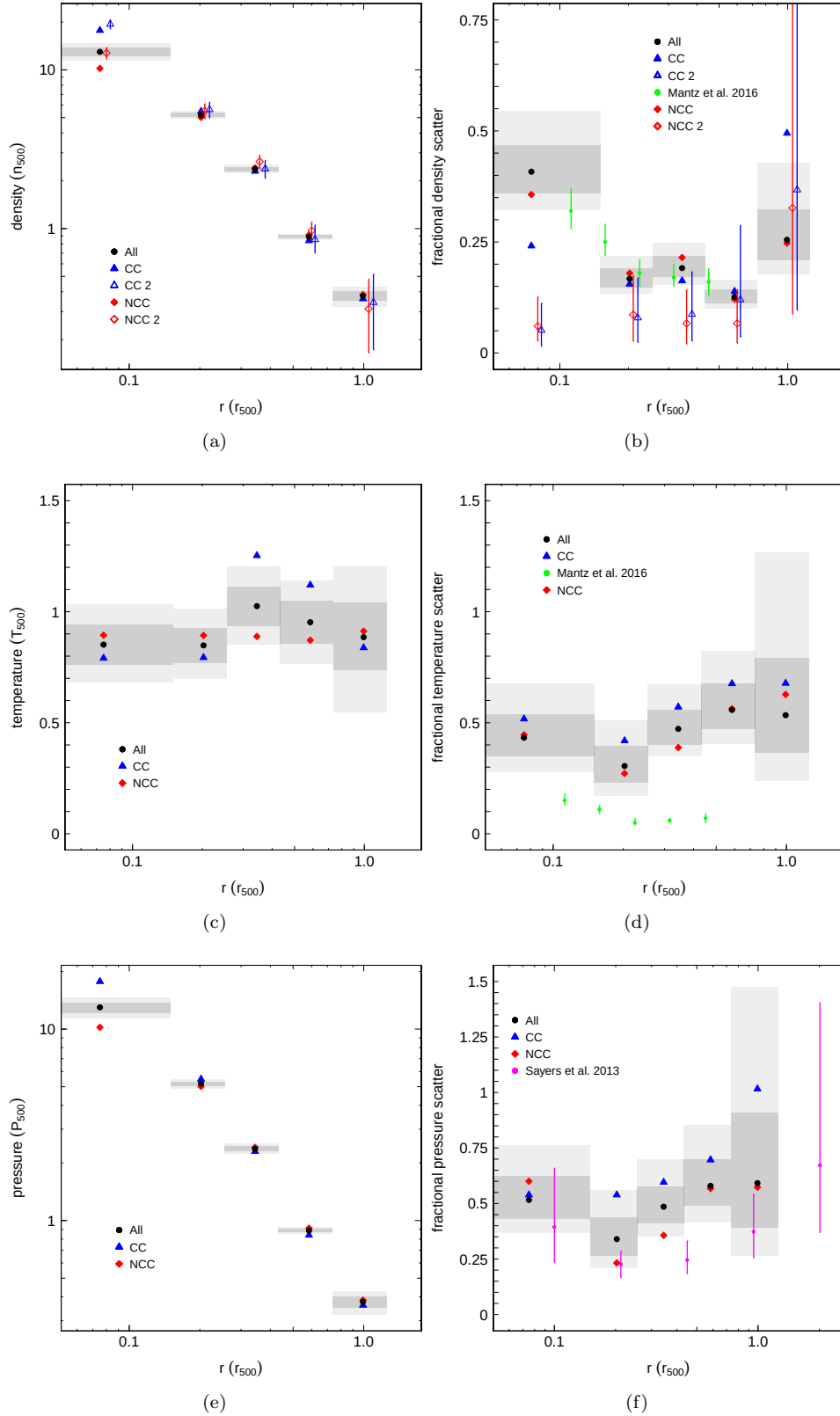
Figure 7. The left column shows the mean density (a), temperature (c), and pressure (e) profiles for the full sample, CC, and NCC subsets (scaled according to the self-similar values given in Sec. 4.2.1). The solid points correspond to the results obtained from the meta-analysis of Sec. 4.2.2, and the hollow points correspond to the results obtained from full likelihood method of Sec. 4.2.1. The gray shaded regions are the 68% and 95% confidence regions for the meta-analysis of the full sample. The confidence regions for the CC and NCC subsets are slightly larger in size, and have been omitted for clarity. The right column shows the fractional intrinsic scatter about the mean profiles. The green points are from Mantz et al. (2016), while the magenta points are from Sayers et al. (2013b).
