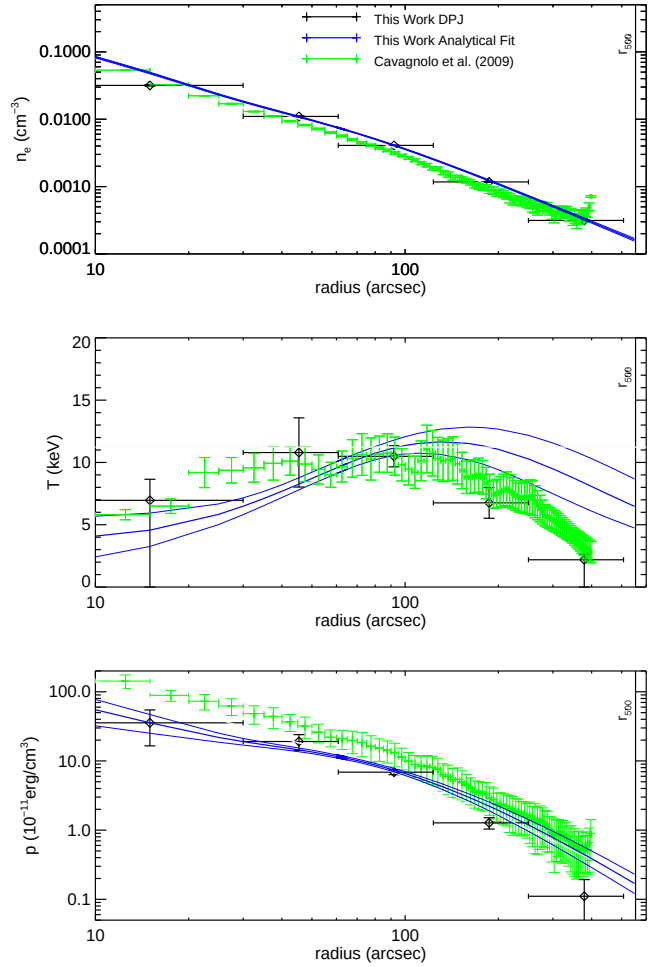
Figure A1. Abell 2204. Our smooth parametric profile fit detects a cool core at a significance of 3.8\sigma , and the temperature drop in the outskirts is detected at a significance 5\sigma . In general, both our smooth parametric fits and deprojections of both the density and temperature are in good agreement with ACCEPT and other previous X-ray results (e.g., Sanders et al. 2005 and Reiprich et al. 2009). Although we classify this cluster as relaxed, Sanders et al. (2005), using X-ray data, found a complicated core consisting of several cold fronts that may be attributed to the cluster recovering from a merger. Gu et al. (2009) also found such temperature substructures, and speculate that they may be caused by AGN. Sanders et al. (2009), again using X-ray data, found dips in the surface brightness that may be caused by radio bubble formation in the core of the cluster. Reiprich et al. (2009) used Suzaku X-ray measurements to probe the cluster out to large radii, approximately 12' , where the temperature was found to be 4 keV. This is in good agreement with both the extrapolation of our smooth parametric profile and with the predictions from the hydrodynamical simulations of Roncarelli et al. (2006).
