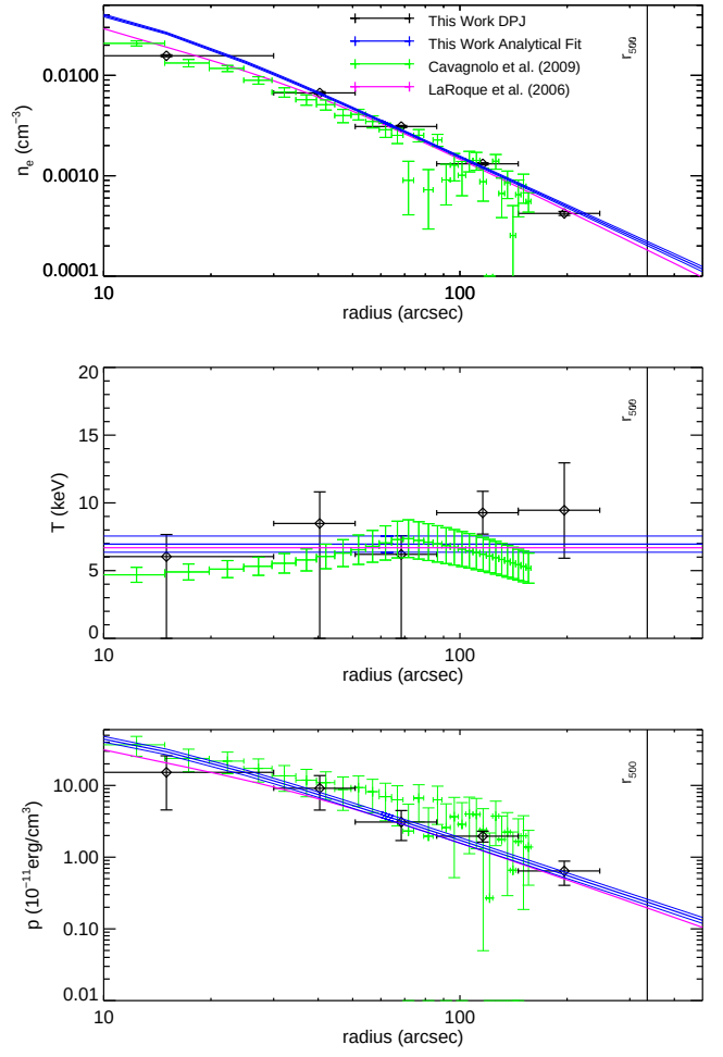
Figure A9. RX J2129.6+005. Both our density and temperature profiles are in fairly good agreement with the ACCEPT results. There is some deviation between our density deprojection and the smooth parametric fit near the center, which may suggest that the single-beta profile is not fully sufficient in describing the data. This is one of the few clusters in the sample where the fits do not reach r_{500} , due to the poor quality of the X-ray data. Landry et al. (2013) used Chandra observations to identify this as a relaxed cluster based on the centroid shift. Furthermore, unlike the relatively isothermal temperature profile found in both our analysis and the ACCEPT analysis, they found a central temperature of 4 keV, a peak temperature of 8 keV near 90'' and a decrease in temperature back to 4 keV in the outskirts (near 240'' ).
