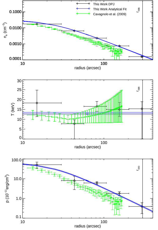
Figure A21. MACS J2211.7-0349. Our densities and pressures are systematically and significantly higher than those found in the ACCEPT study. Due to the lack of independent results for this cluster, it is not possible to determine which analysis may be in error.
