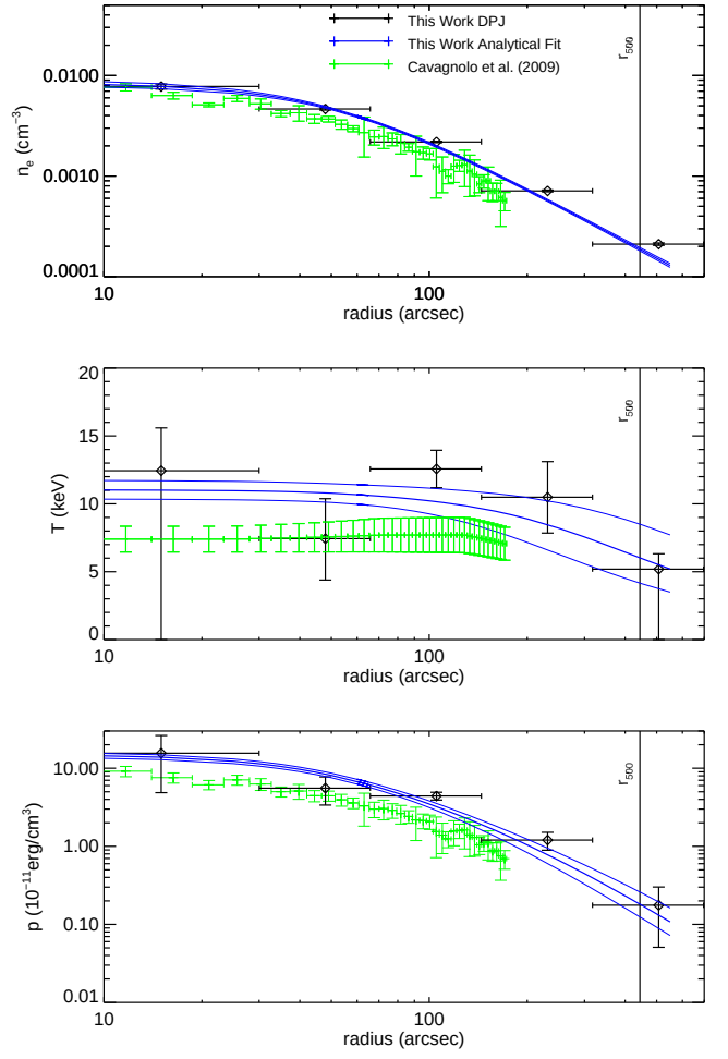
Figure A3. Abell 209. In our smooth parametric fit, we detect a temperature drop in the outskirts at a significance of 3.5\sigma . Although our temperature is somewhat higher than the ACCEPT results, we note that Mercurio et al. (2003) found a temperature of 10.2^{+1.4}_{-1.2} keV using X-ray spectroscopy within 180'' , in good agreement with our results. We classify this cluster as non-disturbed, but Mercurio et al. (2003) found a slightly elongated structure in the X-ray map arising from two X-ray peaks. Adding to the evidence that this cluster is at least somewhat disturbed, Paulin-Henriksson et al. (2007) also found elongation in the mass distribution through weak lensing.
