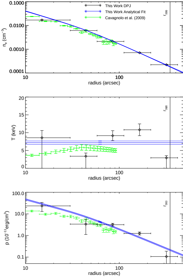
Figure A2. Abell 383. Our density and temperature profiles are reasonably consistent with the ACCEPT results at overlapping radii, although our isothermal smooth parametric fit to the temperature is somewhat higher. This cluster is thought to be prolate and elongated along the line of sight (Newman et al. 2013), and a triaxial geometry is required to reconcile masses determined from X-rays and lensing (Morandi & Limousin 2012).
