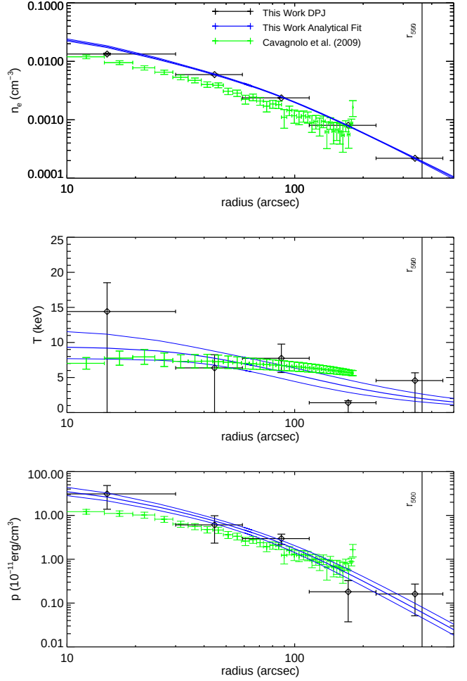
Figure A5. Abell 963. We detect a decrease in the temperature profile at large radius at a significance of 6\sigma . Our temperature profile is in good agreement with the ACCEPT results, although our density profile is somewhat higher. We do not detect the presence of a cool-core, but others have found a slight temperature decrease in the center ( Baldi et al. 2007 ; Cavagnolo et al. 2009 ). Leccardi & Molendi (2008) , using XMM-Newton , specifically made note of this and identified it as an 'intermediate' cluster since the temperature decrease in the center is modest.
