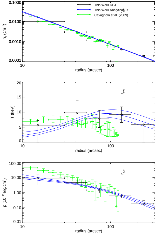
Figure A36. MACS J1423.8+2404. Our profile fit detects a cool core at a significance of 3.3\sigma , and both our density and temperature profiles are consistent with those from the ACCEPT analysis. Adam et al. (2016) conducted a multi-wavelength analysis of the cluster, including X-ray surface brightness and spectroscopy and high resolution SZ data to jointly constrain smooth ICM profiles that are in good agreement with our results. Kotov & Vikhlinin (2006) used Chandra X-ray spectroscopy to constrain the temperature profile, which is again consistent with our results. Morandi et al. (2010) used Chandra data, and found a cool-core (3 keV core and 7 keV peak at 300 kpc), again in good agreement with our fits. Based on lensing measurements, this cluster has been found to be slightly elongated and relaxed, with little substructure (Limousin et al. 2010; Zitrin et al. 2011).
