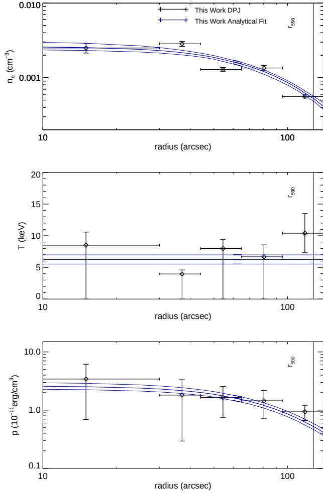
Figure A44. CL J0152.7. The irregular shape of our deprojected density profile is possibly due to the disturbed nature of the cluster. Several studies found evidence of subclusters and of merging based on: X-ray and optical subclusters (Huo et al. 2004), a high velocity dispersion of galaxy cluster members (Girardi et al. 2005), and an offset between the X-ray and SZ emission peaks (Massardi et al. 2010). Maughan et al. (2006) used XMM-Newton to study the X-ray emission distribution in detail, finding many substructures and smaller groups, concluding that the cluster has recently undergone many mergers.
