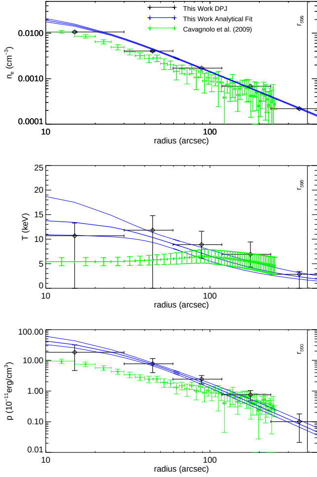
Figure A4. Abell 1423. We detect a decrease in the temperature profile at large radius at a significance of 6.9\sigma . AMI Consortium et al. (2012) , using SZ data rather than X-ray spectroscopic measurements, fit an isothermal model with a temperature of 3.0 \pm 0.8 keV, somewhat low compared to our measurements. However, the X-ray spectroscopic measurements from ACCEPT indicate a higher temperature (5.2 keV), which is in better agreement with our results, at least outside of the core region.
