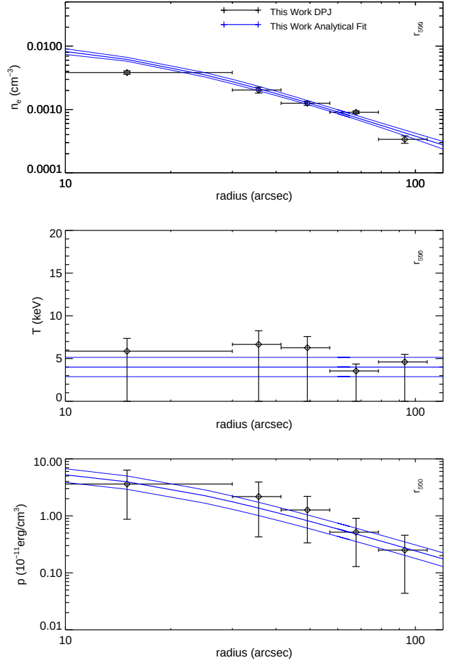
Figure A39. MS 2053.7-0449. This is the least massive cluster in our sample, with M_{500} \approx 3 \times 10^{14} M_{\odot} , and one of the dimmest clusters in the SZ. The low mass and high redshift also produce a weak X-ray signal. This makes it one of the few clusters in our analysis where the constraints do not extend to r_{500} . Verdugo et al. (2007) found a bimodal and elongated mass distribution for this cluster using Hubble data, indicating a merger.
