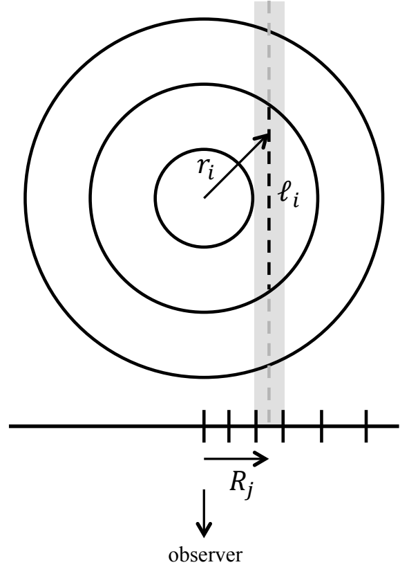
Figure 3. The concentric shell model, adapted from McLaughlin (1999). The observer sees a 2-D map with radial bins denoted by R_j , while the 3-D shells have radii r_i . The radial coordinates for the 2-D bins do not necessarily match those for the 3-D shells. l_i is the distance along the line of sight that radial shell i contributes to the 1D bin at radius R_j .
