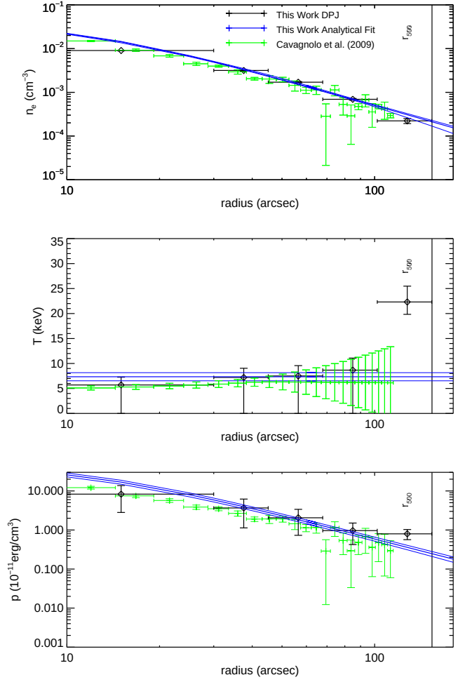
Figure A29. MACS J1311.0-0310. Our results for this cluster are in excellent agreement with the ACCEPT results.
