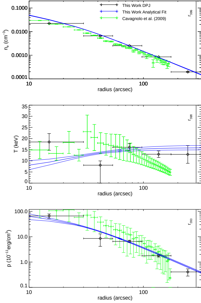
Figure A28. MACS J1347.5-1144. We detect a cool-coor in our smooth parametric fit at a significance of 3.1\sigma , but we do not find strong evidence for a temperature drop in the outskirts. Compared to the ACCEPT results, our temperature is somewhat higher at large radius. Donahue et al. (2014) obtained temperature profiles with a central temperature of 5 keV, with a peak of 17 keV that decreases in the outskirts, in good agreement with the ACCEPT results. Maughan et al. (2008) used Chandra imaging and spectra and assumed isothermal profiles, finding 12.2 keV for r < r_{500} , and 11.7 keV for 0.15 < r < 1r_{500} , roughly consistent with our profiles. Lu et al. (2010) studied this cluster using the optical waveband, and found a possible filament between a cluster 7 Mpc away. This cluster has many SZ-focused studies devoted to it. Ferrari et al. (2011) compared radio GMRT data with MUSTANG, Chandra , and XMM-Newton X-ray data, and found a correlation between the intracluster radio emission and X-ray and SZ emission. Korngut et al. (2011) made a high resolution SZ map using MUSTANG, and was able to find substructure 20'' from the center in the form of gas that has been heated through shocks caused by mergers. Ferrari et al. (2011) combined X-ray and SZ data to study the cluster, finding substructure near the core and very hot gas in the cluster up to 20 keV without the use of X-ray spectroscopy. Komatsu et al. (2001) mapped the SZ signal at 150 GHz with 13'' resolution using the Nobeyama telescope, and detected the excess SZ emission at 20'' . Pointecouteau et al. (2001) on the other hand, made a similarly resolved map, and could not constrain substructure, although they did observe that the signal was not completely spherical. Most recently, Sayers et al. (2016) was able to place an upper limit on the amplitude of the peculiar velocity of the cluster using 5-band SZ measurements.
