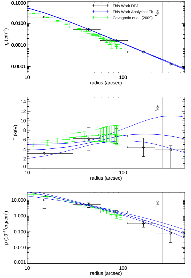
Figure A19. MACS J1532.9+3021. Our results for this cluster are in good agreement with the ACCEPT results. Donahue et al. (2014) obtained temperature profiles from X-ray spectroscopy ( XMM-Newton and Chandra ) with the temperature profile showing a central value of 3-4 keV before rising to 8 keV at larger radii, consistent with our analysis. The XMM-Newton profile decreased down to ~4keV at 900 kpc (~180''), while the Chandra profile does not show the temperature decrease, instead plateauing at ~9 keV. Hlavacek-Larrondo et al. (2013) performed a Chandra , XMM-Newton , VLA, and Hubble analysis. They observed evidence of AGN feedback, a cold front, and X-ray cavities. They note a difference in the temperature map from the east and the west side of the cluster, and find a central temperature of 4 keV rising to 9 keV at 250 kpc (~50''). They also detect slight differences in the temperature profile at small radii (<25'') in different directions, with higher temperatures in the S and W directions.
