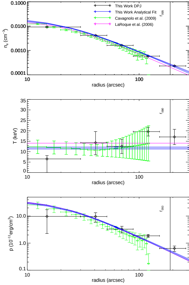
Figure A40. MACS J0647.7+7015. Our results for this cluster are in good agreement with the ACCEPT fits. Although our smooth parametric density profile shows a statistically significant offset from the LaRoque et al. (2006) results, the absolute magnitude of the offset is modest.
