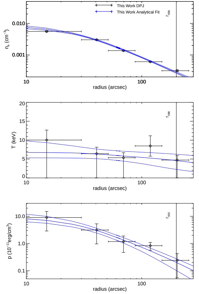
Figure A31. MACS J0911.2+1746. Kartaltepe et al. (2008), using optical data, found this cluster consists of two subclusters with different masses separated by 1 Mpc. The X-ray centroid was found to be significantly offset from the galaxy surface density for the smaller subcluster, suggesting that this system has undergone a recent merger.
