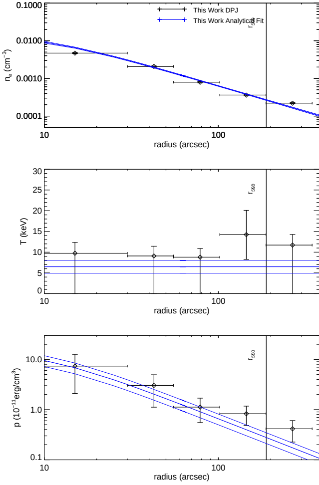
Figure A18. ZWCL 0024+17. Zhang et al. (2005) performed an XMM-Newton study using imaging and spectroscopy, and found a temperature decrease at large radii (80''–180'') from the isothermal ~4keV central region, which is fairly consistent with our results. They also found an elongation in the X-ray hard ratio map on large scales, and substructure at large radii. Ota et al. (2004) used Chandra spectroscopy and found a nearly isothermal profile of ~4.5 keV out to 600 kpc (110''), again quite similar to our results. Böhringer et al. (2000) used ROSAT to look at the cluster's X-ray morphology, and found a very small core radius in the surface brightness. They also found an elongation in the X-ray emission, however it is consistent with a spherical model. Tyson et al. (1998) obtained a mass map using strong lensing measurements, and found a relaxed distribution. Umetsu et al. (2010) performed a full-lensing analysis, including Subaru and Hubble /ACS/NIC3 observations, and looked at X-ray data along with simulations. They suggest that the cluster is in a post-collisional state, with two clusters at the same line of sight, as well as finding the mass profile of the cluster. Jee et al. (2007) noted that the X-ray surface brightness from Chandra is better fit by two isothermal beta models, suggesting that possibly one could be seeing two systems that are along the same line of sight.
