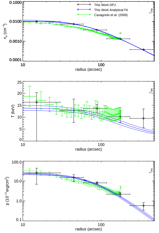
Figure A7. Abell 2219. Our smooth parametric fit shows a decrease in temperature in the outskirts at a significance of 11.8\sigma , and both our density and temperature profiles are in excellent agreement with the ACCEPT values. Jiménez-Bailón et al. (2013) found a shock front with >16 keV gas 2' NW of cluster, and this elongated cluster is possibly undergoing a large merger event (Boschin et al. 2004). Further evidence for a major merger was detailed in Canning et al. (2015), who used Chandra data to identify numerous cold and shock fronts, along with a large temperature spike \sim 25'' away from the core of the cluster.
