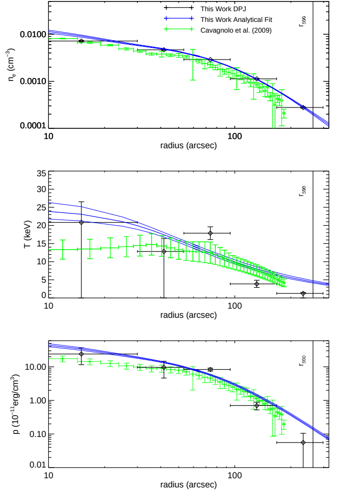
Figure A35. MACS J0717.5+3745. Our profiles for this cluster are in excellent agreement with the profiles obtained in the ACCEPT analysis, and our smooth parametric fit indicates a temperature drop at large radius at a significance of 24\sigma . This cluster has been studied extensively in different wavelengths. Ma et al. (2009) found that the cluster consists of four large subclusters based on X-ray imaging and galaxy positions. Through lensing ( Medezinski et al. 2013 ; Diego et al. 2015 ; Limousin et al. 2016 ; Umetsu et al. 2016 ), four large masses are also clearly found, reflecting that this cluster is a complex merger. Mroczkowski et al. (2012) studied this cluster through the SZ effect, X-ray and lensing observations. They also found very hot gas near 30 keV in some regions of the cluster. A large kSZ signal in one of the subclusters, which has not been accounted for in our analysis, could potentially be a source of bias in our results ( Sayers et al. 2013c ).
