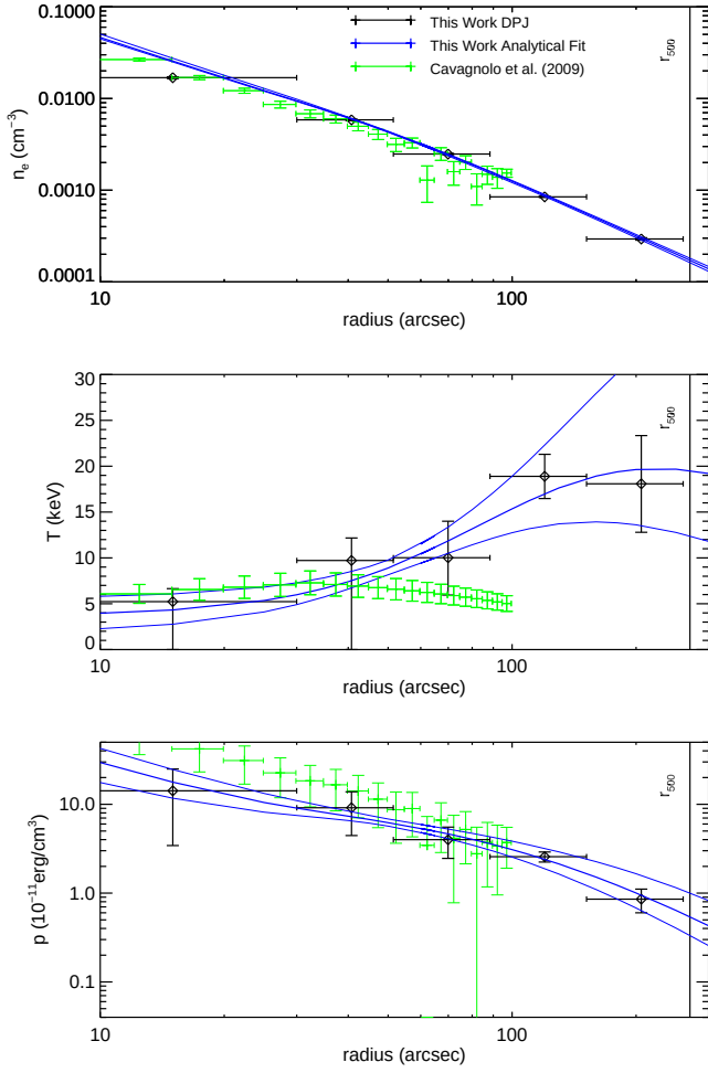
Figure A14. MACSJ1931.8-2634. At overlapping radii, our results are fairly consistent with the ACCEPT results, except for a slight increase in our derived temperatures towards large radius. Based on our smooth parametric fits, there is some evidence for a drop in temperature at the cluster center ( \sim 2\sigma ). A detailed multi-wavelength study of this cluster was performed by Ehlert et al. (2011) using X-ray ( Chandra ), optical (Subaru), and radio (Very Large Array) data. They found a cool core with AGN feedback (seen in the X-ray and in the radio), along with evidence of merging, suggesting a cool core that is currently being destroyed. They created a temperature map of the cluster from X-ray spectroscopy out to radii of 500 kpc (100"), and found an asymmetric temperature distribution. Their azimuthally averaged temperature profile has a central temperature of 5 keV and peak of 10 keV, roughly consistent with our results.
