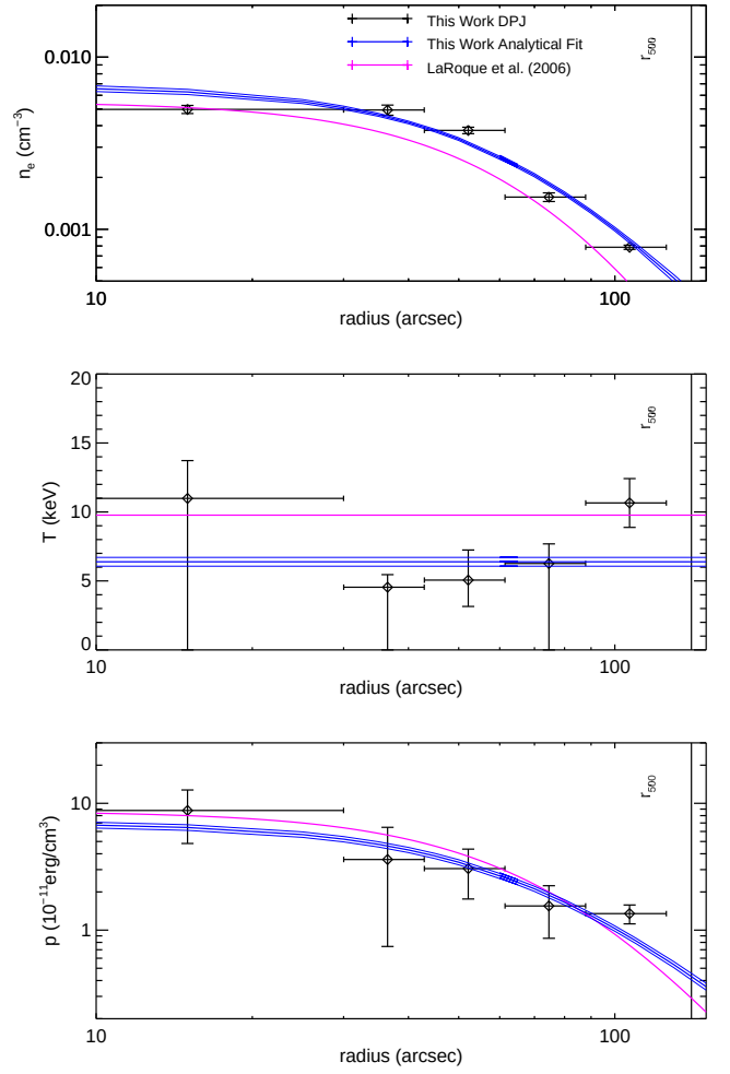
Figure A43. MS1054.4-0321. Compared to the smooth parametric fits of LaRoque et al. (2006) , our smooth parametric fits show a significant offset in both density and temperature. Gioia et al. (2004) used XMM-Newton to find an average temperature of \sim 7\text{keV} , in good agreement with our results. Neumann & Arnaud (2000) studied this cluster using the X-ray ( ROSAT ), finding substructure and other signs of recent merging processes (e.g., BCG and X-ray peak offset, X-ray centroid and peak offset).
