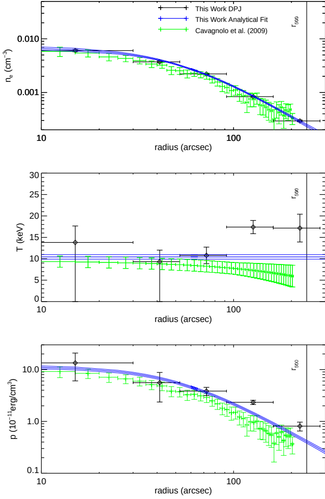
Figure A34. MACS J1149.5+2223. Our results for this cluster are in general agreement with the ACCEPT results, although our deprojection indicates a somewhat higher temperature at large radius. This massive cluster has been widely studied through gravitational lensing. Using Hubble data, Mohammed et al. (2016) constrained the mass distribution of this cluster and found several main peaks and clear non-sphericity, suggesting this is a merging cluster.
