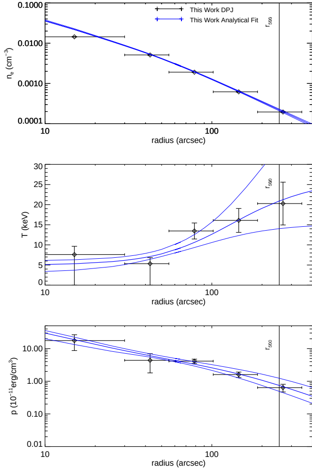
Figure A16. MACS J1115.8+0129. The ACCEPT analysis finds densities systematically lower than ours, but our results are consistent with other studies (e.g., Mantz et al. 2016 ), and so the ACCEPT profiles are not plotted. Donahue et al. (2014) found temperature profiles from X-ray spectroscopy ( XMM-Newton and Chandra ), showing a central temperature of around 3 keV rising to 8–9 keV, roughly matching our results over the same region. However, the XMM-Newton data then show a decrease in the temperature profile near 800 kpc (160''), which is not seen in our results.
