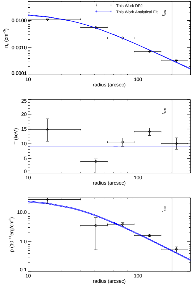
Figure A37. MACS J0454.1-0300. The densities from the ACCEPT analysis are systematically lower than ours. However, the ACCEPT results are also inconsistent with two other analyses (Bonamente et al. 2006; Amodeo et al. 2016), and so the ACCEPT profiles are not plotted. Donahue et al. (2003) used Chandra X-ray spectroscopy to obtain an isothermal temperature of 10.2 keV, consistent with our results. They also found an elliptical cluster morphology, and a shift in the BCG location and X-ray centroid.
