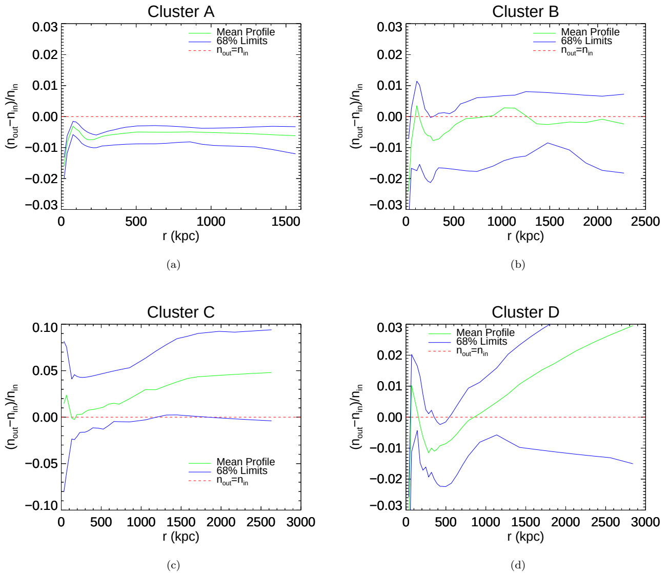
Figure 5. Normalized difference between the input deprojected density profile used to generate the test clusters and the fitted deprojected density profile recovered from the mock observations. Note the y-axis scale is larger for Cluster C than for the others. The green line represents the mean fitted profile, while the blue limits represent the upper and lower 68% limits for the fitted density at that particular radius.
