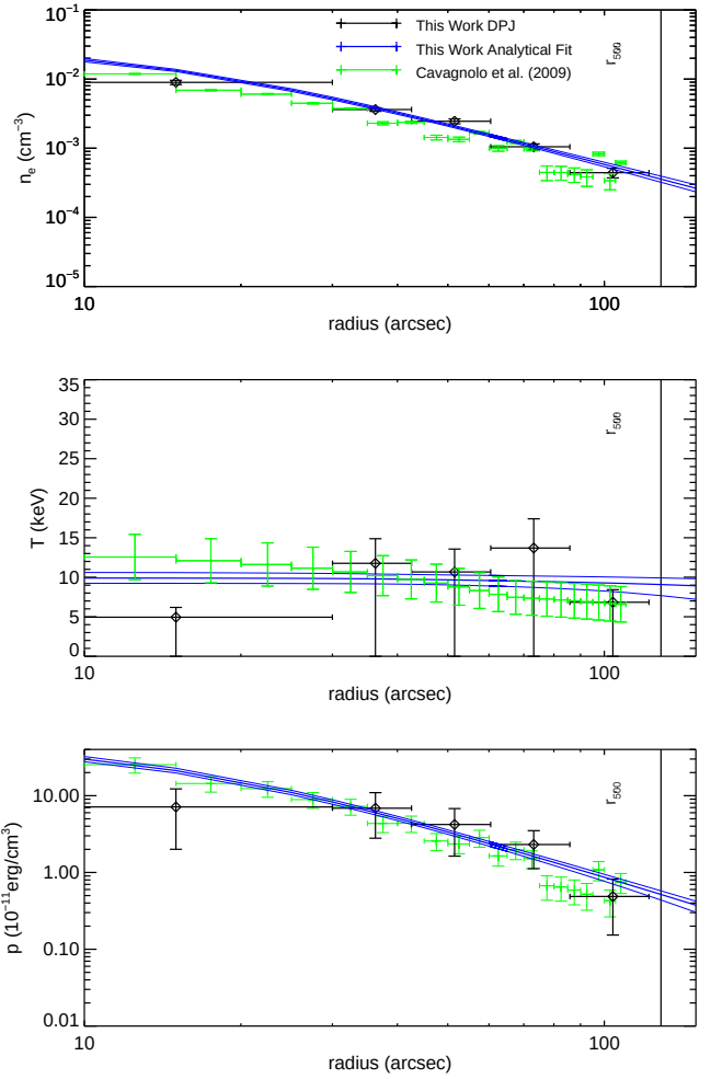
Figure A45. CL J1226.9+3332. Our results for this cluster are in relatively good agreement with the ACCEPT fits. Although this cluster is classified as non-disturbed in our analysis, several other works have found evidence of merging through X-ray temperature map asymmetries (Maughan et al. 2007), subclumps through weak lensing (Jee & Tyson 2009), and multiple peaks in the SZ through high resolution MUSTANG maps (Kornigut et al. 2011).
