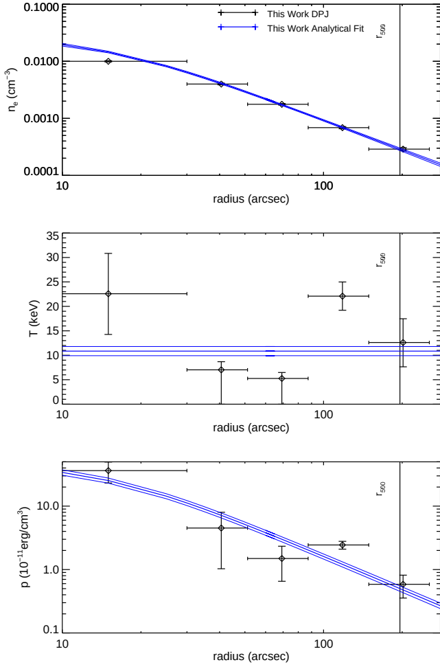
Figure A30. MACS J0257.1-2325. This cluster was part of the ACCEPT study, but the density profile is significantly low compared to our and other results (Amodeo et al. 2016), and so the ACCEPT profile is not plotted. Through the optical, Kartaltepe et al. (2008) found that, on large scales, this system has filaments directed into the cluster.
