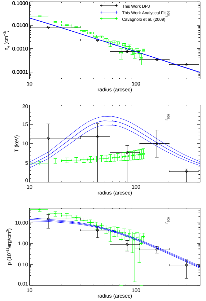
Figure A13. MS 2137. In our smooth parametric fits, we detect a temperature drop in the center at a significance of 5.3\sigma and a temperature drop in the outskirts at a significance of 11.3\sigma . Our fits are mostly consistent with the ACCEPT results, although our smooth parametric fit indicates a significantly higher temperature at intermediate radii. In reasonable agreement with the ACCEPT results, Donnarumma et al. (2009) obtained a spectroscopic temperature profile using Chandra with a 4 keV central temperature, a peak of 5.5 keV at 100 kpc (around 20''), and decreasing to 3.5 keV in the outskirts at 500 kpc (around 110'').
