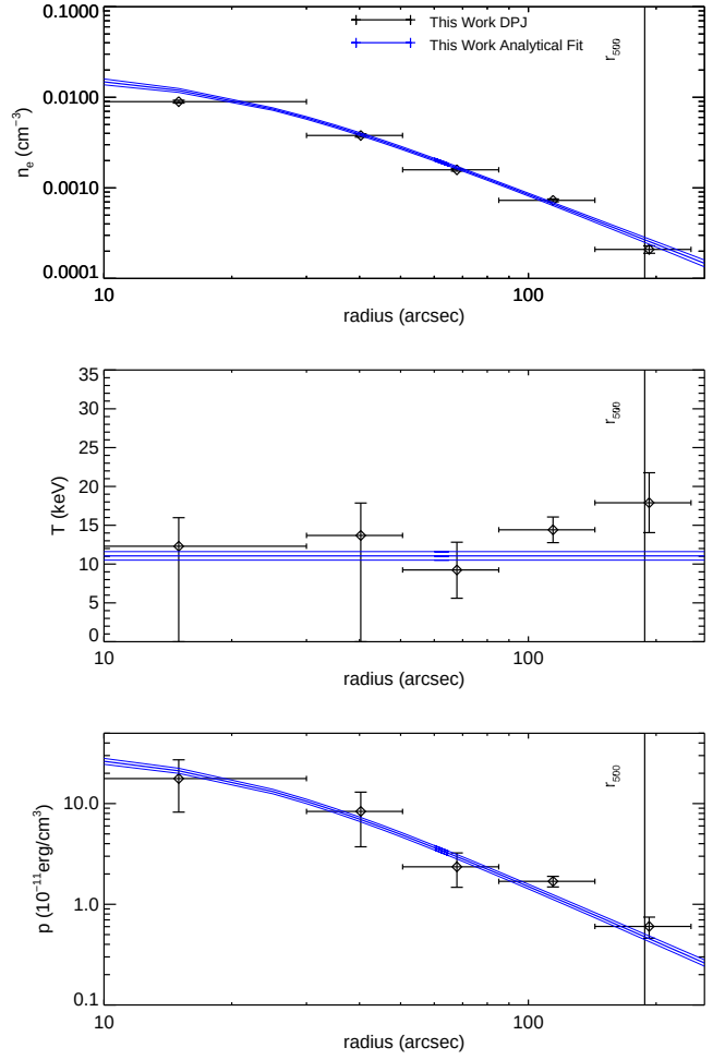
Figure A41. MACS J2129.4-0741. Mann & Ebeling (2012) conducted a classification of clusters based on morphology, using a combination of X-ray and optical data. For this cluster they deduced it was a merger because the X-ray centroid location is significantly different than the BCG's.
