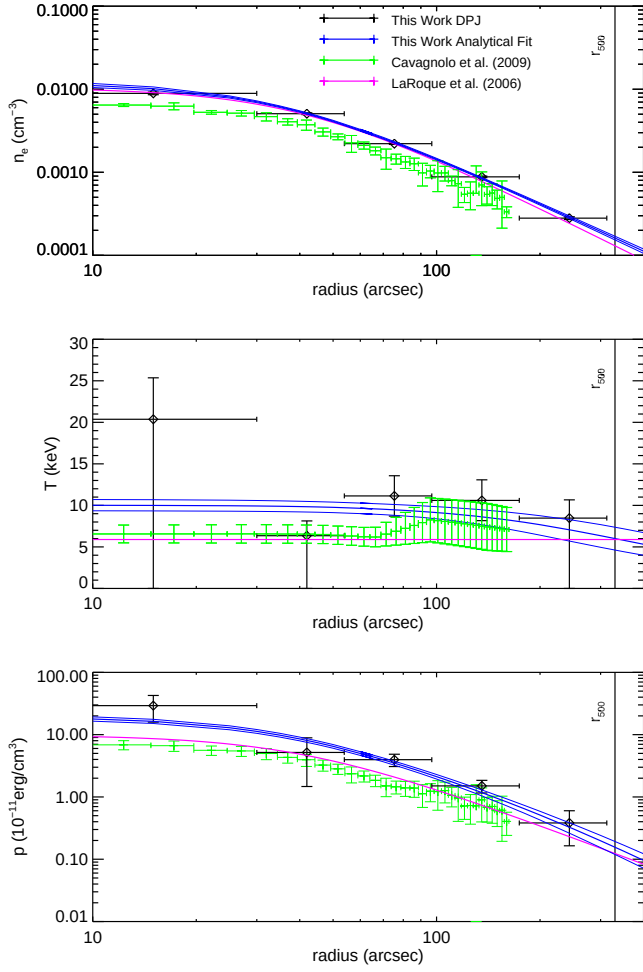
Figure A8. Abell 267. Our deprojections and smooth parametric fits show a mostly flat temperature profile. Overall, the temperature is consistent with ACCEPT’s relatively flat temperature profile, although our data indicate a somewhat higher temperature in the core region. Our smooth parametric fit shows some evidence for a drop in temperature at large radius ( 2.8\sigma ). Jiménez-Bailón et al. (2013) used XMM-Newton spectroscopy to deproject a temperature profile, and they also found an approximately flat profile with a temperature of \sim 6 keV. They consider A267 a ‘fossil’ system, which is dominated by a massive elliptical galaxy. Fossil systems in general have not merged recently, and usually host a cool-core. The lack of a cool core in this cluster is perhaps related to heating from an AGN.
