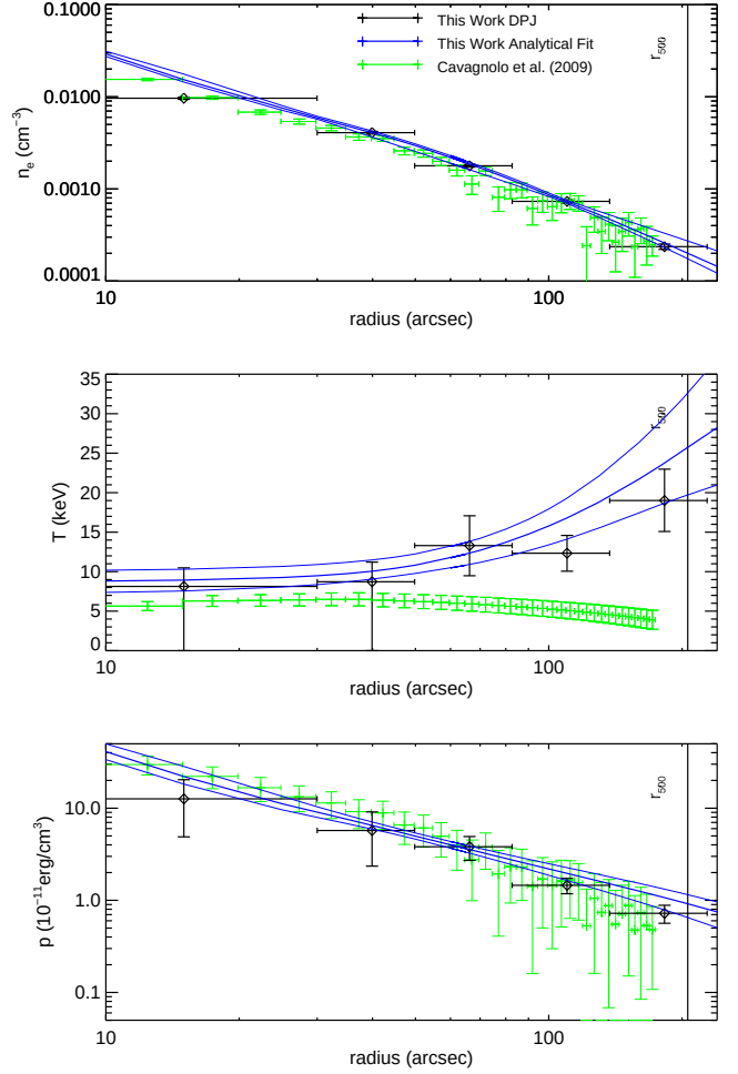
Figure A27. MACS J0329.6-0211. Our smooth parametric fit finds a temperature drop in the core at modest significance ( 2.1\sigma ). Compared to ACCEPT, our temperature profile is notably higher outside of the core region. Maughan et al. (2008) found a temperature of 4.5 keV for r < r_{500} , and 4.4 keV for radii within 0.15 < r < 1r_{500} , in good agreement with the ACCEPT results. Mann & Ebeling (2012) found this to be a relaxed cluster according to X-ray and optical alignment. Kotov & Vikhlinin (2006), using Chandra and XMM-Newton data, found this cluster to follow a standard cool-core temperature profile, except for a dip in temperature at intermediate radii (around 100 kpc), which could hint at some substructure. Giacintucci et al. (2014) found a possible radio minihalo centered in the cluster using VLA data, filling out much of the core to 150 kpc.
