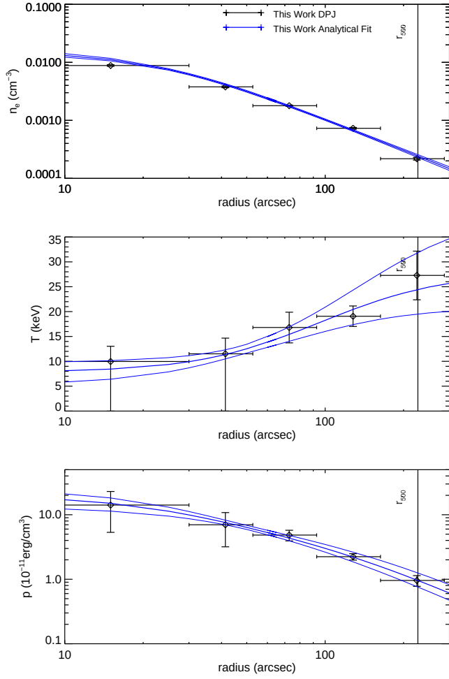
Figure A32. MACS J2214.9-1359. This cluster is part of the ACCEPT study, but the density profile is systematically lower than both ours and two other analyses (Bonamente et al. 2006; Amodeo et al. 2016), and so the ACCEPT profile is not plotted. Our smooth parametric fits indicate a temperature drop in the center at a significance of 2.2\sigma . Mann & Ebeling (2012) found this cluster to have the most relaxed morphological denotation, with a prominent cool core and perfect alignment between the X-ray peak and BCG.
