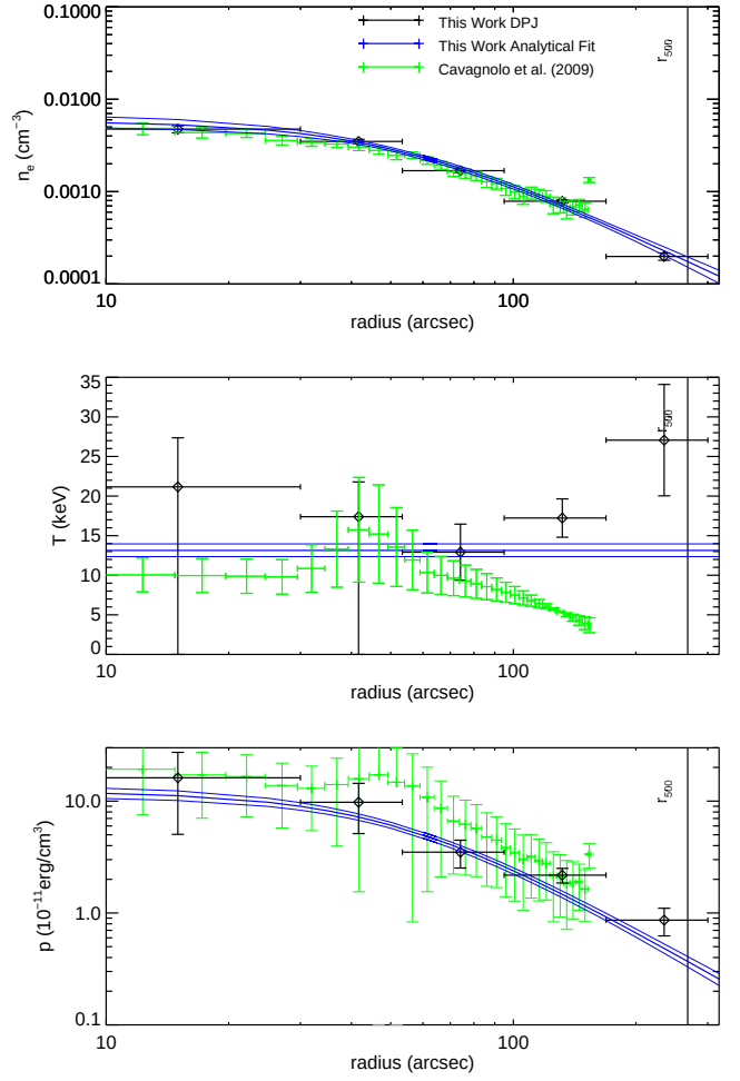
Figure A17. Abell 370. Our results for this cluster are fairly consistent with the ACCEPT results, although they do not show a temperature drop at large radius. Several studies at different wavelengths have found that this cluster is not spherical. This is a very popular lensing cluster, and many such studies have been performed ( Medezinski et al. 2010 ). De Filippis et al. (2005) combined X-ray and SZ data to find the 3d shapes of galaxy clusters, including Abell 370, and found a triaxial morphology, elongated along the line of sight. Richard et al. (2010) conducted a strong lensing analysis based on Hubble /ACS observations and reconstructed the mass distribution, which indicates an elongated, bimodal, mass distribution aligned with the Chandra X-ray luminosity maps. The galaxy distribution also shows bimodality, suggesting a merging cluster. Grego et al. (2000) , using OVRO SZ observations of this cluster, also found a smooth but non-spherical distribution.
