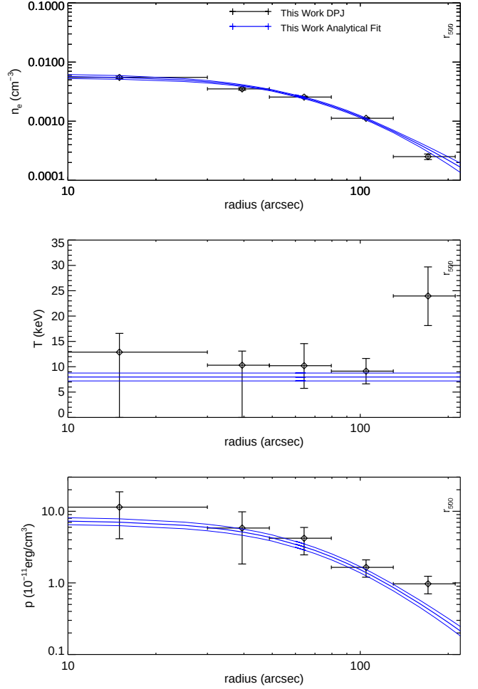
Figure A23. MACS J0416.1-2403. Several studies have identified this cluster as a binary merger system. Mann & Ebeling (2012), using optical and X-ray data, found this system to contain a possible binary head-on collision, just after the first collision. Jauzac et al. (2015) conducted a joint X-ray and optical study, and unveiled a large structure associated with a line-of-sight filament that could not be seen in the X-ray. A large offset in the radial velocity between two subclusters was found, and their temperatures were determined to be 10 and 13.6 keV, slightly higher than our isothermal smooth parametric fit. Ogrea et al. (2015) created temperature, pressure, and entropy maps using a multi-wavelength analysis of Chandra , the VLA, the GMRT, and Hubble . The temperature map is elongated, and has a relatively high mean temperature of 10 keV. The radio halo is also elongated along the same direction.
