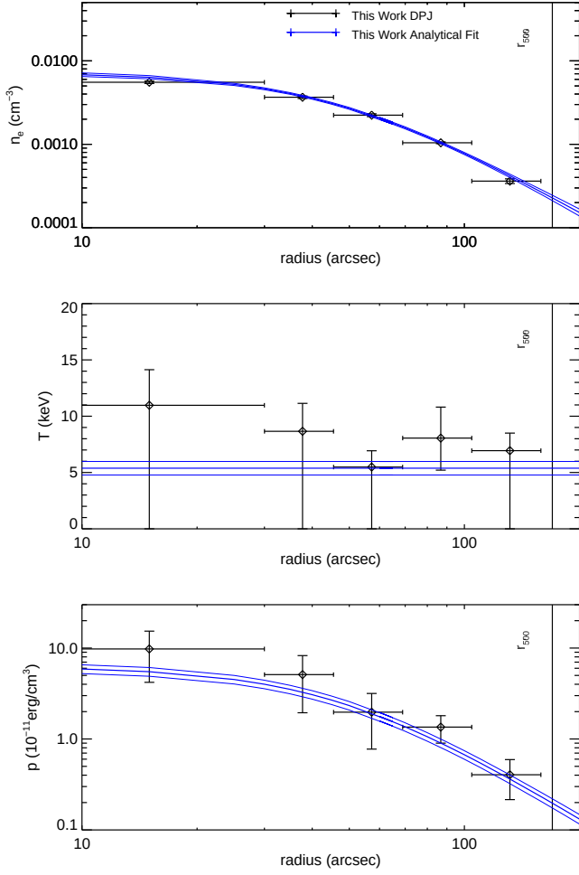
Figure A38. MACS J0025.4-1222. Although this cluster is classified as non-disturbed in our analysis, two other studies find that it is clearly a major merger between two clusters of similar masses (Bradač et al. 2008; Kartaltepe et al. 2008). Furthermore, Bradač et al. (2008) found that the cluster total mass distribution is not consistent with the gas distribution.
