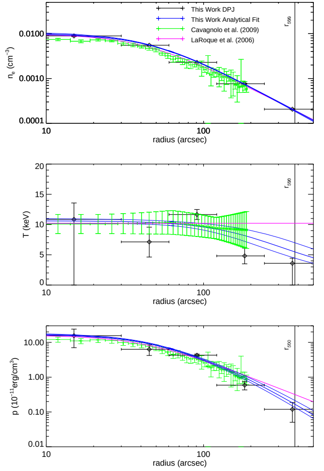
Figure A11. Abell 697. We find a relatively flat inner temperature profile, and we detect a drop in temperature near r_{500} at a significance of 4.5\sigma . Our Pressure profiles are consistent with the joint X-ray/SZ study of LaRoque et al. (2006), and there is good agreement between our density, temperature, and pressure profiles and the corresponding ACCEPT profiles. Although we characterized the cluster as non-disturbed, several other studies have shown that the cluster has undergone recent merging. Giardi et al. (2006) conducted a multi wavelength study using optical and X-ray data, where line of sight galaxy velocity dispersions and spectroscopic temperatures were calculated, respectively, and found that A697 is not relaxed. With elongated X-ray emission and substructures near the center, Abell 697 likely went through many mergers. Through lensing, Metzger & Ma (2000) also concluded that the cluster has undergone a recent merger.
