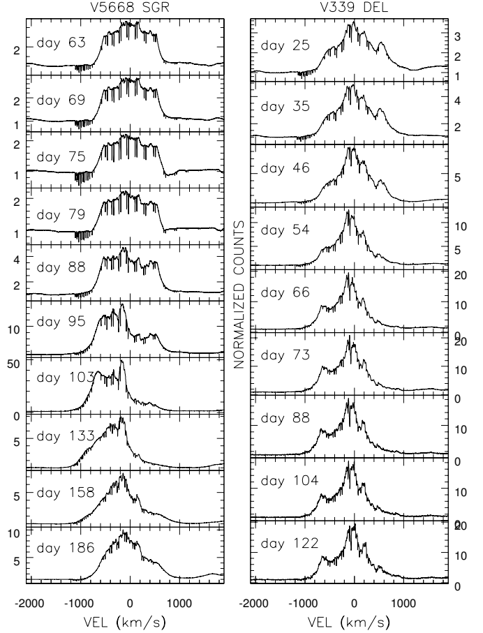
Fig. 5. Comparison of the time development of [O I] 6300 Å for V5668 Sgr (left column) and V339 Del (right column). An intrinsically optically thin transition, this forbidden line traces the effect of the dust formation event. See text for details
