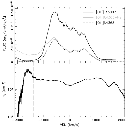
Fig. 7. Electron density distribution in the V5668 Sgr ejecta for day 186 based on the optical [O III] profiles. The 4363 Å is plotted without removing the H \gamma contribution for visualization purposes. The H \beta line was used to model H \gamma , see text for discussion. Notice that, like the nitrogen ratios, the derived n_e is the same for the two lobes of the ejecta despite the profile asymmetries.
