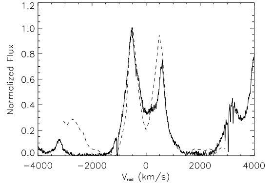
Fig. 8. Comparison of the [Si VI] 1.96 \mu profile from day 350 (dash) with He II 1640 Å from the STIS spectrum (solid). This highlights the difference in the extinction between the infrared and UV. See text for details.
