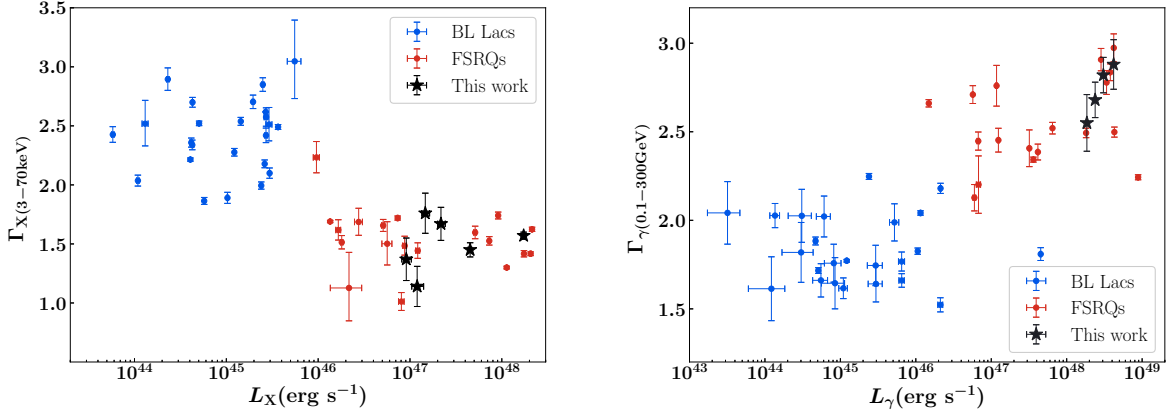
Figure 7. Left panel: NuSTAR luminosity versus X-ray spectral index for all BL Lacs and FSRQs listed in the 3LAC detected by NuSTAR (Marcotulli et al., in preparation). Our sources fall in the lower right corner of the graph, having high X-luminosities and hard \Gamma_X , therefore in agreement with the most powerful blazars. Right Panel: Fermi -LAT luminosity versus \gamma -ray spectral index for the same sources. As can be seen, our high-redshift blazars belong to the most powerful FSRQs, with high \gamma -luminosities and very soft \Gamma_\gamma .
