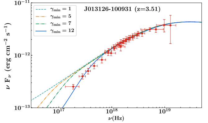
Figure 6. Zoomed SED of J013126–100931, showing the X-ray spectrum. The different lines represent the modeling done with various \gamma_{\min} values (as labeled). As can be seen, good X-ray coverage allows us to constrain the value of \gamma_{\min} which, due to the break in the soft X-ray spectrum, is found to be \sim 12 .
