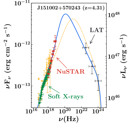
Figure 4. Zoomed high-energy SED of J151002+570243. The yellow/orange data points are the archival observations and the yellow/orange line is the SED model derived by Ackermann et al. 2017. The blue line is the best fit model we obtained using combined soft X-ray (green), hard X-ray (red) and \gamma -ray (black) data.
