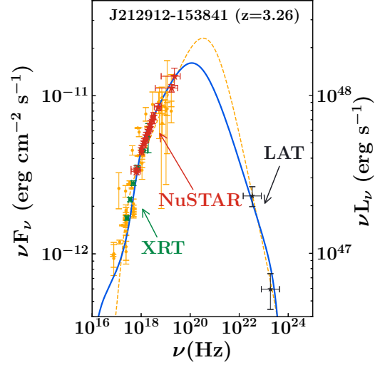
Figure 5. Zoomed high-energy SED of J212912-153841. The yellow/orange data points are the archival observations and the yellow/orange line is the SED model derived by Ackermann et al. 2017. The blue line is the best fit model we obtained using combined soft X-ray (green), hard X-ray (red) and \gamma -ray (black) data.
