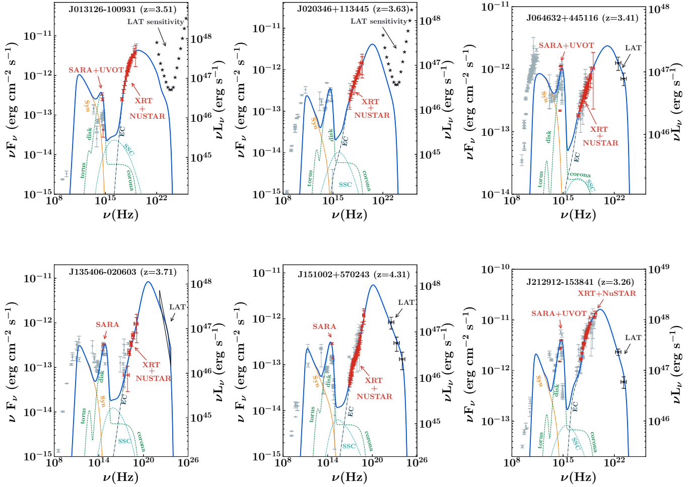
Figure 2. The broadband SED of six quasars using quasi-simultaneous SARA, Swift , NuSTAR , and Fermi -LAT data, modeled via the one zone leptonic emission model described in the text. Grey circles represent the archival data, the black stars are the Fermi data extracted from Ackermann et al. 2017, while the red points show our quasi-simultaneous observations. Since the LAT SED data points for J135406-020603 are not published in Ackermann et al. 2017, we use the parameters listed in their paper to extract the bowtie plot showed here. The lines are the modeling lines illustrating different components considered: the orange line is the synchrotron emission; the green dotted line includes the thermal emission from the torus, the disk and the corona; the light-blue dotted line represents the SSC component; the dark blue dotted line is the EC component. The blue solid line is the sum of all the other contributors and delineate our best fit model (see Section 4 for detailed discussion). For the optical data, when available, we plot the photometric data below the redshifted Ly- \alpha frequency since above this limit the emission is significantly affected by absorption from intergalactic hydrogen (e.g. Songaila & Cowie 2010; Croft et al. 2018).
