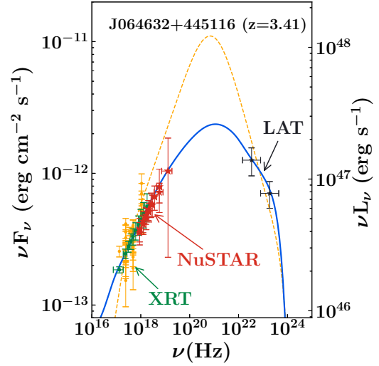
Figure 3. Zoomed high-energy SED of J064632+445116. The yellow/orange data points are the archival observations and the yellow/orange line is the SED model derived by Ackermann et al. 2017. The blue line is the best fit model we obtained using combined soft X-ray (green), hard X-ray (red) and \gamma -ray (black) data. We emphasize that the availability of NuSTAR observations allow us to tightly constrain the rising part of the EC peak, enabling us to accurately infer the power of the jet and the underlying particle distribution shape (see Table 6).
