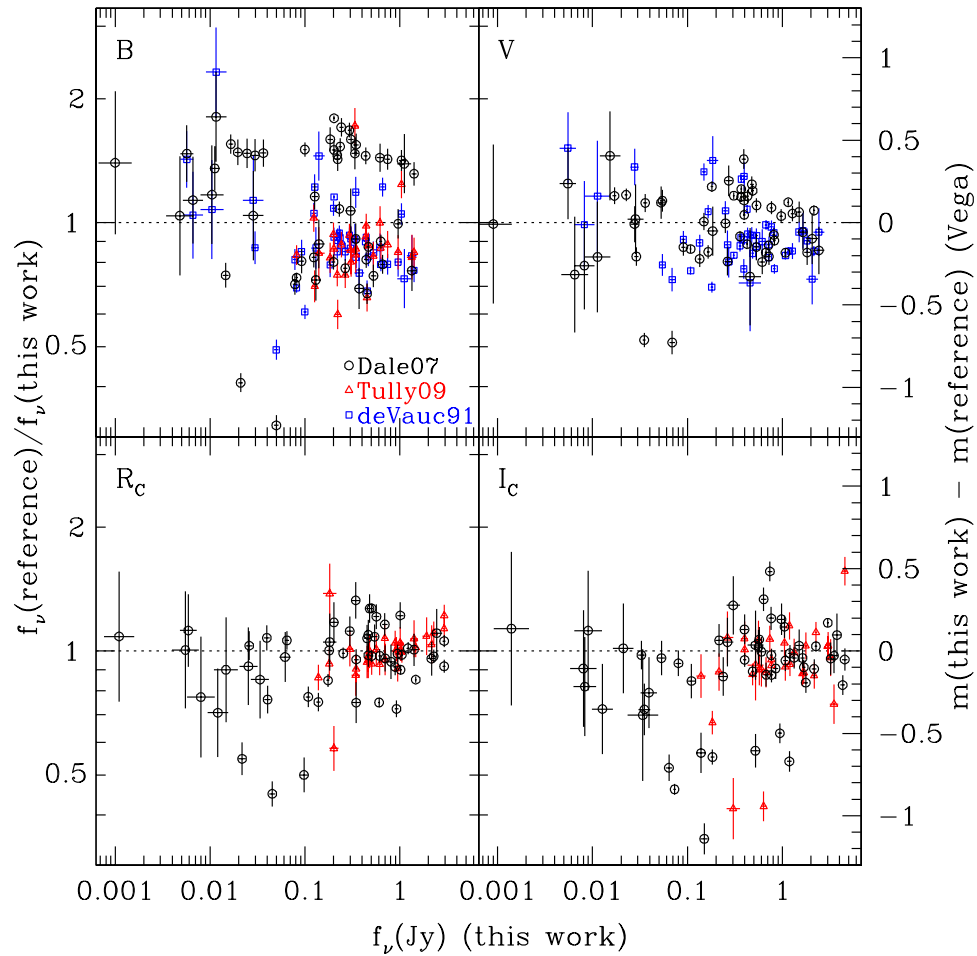
Figure 2. Comparison of global BVR_C I_C galaxy photometry from the literature with those measured here that are calibrated based on Pan-STARRS1 g_{p1}r_{p1}i_{p1}z_{p1} photometry on field stars (see Section 3.1).
