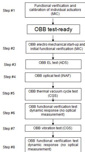
Figure 7. Sequence of the laboratory test campaign.
