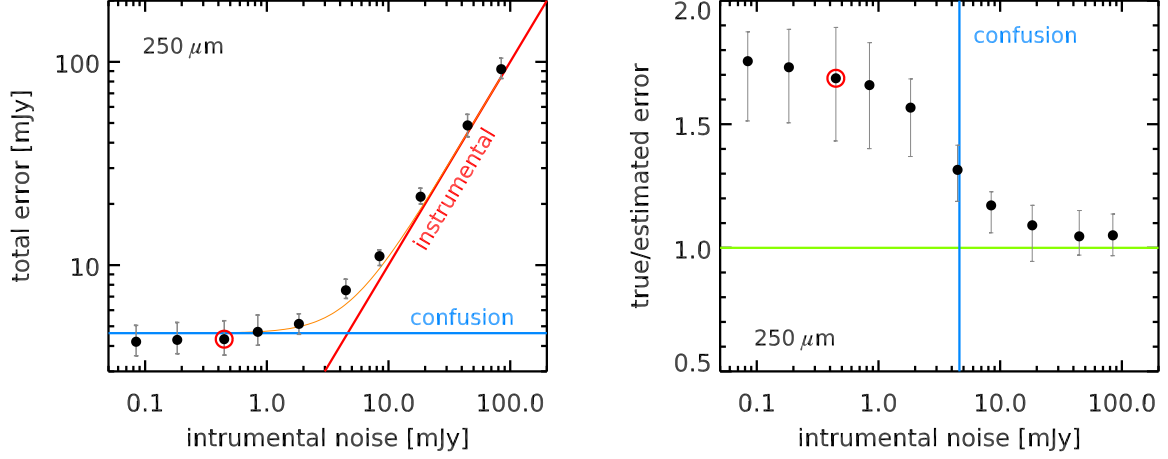
Fig. B.4. True error \sigma on the stacked flux measurements as a function of the instrumental white noise level \sigma_{\text{inst.}} that is put on the image (here normalized to a “PSF” noise in mJy, i.e., the error on the flux measurement of a point source in the absence of confusion). We generated multiple simulations of the 250\,\mu\text{m} maps using varying levels of white noise, and compute \sigma from the difference between the measured fluxes and their expected values. Left: evolution of the average total noise per source \sigma_{\text{tot.}} = \sigma \times \sqrt{N_{\text{stack}}} where N_{\text{stack}} is the number of stacked sources. This is the total error when extracting the flux of a single source on the map. When the instrumental noise (red line) is high, it dominates the error budget over the confusion noise. However, when reaching too low values, the measured total noise is dominated by the confusion noise \sigma_{\text{conf.}} (blue line). We fit this evolution as \sigma_{\text{tot.}}^2 = \sigma_{\text{inst.}}^2 + \sigma_{\text{conf.}}^2 (orange line) to obtain \sigma_{\text{conf.}} = 4.6\,\text{mJy} . The red circle marks the instrumental noise level reached in the real maps. Right: comparison between the estimated error from the stack residual \sigma_{\text{IMG}} and the true error \sigma . The points show the median of \sigma/\sigma_{\text{IMG}} , and the error bars are showing the 16th and 84th percentiles of the distribution. The green horizontal line is the line of perfect agreement, and the blue vertical line marks the confusion noise at 250\,\mu\text{m} . The red circle marks the instrumental noise level reached in the real maps.
