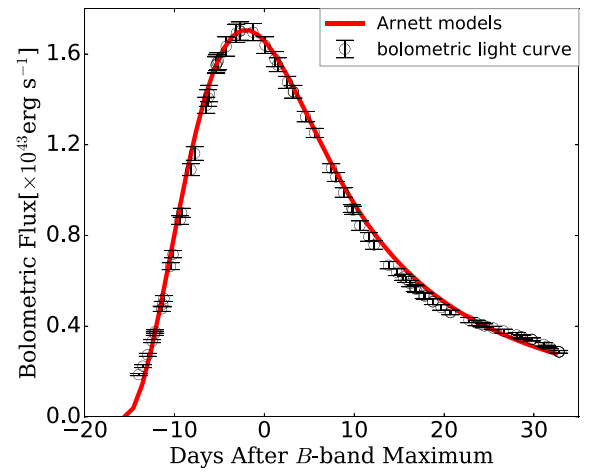
Figure 14. The quasi-bolometric light curve of SN 2019np (open black circles) compared to the best-fitting radiation diffusion model (red line; Arnett 1982).
