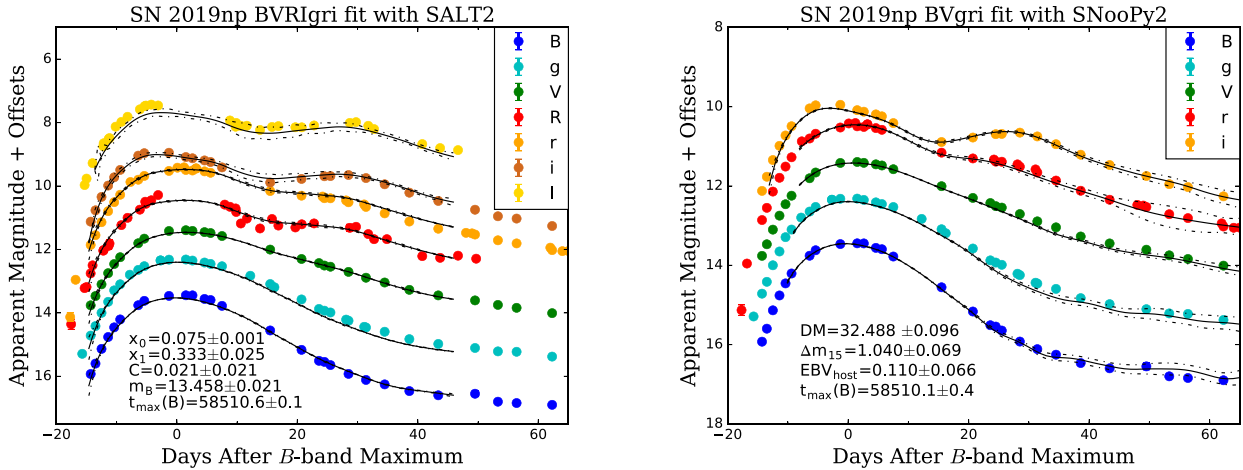
Figure 3. Best-fitting light-curve models from SALT2 (left-hand panel) and SNOOPy2 (right-hand panel). The light curves of different bands have been shifted vertically for better display. The dashed lines represent the 1- \sigma uncertainty of the light-curve templates. The parameter x_0 represents the normalization of the SED sequence, x_1 is the light curve shape parameter, and C stands for the colour. m_B and t_{\max}(B) denote the maximum magnitude of the B -band and the corresponding time. DM is the distance modulus.
